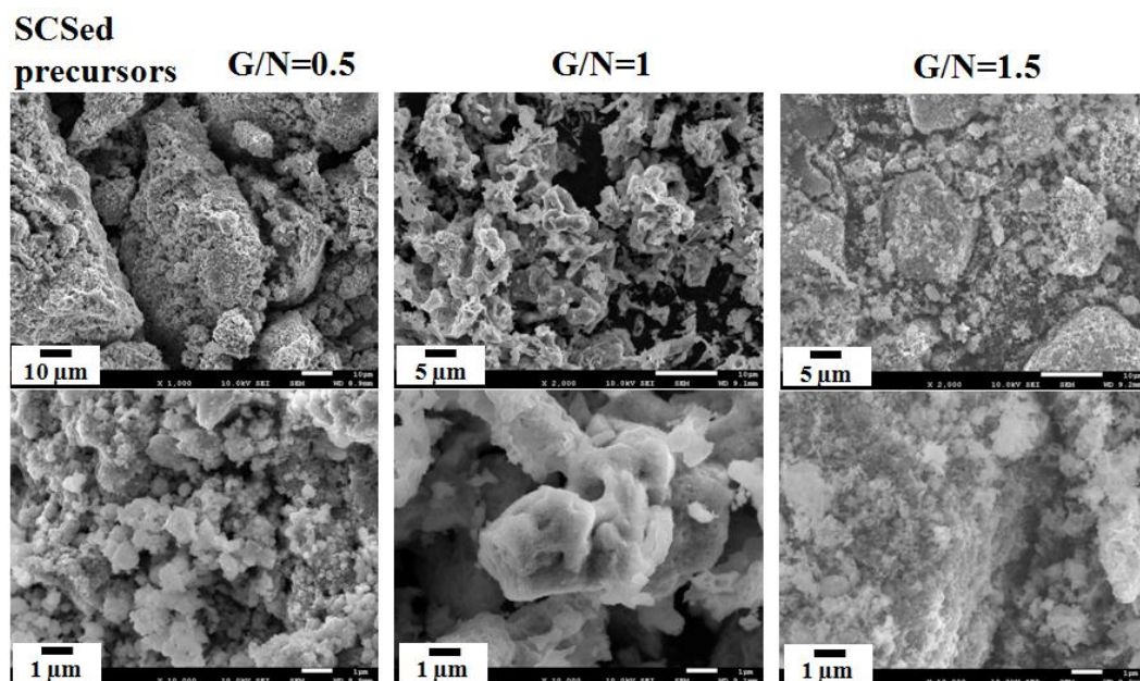
Figure 5. SEM images of the SCS-prepared precursors at different G/N ratios.
