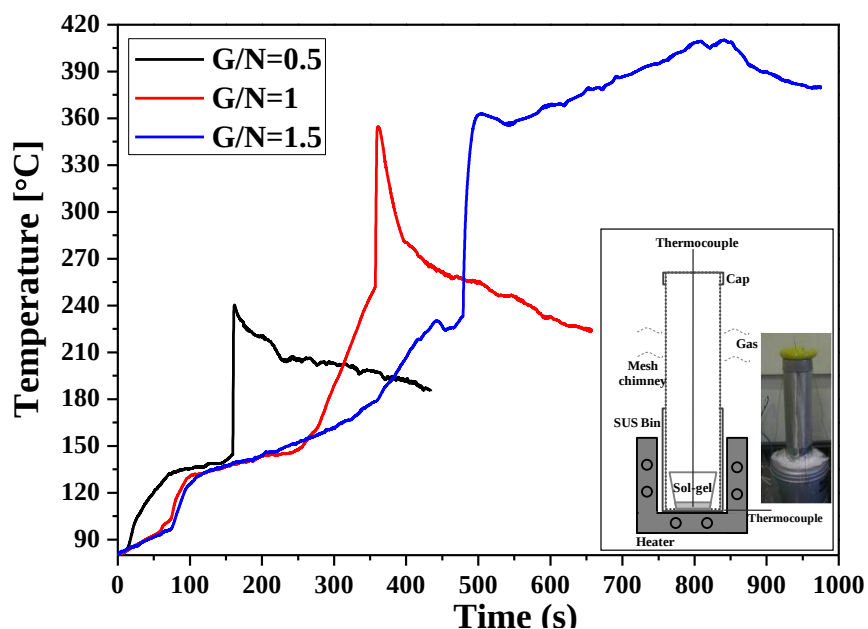
Figure 1. Temperature history of the combustion synthesis at different G/N ratios. 80 °C was assumed as zero point for the data-log. The inset shows an image of the apparatus used for the combustion synthesis.
