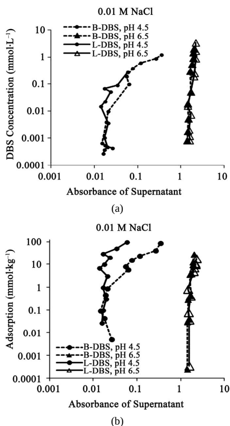
Figure 3. Relationships between absorbance of supernatant at 400 nm and (a) DBS concentration of supernatant; (b) Adsorption of DBS at 0.01 \text{ M} NaCl. The absorbance corresponds to relative concentration of dissolved humic substances. B-DBS indicates DBS with branched carbon chain and L-DBS with linear carbon chain.
