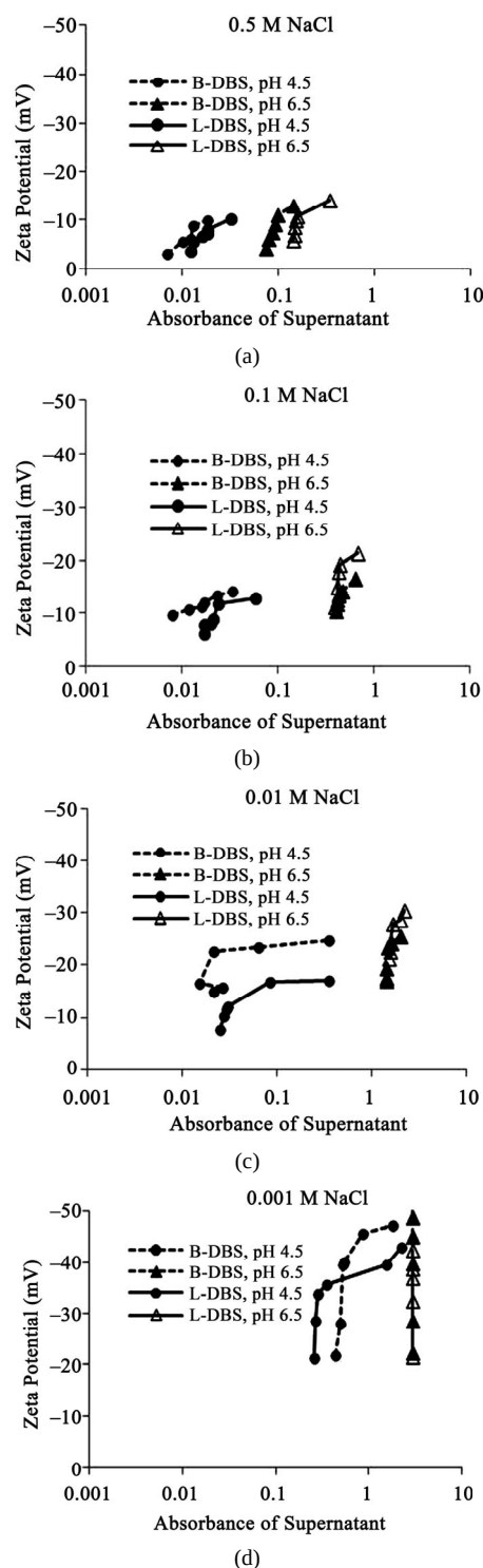
Figure 9. Relationships between absorbance of supernatant and zeta potential of the soil particles in suspension at electrolyte concentration of (a) 0.5 M NaCl and (b) 0.1 M NaCl, (c) 0.01 M NaCl and (d) 0.001 M NaCl for both branched and linear DBS at pH 4.5 and 6.5. The absorbance corresponds to the relative concentration of dissolved humic substances. B-DBS indicates DBS with branched carbon chain and L-DBS with linear carbon chain.
