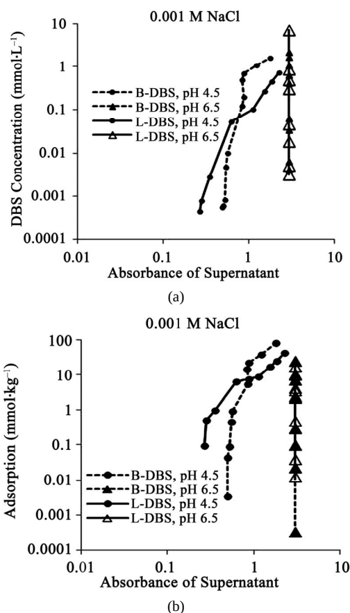
Figure 4. Relationships between absorbance of supernatant at 400 nm and (a) DBS concentration of supernatant; (b) Adsorption of DBS at 0.001 \text{ M} NaCl. The absorbance corresponds to relative concentration of dissolved humic substances. B-DBS indicates DBS with branched carbon chain and L-DBS with linear carbon chain.
