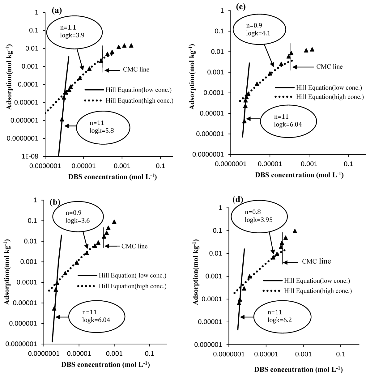
Fig. 4 Comparison of the calculated adsorption values using the Hill equation (3) and measured adsorption isotherm. (a) Branched DBS at pH 6.5, (b) branched DBS at pH 4.5, (c) linear DBS at pH 6.5 and (d) linear DBS at pH 4.5.
