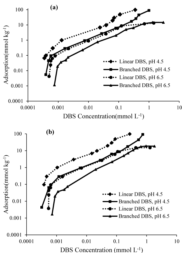
Fig. 5 Comparison between branched and linear DBS adsorption at pH 4.5 and 6.5 (a) after 3-hour and (b) 24-hour mixing.
