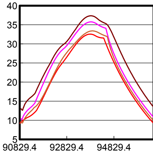
Figure 9. Comparison of temperature history at outer structure under worst hot case between two- and multi-nodal analyses.
