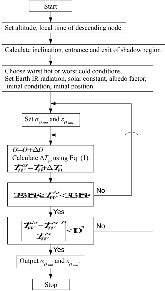
Figure 4. Flowchart of one-nodal analysis.
