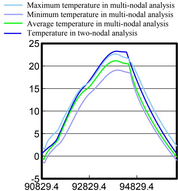
Figure 14. Comparison of temperature history at outer structure under worst cold case between two-nodal analysis with revised absorption at solar cells and multi-nodal analysis.
