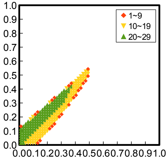
Figure 6. Combinations of \alpha_R and \epsilon_R when satellite temperature stays within design temperature range under worst hot and cold cases.
