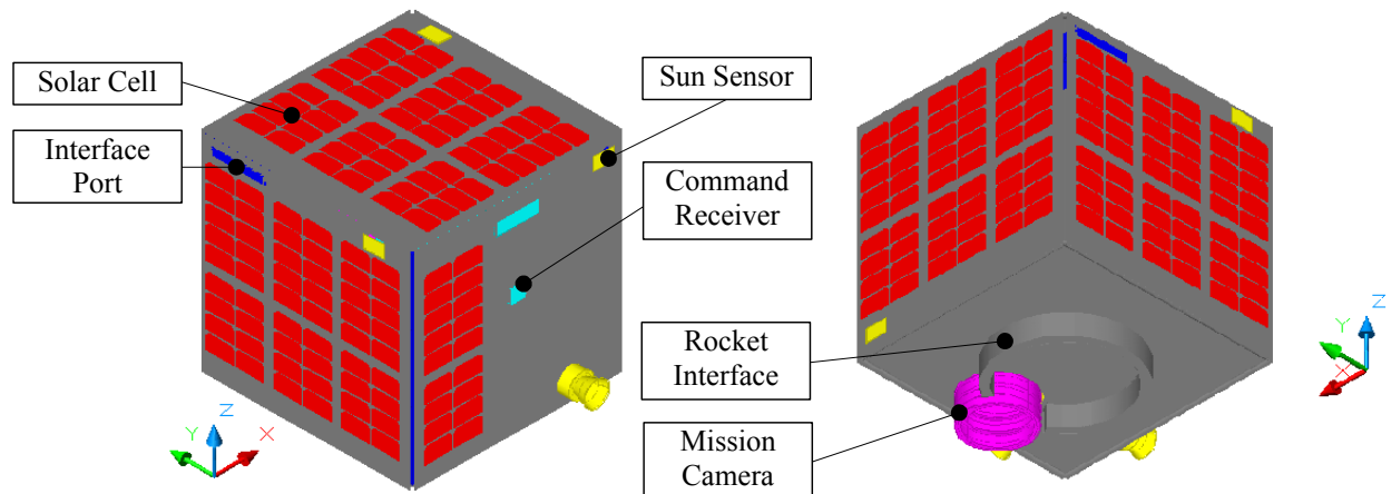
Figure 1. Schematic of satellite model.
