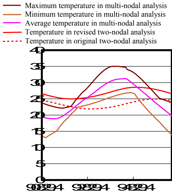
Figure 15. Comparison of temperature history at inner structure under worst hot case between two- and multi-nodal analyses.
