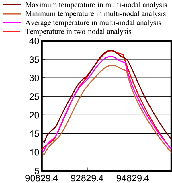
Figure 13. Comparison of temperature history at outer structure under worst hot case between two-nodal analysis with revised absorption at solar cells and multi-nodal analysis.
