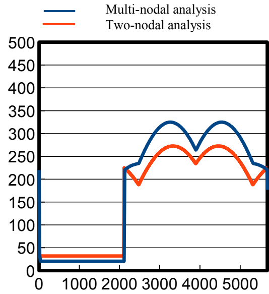
Figure 12. Comparison of absorbed heating rate history at solar cell under worst cold case between two- and multi-nodal analysis.
