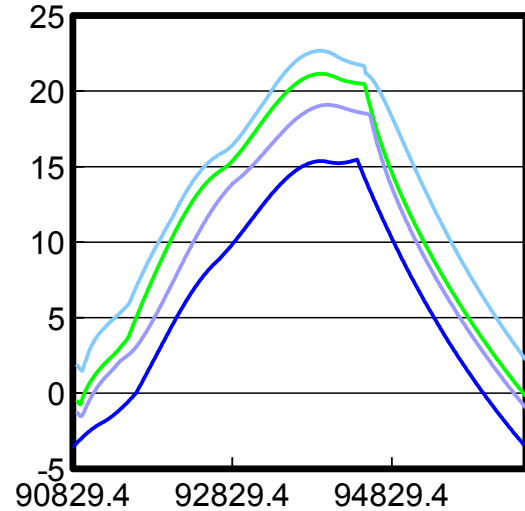
Figure 10. Comparison of temperature history at outer structure under worst cold case between two- and multi-nodal analyses.
