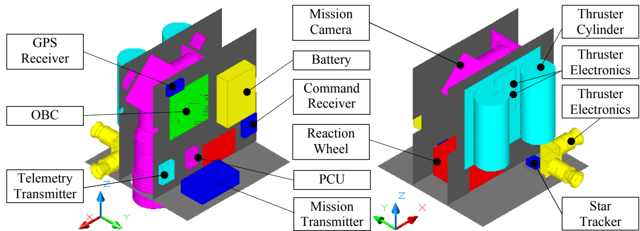
Figure 2. Configuration of components and inner structure.
