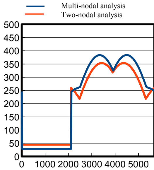
Figure 11. Comparison of absorbed heating rate history at solar cell under worst hot case between two- and multi-nodal analysis.
