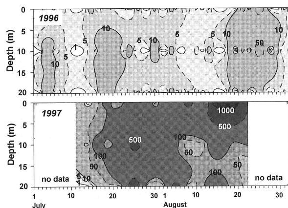
Fig. 5. Cell densities of Chaetoceros spp. (cells \text{ml}^{-1} ) in 1996 and 1997.
