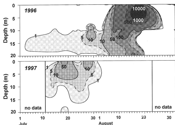
Fig. 4. Cell densities of K. mikimotoi (cells \text{ml}^{-1} ) in 1996 and 1997.
