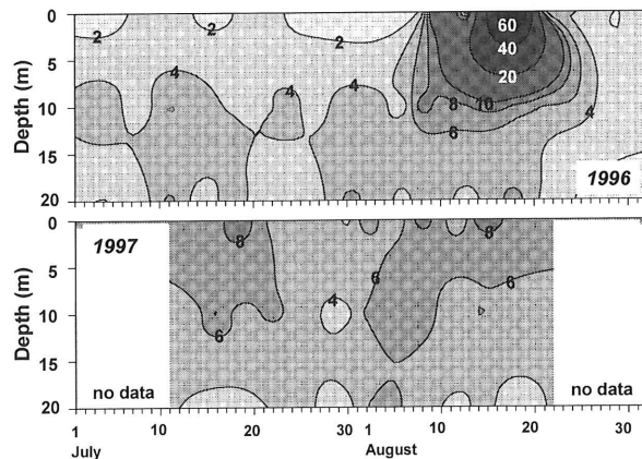
Fig. 6. Chl a concentrations ( \mu\text{g l}^{-1} ) in 1996 and 1997.
