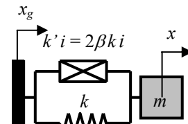
(b) Complex stiffness model
