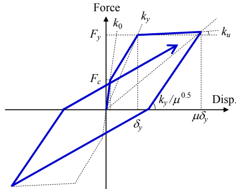
Fig. 7 Restoring force characteristics.
