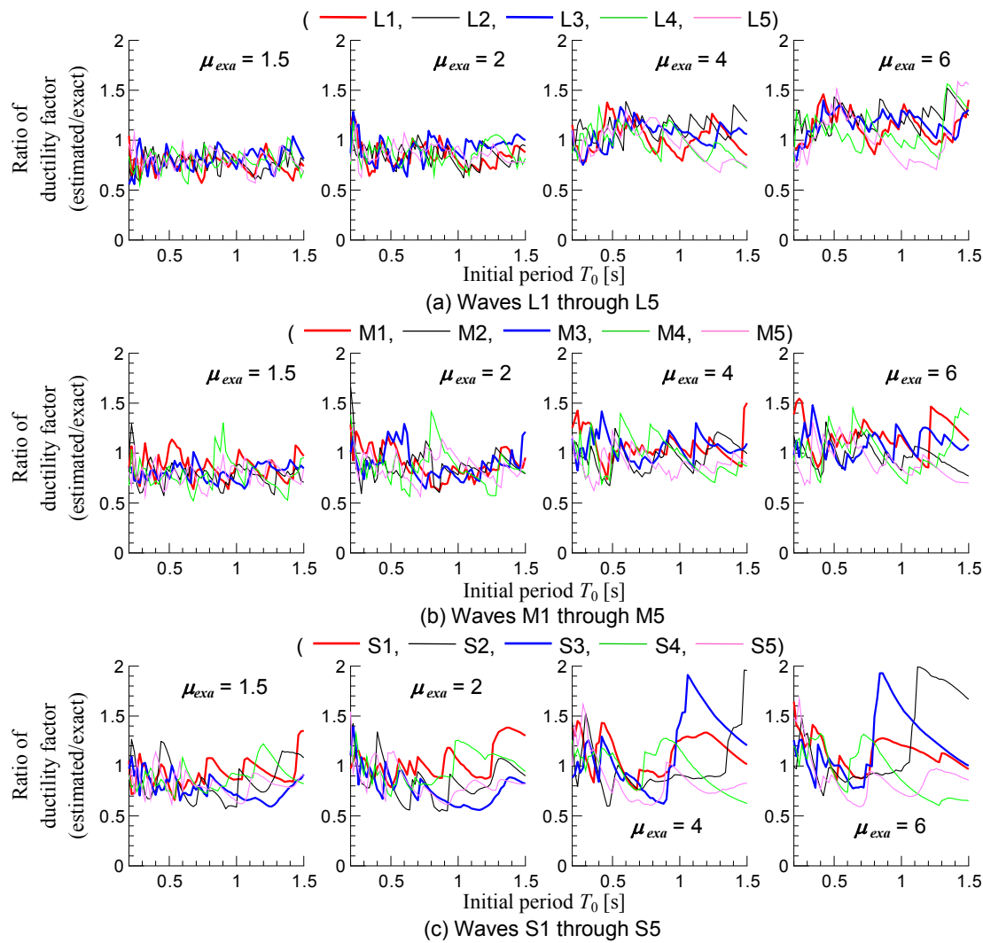
Fig. 13 Ratio of estimated ductility factor \mu_{est} to exact ductility factor \mu_{exa} (existing method using Eq. (15b)).
