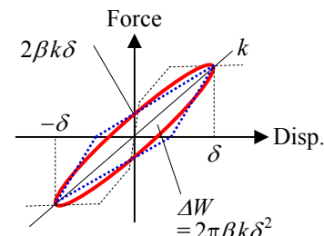
(a) Equivalent linearization
