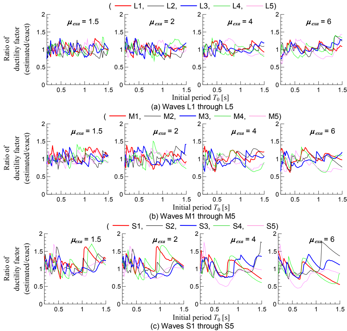
Fig. 11 Ratio of estimated ductility factor \mu_{est} to exact ductility factor \mu_{exa} (proposed method).
