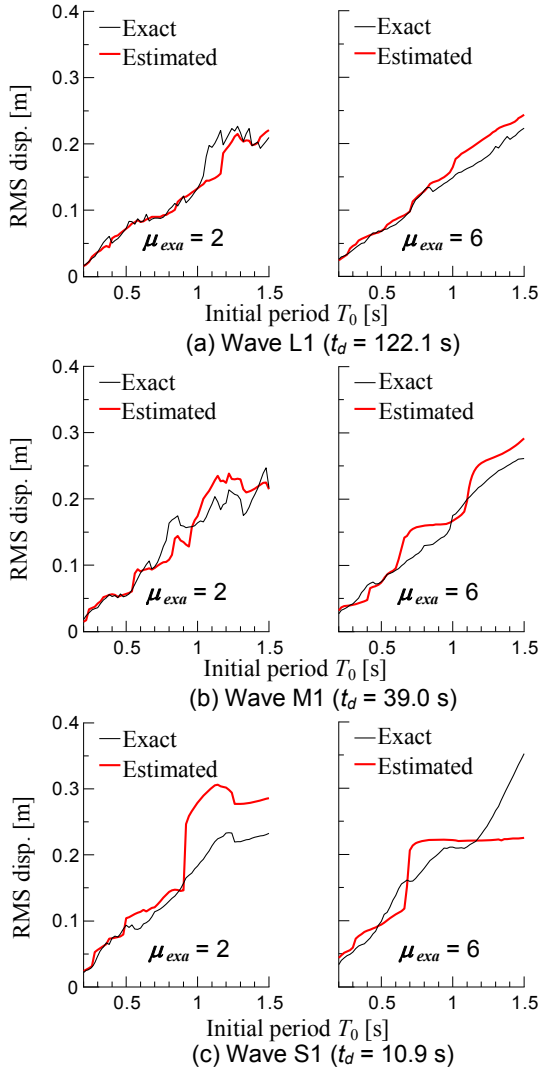
Fig. 9 RMS response displacement (proposed method).
