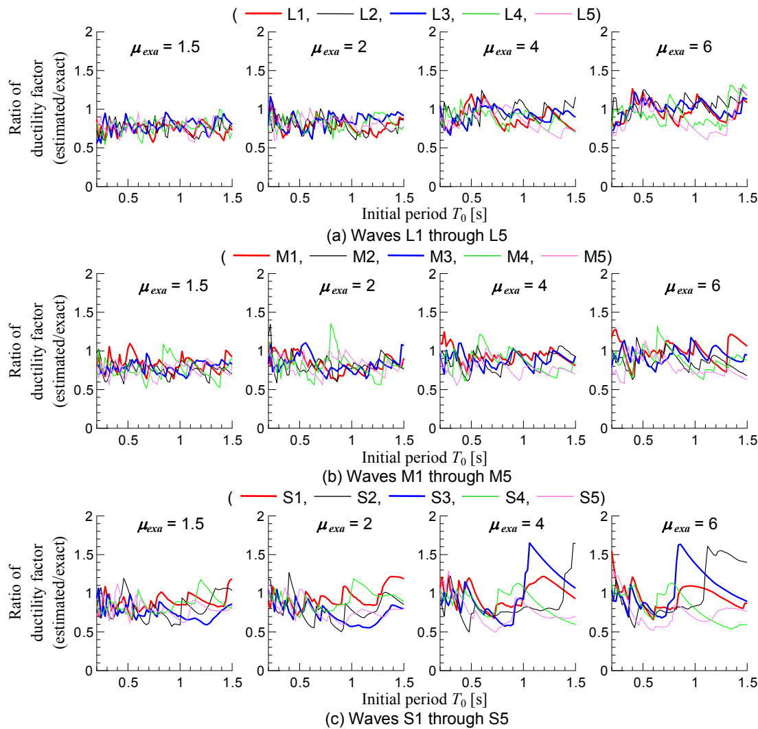
Fig. 12 Ratio of estimated ductility factor \mu_{est} to exact ductility factor \mu_{exa} (existing method using Eq. (15a)).
