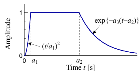
Fig. 5 Time envelope functions of input motions.
