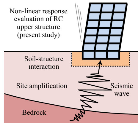
Fig. 1 Overview of research (development of comprehensive earthquake-resistant-design method).
