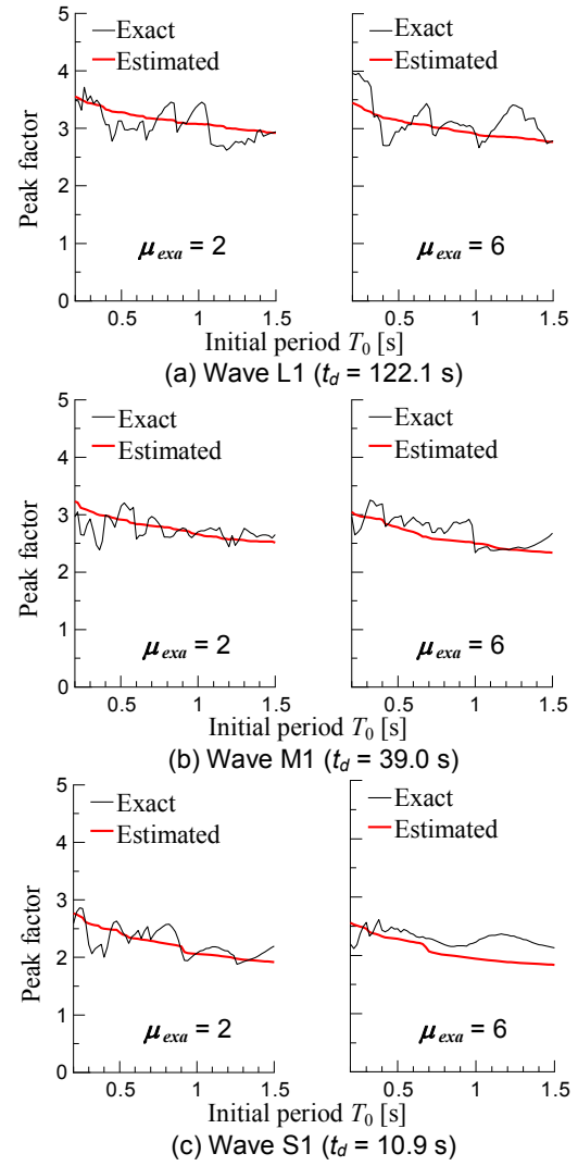
Fig. 10 Peak factor (proposed method).
