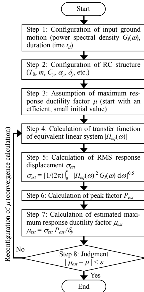
Fig. 2 Flowchart of the proposed method.
