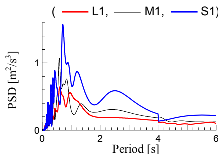
Fig. 4 Power spectral densities of input motions (one-sided PSD, smoothed by a Parzen window with a bandwidth of 0.5 Hz).
