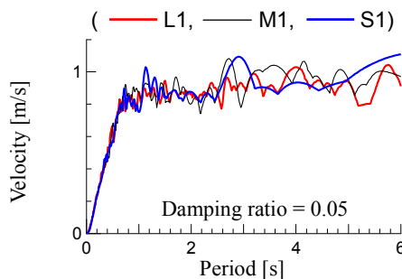
Fig. 3 Velocity response spectra of input motions.
