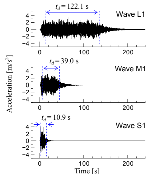
Fig. 6 Time history accelerations of input motions.
