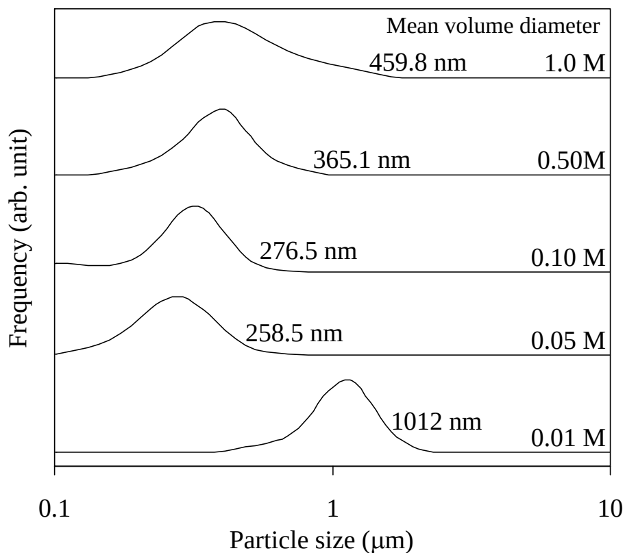
Figure 3 particle size distributions of the products at different electrolyte concentrations. Particle sizes were measured by dynamic light scattering. The particle size was decreased with decreasing the electrolyte concentrations. At 0.01 M, particle size was big because of the \text{Sn}_6\text{O}_4(\text{OH})_4 crystals formation.
