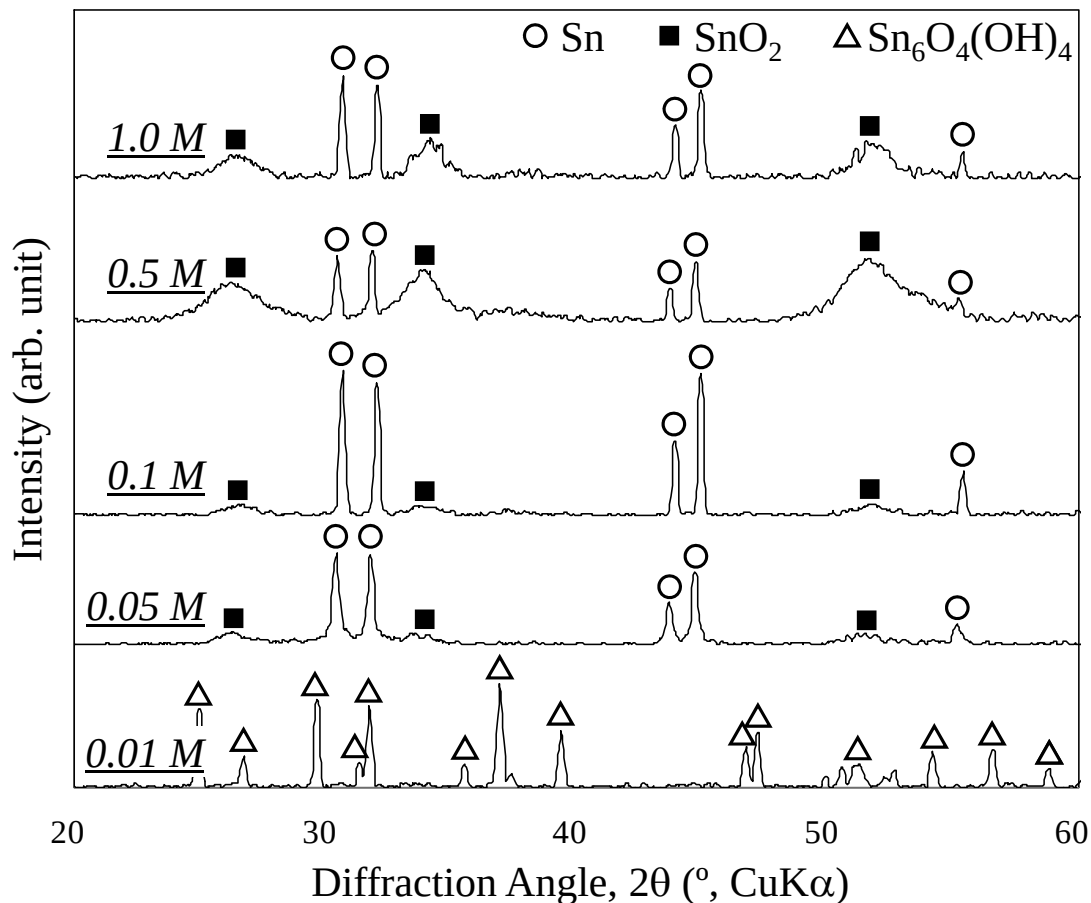
Figure 2 XRD patterns of the products synthesized at different KCl concentrations of the electrolyte. From 0.05 to 1.0 M of KCl, Sn and \text{SnO}_2 phases were formed. In contrast, the 0.01 M concentration of KCl, the \text{Sn}_6\text{O}_4(\text{OH})_4 were synthesized.
