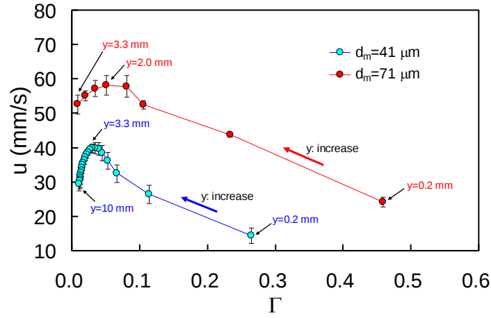
Fig. 9. Relationship between \Gamma and u at x=500 mm.
