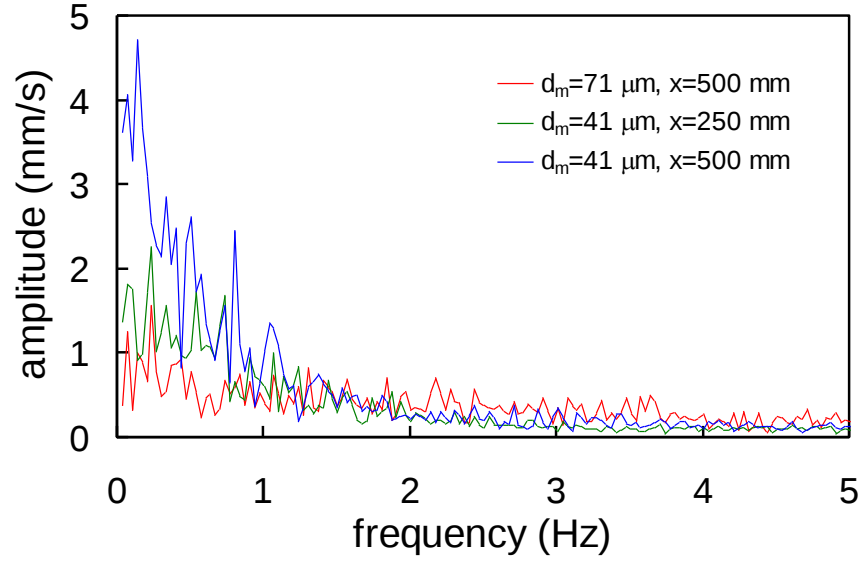
Fig. 13. Spectrum of u_a .
