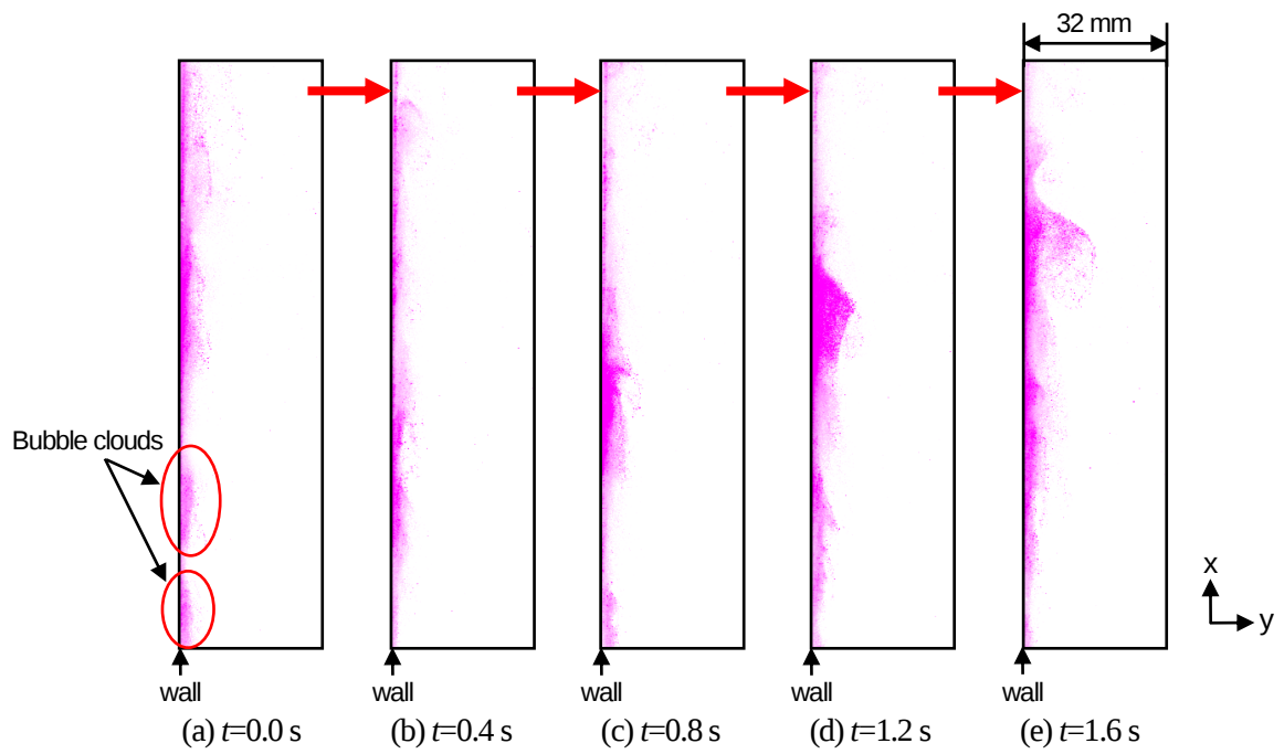
Fig. 17. Typical time-series of images of bubbles near the wall for d_m=41\ \mu\text{m} at x=500\ \text{mm} .
