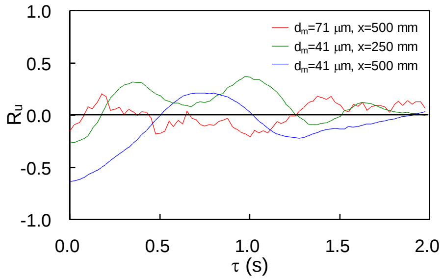
Fig. 14. Cross-correlation between L_a' and u_a' .
