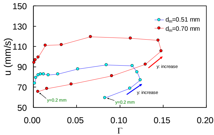
Fig. 11. Relationship between \Gamma and u at x=170 mm for sub-millimeter-bubble flows obtained using Kitagawa et al.'s experimental results (Kitagawa et al., 2009).
