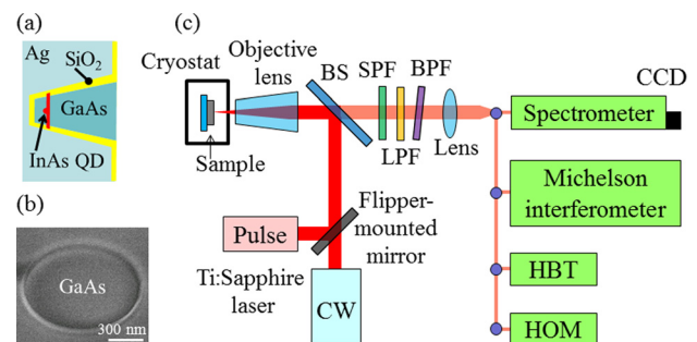
FIG. 1. (a) Schematic of an Ag-embedded nanocone structure with a thin SiO 2 insulator layer between the Ag and the semiconductor part. (b) Top-view SEM image. (c) Measurement setup.
