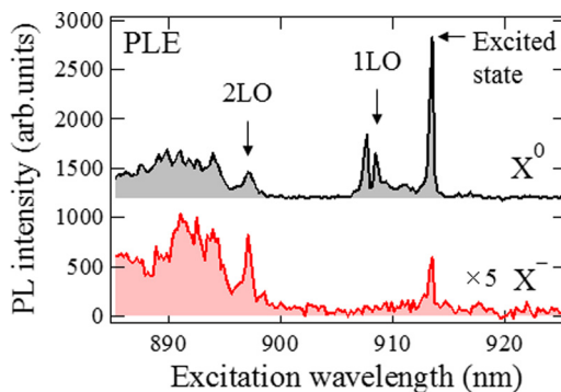
FIG. 5. PLE spectra measured on X^0 and X^- emissions. It should be noted that the PLE spectrum of the X^- line is multiplied by 5.
