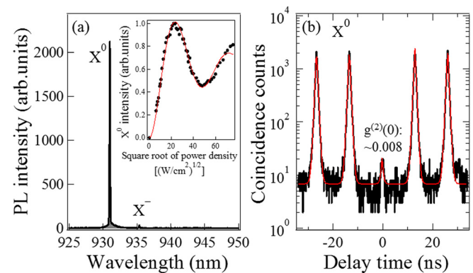
FIG. 6. (a) PL spectrum measured under the quasi-resonant excitation. The inset shows the Rabi oscillation of the X^0 emission intensity. (b) Semi-log plot of the measured second-order intensity correlation of the X^0 emission under the \pi -pulse excitation. The red curve is the theoretical fit to the data. 36
