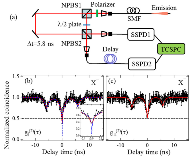
FIG. 4. (a) Schematic of CW two-photon interference measurement. A fixed time delay between two optical paths was 5.8 ns. (b) and (c) are the normalized two-photon interference coincidences of the X^- line under parallel and orthogonal polarizations, respectively. The inset in (b) is the zoom-in near the central dip. The horizontal dashed line corresponds to the g^{(2)}(0) = 0.5 level. The solid curves in (b) and (c) are calculated for parallel and orthogonal polarizations, respectively, with Eqs. (3) and (4) by taking the convolution with the IRF. The dashed curve in (b) is the calculation without the convolution.
