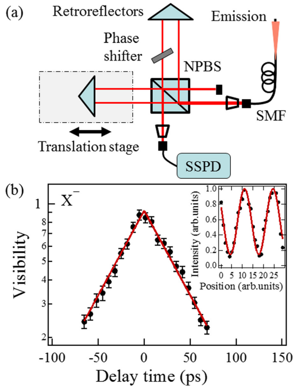
FIG. 3. (a) Experimental setup of Michelson interferometer for measuring the coherence time. NPBS: non-polarizing beam splitter. The phase shifter was introduced to record the interference fringes at a fixed optical-path length difference set by the translation stage. (b) The visibility as a function of delay time for the X^- emission. The inset shows an example of interference fringes at a position close to zero time delay.
