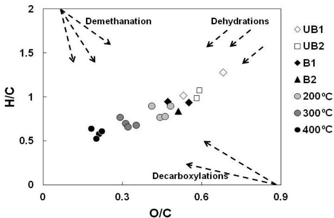
Fig. 4.2. The Van Krevelen plot (H/C vs O/C ratios) of humic acids collected from Sebangau soil (UB1), Forest soil (UB2), Deforest soil (B1), Burnt soil in Kereng (B2) and thermally treated samples (200, 300, 400 °C).
