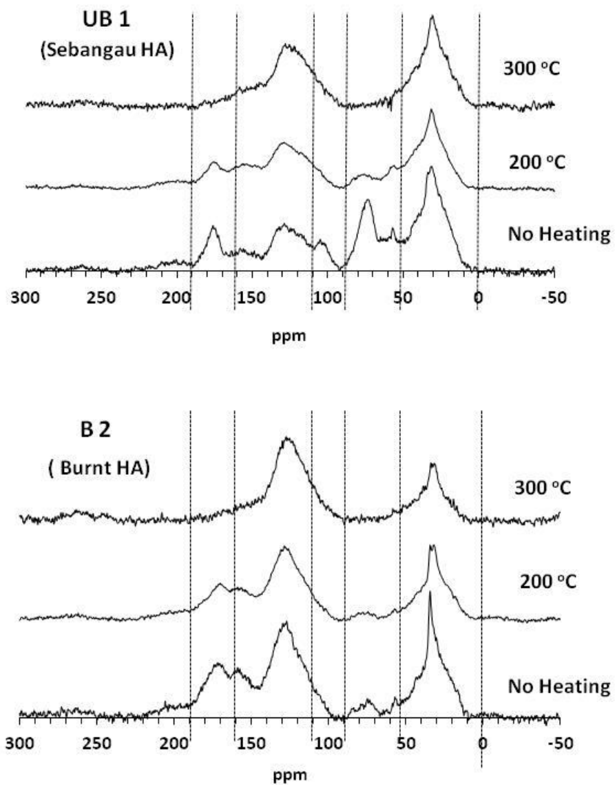
Fig.4.3. CP/MAS ^{13}\text{C} -NMR spectra of humic acids from unburnt site (UB1), burnt site (B2) and thermally treated samples (200, 300 °C)
