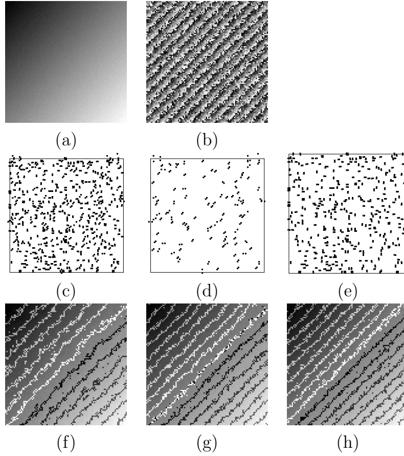
Figure 4.5: A comparison of the unwrapped phase results for simulated phase data has noise with \sigma = 0.15 cycle: (a) the original phase data, (b) the wrapped data, (c) the positions of all SP pairs, (d) the positions of the pairs of non-adjointing SPs, (e) the positions of the pairs of adjoining SPs, (f) unwrapped result by LS-DCT, (g) unwrapped result by RC, and (h) unwrapped result by RC+DC. In (a), (b), and (f)-(h), the phase increases with the increases of brightness. In (f)-(h), contour lines of the phase with the interval of one cycle are also shown.
