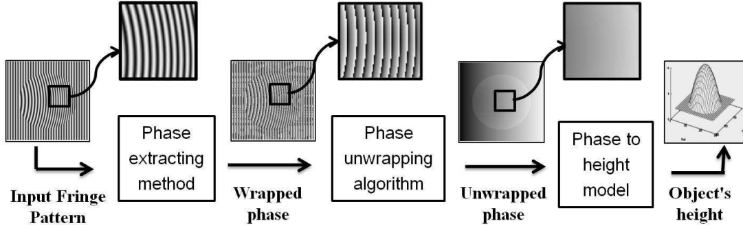
Figure 1.1: Fringe analysis for an object
