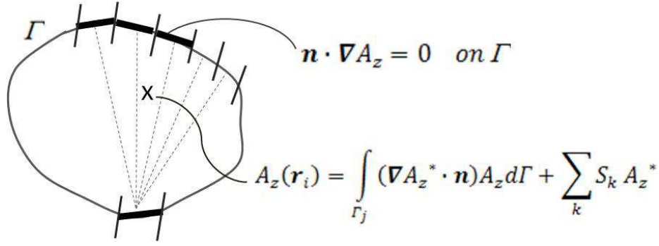
Figure 5.7: Schematic of BEM to solve flux density A_z : shows the steps of BEM to compute the flux, the condition in boundary \Gamma is \hat{\mathbf{n}} \cdot \nabla A_z = 0 , and for internal point inside the specific domain is, A_z(\mathbf{r}_i) = \int_{\Gamma_i} (\nabla A_z^* \cdot \hat{\mathbf{n}}) A_z d\Gamma + \sum_k S_k A_z^* .
