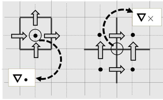
Figure 5.11: A schematic for the proposed algorithm to illustrate the way for solving Poisson's equation to compute the flux values. This way uses rotational, (\nabla \times) , and divergence, (\nabla \cdot) operators to produce the flux density values directly without any integration to evaluate the compensators.
