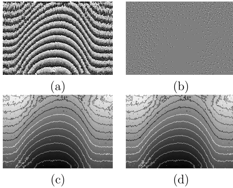
Figure 5.16: Unwrapped phase results of experimental data for candle flame: (a) wrapped data, (b) SPs distribution map (positive and negative SPs are represented by white and black dots, respectively), (c) unwrapped result of the old LC method (LC.bem+svd), and (d) unwrapped result obtained by the proposed method (LC.rot+div). In (c) and (d), contour lines of the phase with the interval of one cycle are also shown.
