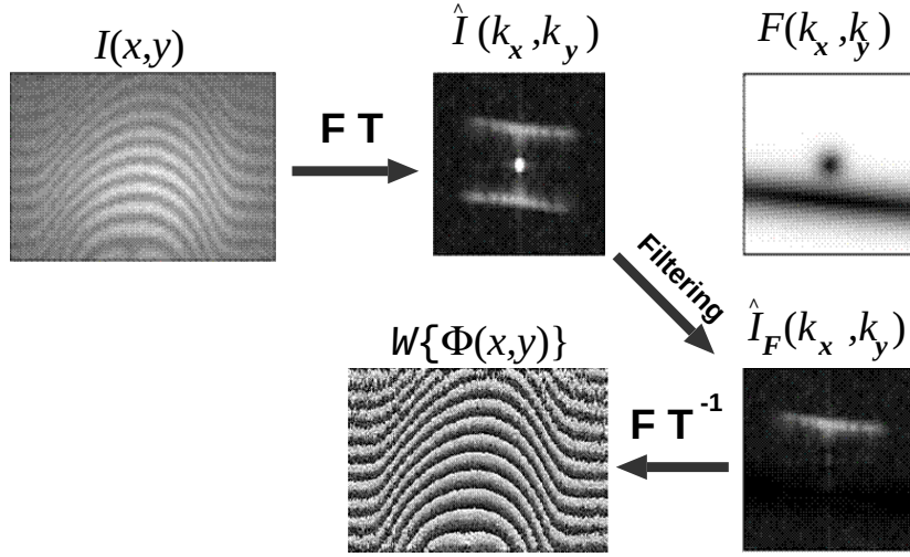
Figure 2.2: Procedure for calculating the phase from an interferogram: FT Fourier transformation, FT^{-1} inverse Fourier transformation, the I(x, y) is a fringe pattern for interferometric data, the \hat{I}(k_x, k_y) shows Fourier spectrum of the fringe pattern, the F(k_x, k_y) shows the filtering function, the \hat{I}_F(k_x, k_y) shows the filtered spectrum, the W\{\Phi(x, y)\} is the wrapped phase modulation.
