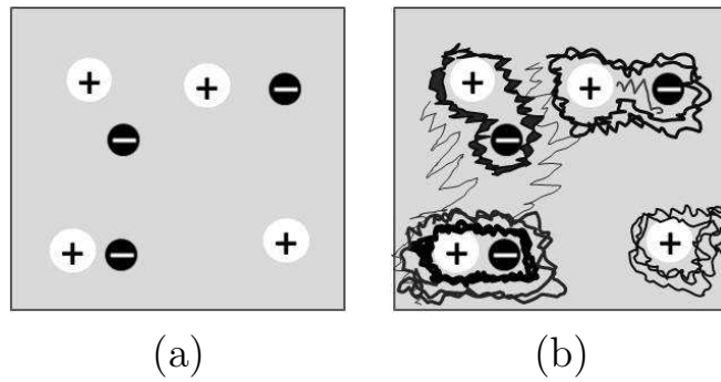
Figure 2.10: Spreading of errors in regular regions due to the SSPU method handling way for the singularity regions in the phase map: (a) SPs distribution map, (b) phase errors appear in regular regions.
