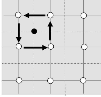
Figure 2.4: Elementary path in two-dimensional coordinate for visualizing SP identification: the white circles denote points at which the phase values are defined, the thick arrows denote the direction of the path around the tested SP, the black circle illustrates the position of the tested SP.
