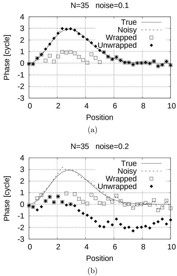
Figure 1.4: One-dimensional phase unwrapping noisy examples: (a) successful example has noise with magnitude 0.1 and sample points number is 35; (b) unsuccessful example has noise with magnitude 0.2 and sample points number is 35.
