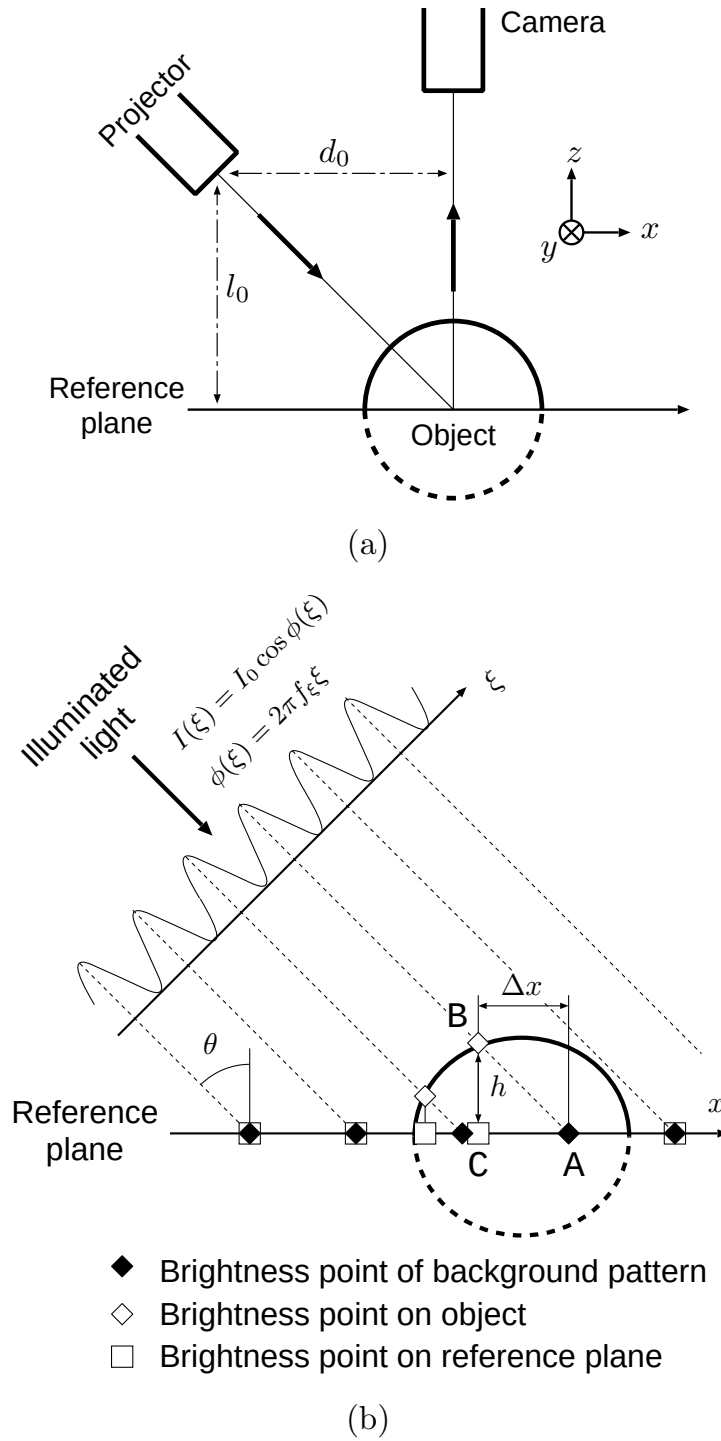
Figure 2.3: Experimental setup of three-dimensional shape measurement system. (a) geometry for the projecting and imaging grating pattern on the object, (b) sketch map for projected light pattern.
