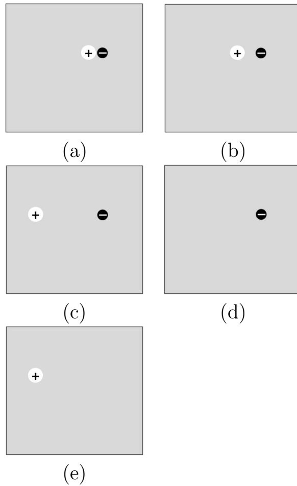
Figure 2.6: Schematic figure shows SPs types: (a) one pixel apart dipole SPs generated by phase noise, (b) dipole SPs generated by phase noise several pixels apart, (c) dipole SPs generated by discontinuous objects and under-sampling have the tendency of lying far apart from each other and (d) & (e) are monopole SPs.
