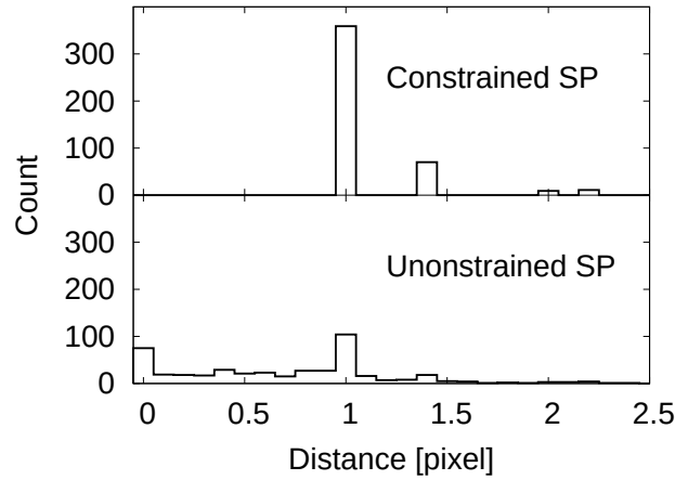
Figure 3.6: Frequency histogram for distance from a positive SP to the nearest negative SP.
