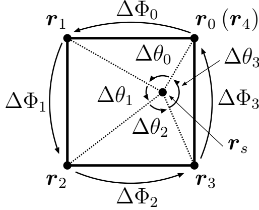
Figure 3.2: Elementary path including an unconstrained singular point: The \Delta\theta_l means the facing angle of the side with the ends r_l and r_{l+1} . The \Delta\Phi_l means the difference of the wrapped phases.
