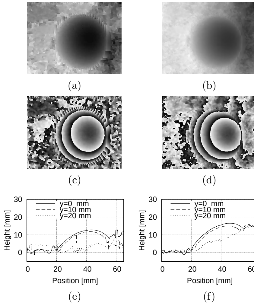
Figure 4.12: Comparison of the accuracy of the examined phase unwrapping algorithms' results for the measured data: the first row shows the unwrapped phase shift of the object, the second row shows the rewrapped phase shift of the object, the third row shows the cross-sectional profile of the object's height. (a), (c), and (e) show the results of Flynn's method. (b), (d), and (f) show the results of RC+DC algorithm.
