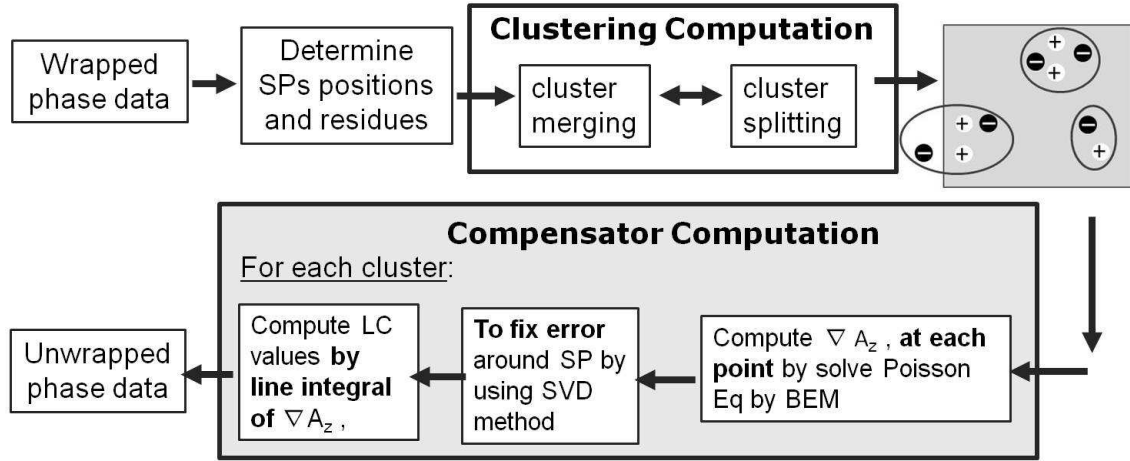
Figure 5.4: A flowchart of the original LC method (LC.bem+svd) shows the two main steps for this method.
