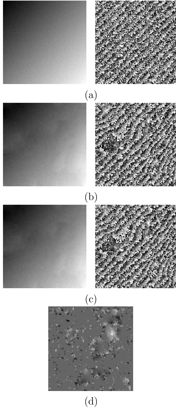
Figure 5.13: A comparison of the unwrapped phase results for simulated phase data has noise with \sigma = 0.2 [cycle]: (a) the original and wrapped phase data, (b) the unwrapped and rewrapped results obtained by the old LC method (LC.bem+svd), (c) the unwrapped and rewrapped results obtained by the proposed modified LC method (LC.rot+div), (d) the phase difference between the unwrapped results the range of values is [-0.1\pi : 0.2\pi] . The left side in (a) to (c), the phase increases with the increases of brightness.
