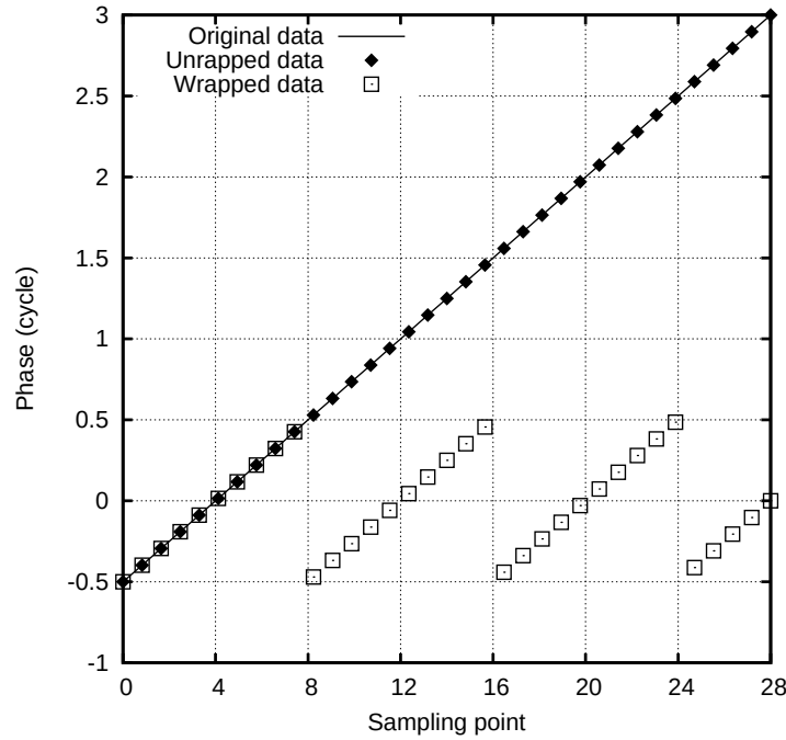
Figure 1.2: Concept of phase unwrapping technique
