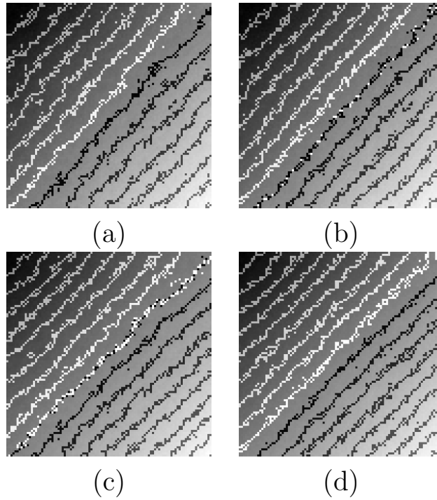
Figure 3.7: Unwrapped phase results with contour lines for simulated noisy data with 0.15 cycle standard deviation, obtained when uses: (a) RC technique only, (b) RC technique with using USP approach only, (c) RC technique with using VSP approach only, (d) RC technique with using both USP and VSP approaches.
