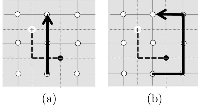
Figure 2.5: Unwrapping path with the existence of the branch cuts in the phase map: the thick dashed line denotes the branch cut that connects two of opposite sign SPs, the thick arrow shows the direction of unwrapping path; (a) incorrect unwrapping path, (b) correct unwrapping path.
