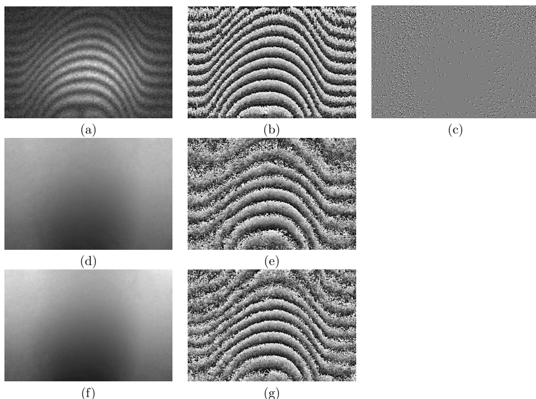
Figure 3.9: Unwrapped phase of fringe by Mach-Zehnder interferometer for candle flame: (a) fringe pattern obtained with existence of flame, (b) wrapped phase map obtained by Fourier domain method, (c) SPs distributions, (positive and negative SPs are represented by white and black dots, respectively), (d) & (e) unwrapped and rewrapped phases map obtained by LS-DCT method, (f) & (g) unwrapped and rewrapped phases map obtained by the developed RC method.
