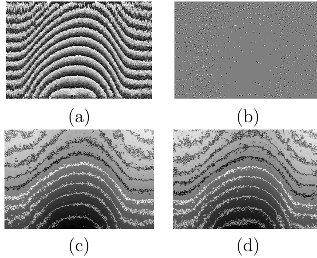
Figure 4.7: Unwrapped phase result of experimental data for candle flame: (a) the wrapped data, (b) SPs distribution map, (positive and negative SPs are represented by white and black dots, respectively); (c) the unwrapped result of RC algorithm, (d) the unwrapped result of RC+DC,
