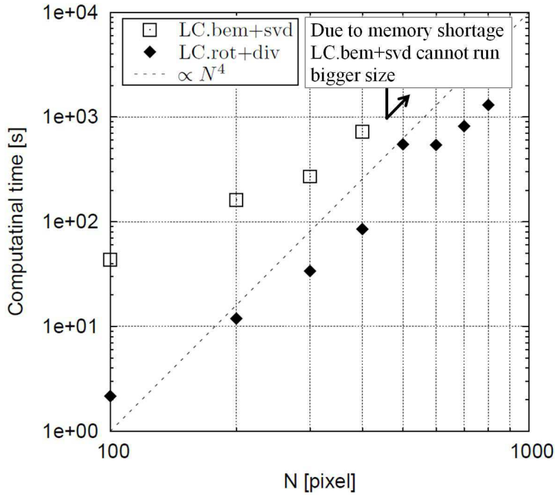
Figure 5.14: Required computational time of each algorithm for various image sizes: The horizontal axis N denotes one-dimensional area size in pixels. “LC.bem+svd” shows the required time cost for the old LC method, and “LC.rot+div” shows the required execution time for the proposed method.
