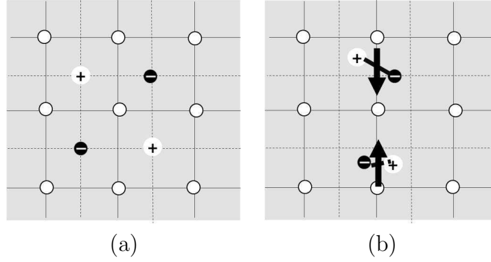
Figure 4.3: Complex cases for the position patterns of SP pairs and the direct compensators for the adjoining SPs pairs: (a) SPs are distributed in discrete values, (b) SPs are distributed by using USP technique; in (b) the thick dashed line denotes the branch cut that connects two SPs of opposite sign and also shows the direct compensator positions are denoted by thick arrows.
