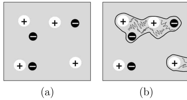
Figure 5.3: Spreading of errors in regular regions due to the handling way of the LC method for the singularity regions in the phase map: (a) SPs distribution map, (b) phase errors appear in regular regions.
