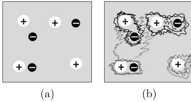
Figure 3.3: Spreading of errors in regular regions due to the RC method handling way for the singularity regions in the phase map: (a) SPs distribution map, (b) phase errors appear in regular regions.
