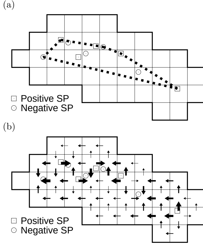
Figure 5.6: Definition of local domain and flux density around SPs: (a) local domain including SPs, (b) flux distribution in the local domain. Outmost closed thick line is a boundary of the local domain, and the grids are segments of elementary loops. The dashed line in (a) represents concave polygon that contains all SPs. The arrows in (b) are the flux density of which line width expresses the magnitude.
