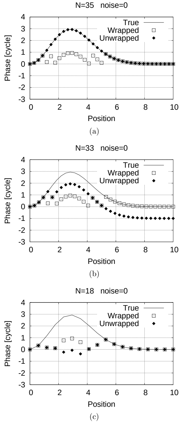
Figure 1.3: One-dimensional phase unwrapping examples: (a) successful example with sufficient sample points number is 35; (b) unsuccessful example with insufficient sample points number is 33, which is slightly under Nyquist rate; (c) unsuccessful example with insufficient sample points number is 18.
