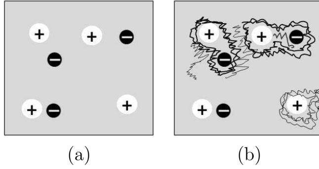
Figure 4.4: Spreading of errors in regular regions due to the proposed method (RC+DC) handling way for the singularity regions in the phase map: (a) SPs distribution map, (b) phase errors appear in regular regions.
