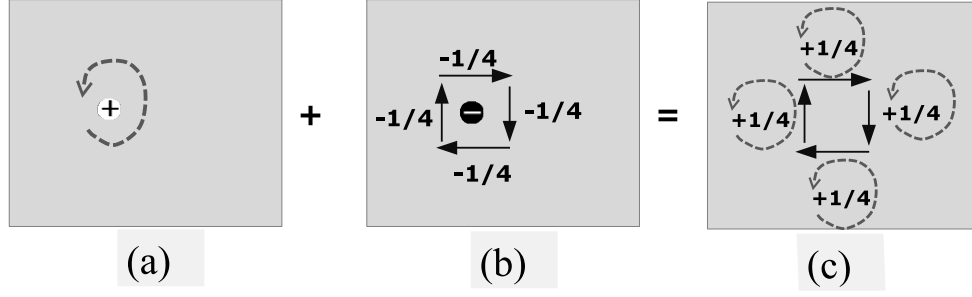
Figure 2.9: Schematic of the singularity spreading phase unwrapping: (a) singular point, (b) compensator, (c) spread singularity.
