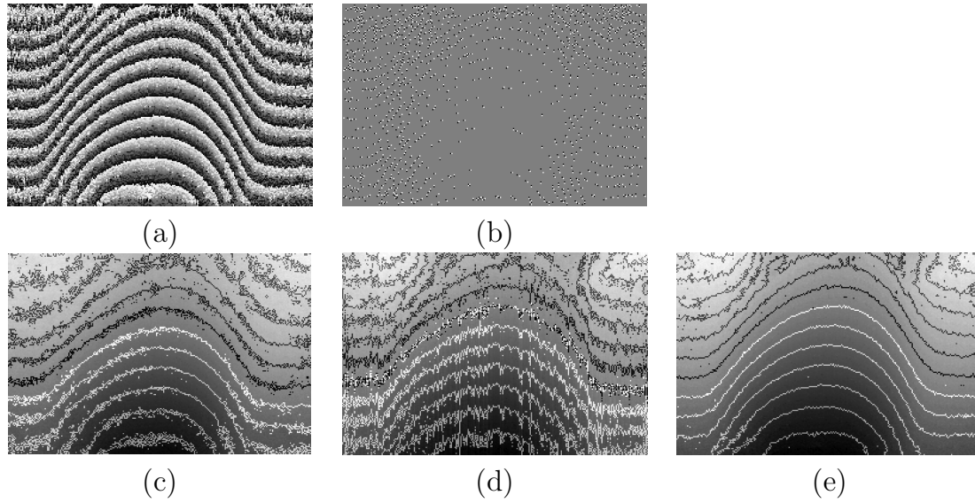
Figure 5.10: Accuracy comparison for unwrapped phase results of experimental data for candle flame: (a) wrapped data, (b) SPs distribution map (positive and negative SPs are represented by white and black dots, respectively), (c) unwrapped result of the RC+DC method, (d) unwrapped result of the old LC method by using BEM only, and (e) unwrapped result obtained by the old LC method using both BEM and SVD. In (c), (d) and (e), contour lines of the phase with the interval of one cycle are also shown.
