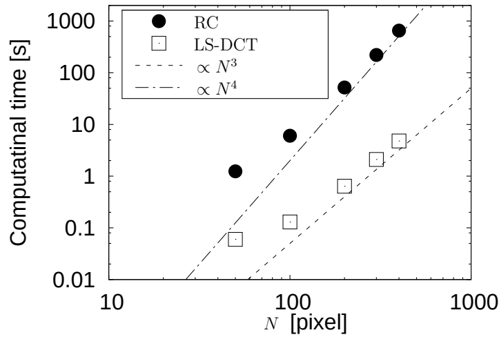
Figure 3.8: Computational time: The horizontal axis N denotes one-dimensional area size in pixels. The computational time is measured with a PC including CPU of Intel Core 2 DUO (TM) with 2.13GHz clock in a single CPU operation mode.
