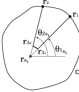
Figure 3.1: Configuration to compute the rotational compensator
