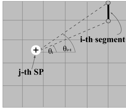
Figure 5.1: Schematic of rotational compensator phase unwrapping method: the singularity of j -th SP is canceled by computing the RC of i -th segment using eq. (5.1).
