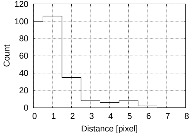
Figure 4.1: Example of dipole distance distribution: the dipole distance is defined as the distance between one SP and the closest SP with opposite polarity.
