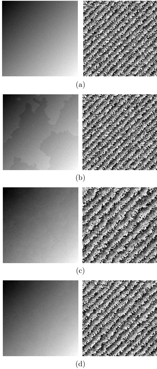
Figure 3.5: Unwrapped and rewrapped phase map of simulated phase data has noise with \sigma = 0.15 cycle: In each figure, the left-hand side figure shows original or unwrapped phase map where phase increases with increasing of brightness, and the right-hand side figure shows wrapped or rewrapped phase map. (a) original phase map, (b) Goldstein's path-following method, (c) least squares method with DCT, (d) RC method.
