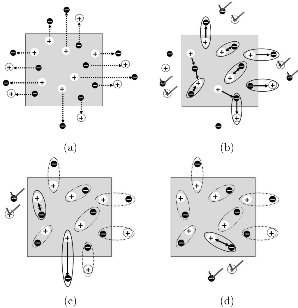
Figure 3.4: Determination of dipole pairs: (a) definition of the virtual SP candidates, each dashed arrow shows the correspondence between original and virtual SP; (b) search nearest SP and pairing in the first iteration: each arrow shows the nearest opposite-signed SP, the SPs encircled are paired as dipoles, the checked virtual candidate is removed from the list of candidates in subsequent steps; (c) the second iteration: SPs enclosed with dashed ellipse have been already paired; (d) elimination of removable virtual SP pairs.
