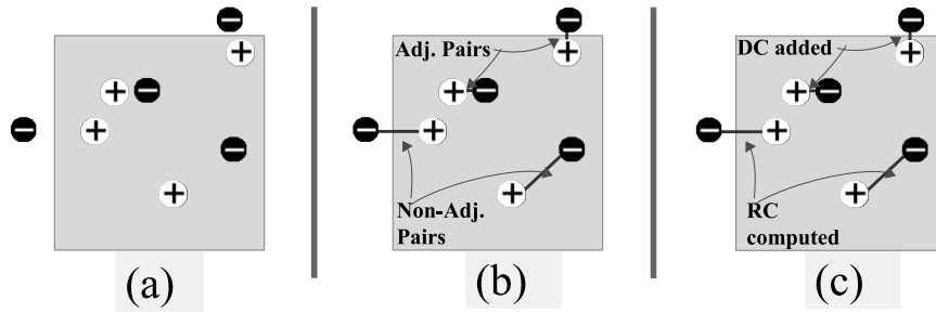
Figure 5.2: Schematic of rotational and direct compensator phase unwrapping method: (a) defined SPs, (b) create SPs pairs and defined adjoining and nonadjoining pairs, (c) add DC for adjoining pairs and compute RC for nonadjoining pairs.
