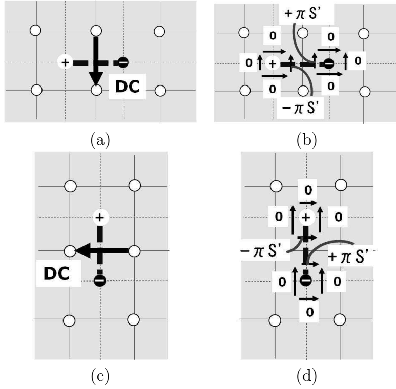
Figure 4.2: The existence of the branch cuts between the adjoining SPs and the concept of direct compensation: the thick dashed line denotes the branch cut that connects two SPs of opposite sign, compensator position is denoted by thick arrow, the thin arrows show the direction and distribution of compensators for the segments of each SP where S and S' denote the residues of the SPs.
