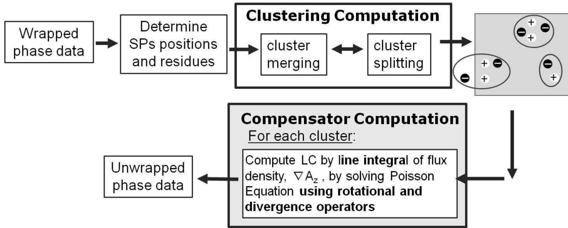
Figure 5.12: A flowchart of the proposed algorithm (LC.rot+div).
