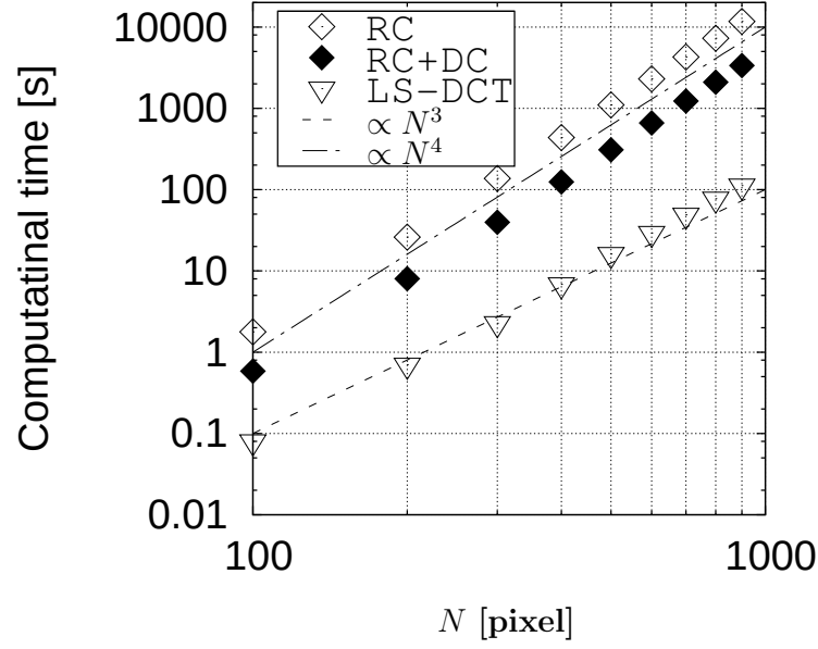
Figure 4.6: Required computational time of each algorithm for various image sizes: The horizontal axis N denotes one-dimensional area size in pixels. “RC” shows the required time cost for RC method, “RC+DC” shows the required execution time for the proposed method, and “LS-DCT” shows the required time cost for LS-DCT method. The computational time is measured with a PC including an Intel Core 2 DUO CPU with 2.13 GHz clock in the single CPU operation mode.
