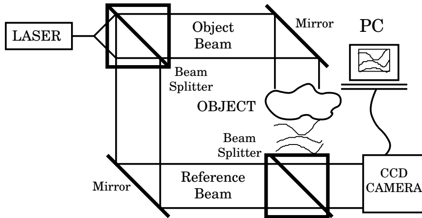
Figure 2.1: A schematic diagram of an experimental setup system of the interferometer technique measurement.
