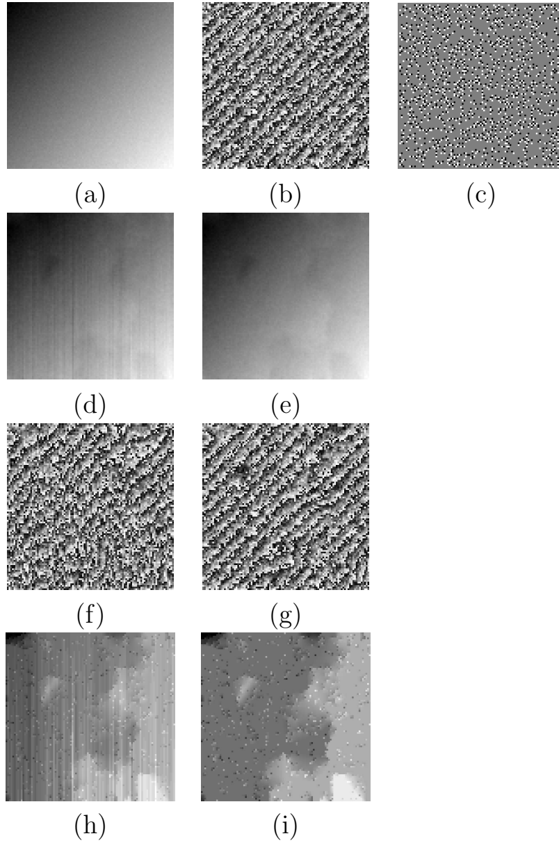
Figure 5.9: An example of unwrapped phase results for simulated phase data has noise with 0.2 cycle standard deviation to show the errors produce when use BEM only for the old LC method: (a) original phase data, (b) wrapped data, (c) SPs distribution map (positive and negative SPs are represented by white and black dots, respectively), (d) unwrapped result of the old LC method by using BEM only, (e) unwrapped result obtained by the old LC method using both BEM and SVD, (f) rewrapped result of the old LC method by using BEM only, (g) rewrapped result obtained by the old LC method using both BEM and SVD, (h) errors generated due to using of BEM only for unwrapped result the range of values is [-0.06\pi : 1.8\pi] , and (i) errors generated due to using both BEM and SVD to produce unwrapped result the range of values is [-0.05\pi : 1.3\pi] .
