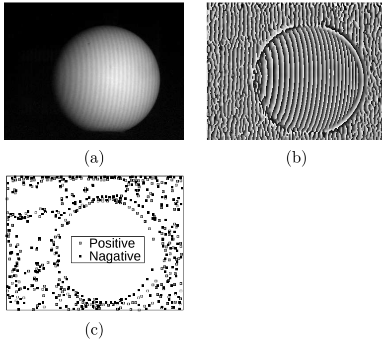
Figure 4.11: Experimental measured data: (a) deformed grating image, (b) wrapped phase image, and (c) map of distribution of SPs.
