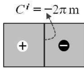
Figure 5.5: Example of two adjacent loops have two SPs with opposite polarity, presenting the compensator value for the internal segment.
