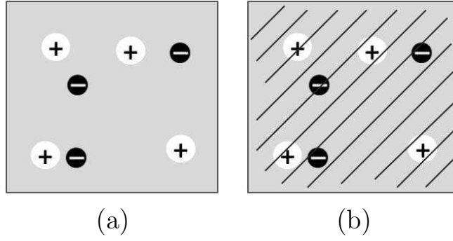
Figure 2.8: Spreading of errors in regular regions due to the LS-DCT method handling way for the singularity regions in the phase map: (a) SPs distribution map, (b) phase errors appear in regular regions.
