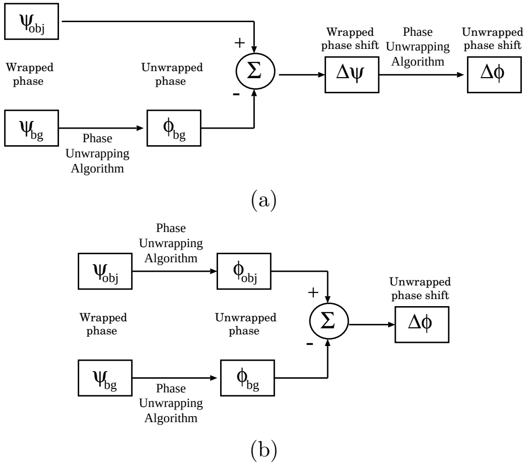
Figure 4.8: The way of an object extraction from experimental data: (a) pre-rejection of background. (b) Post-rejection of background.
