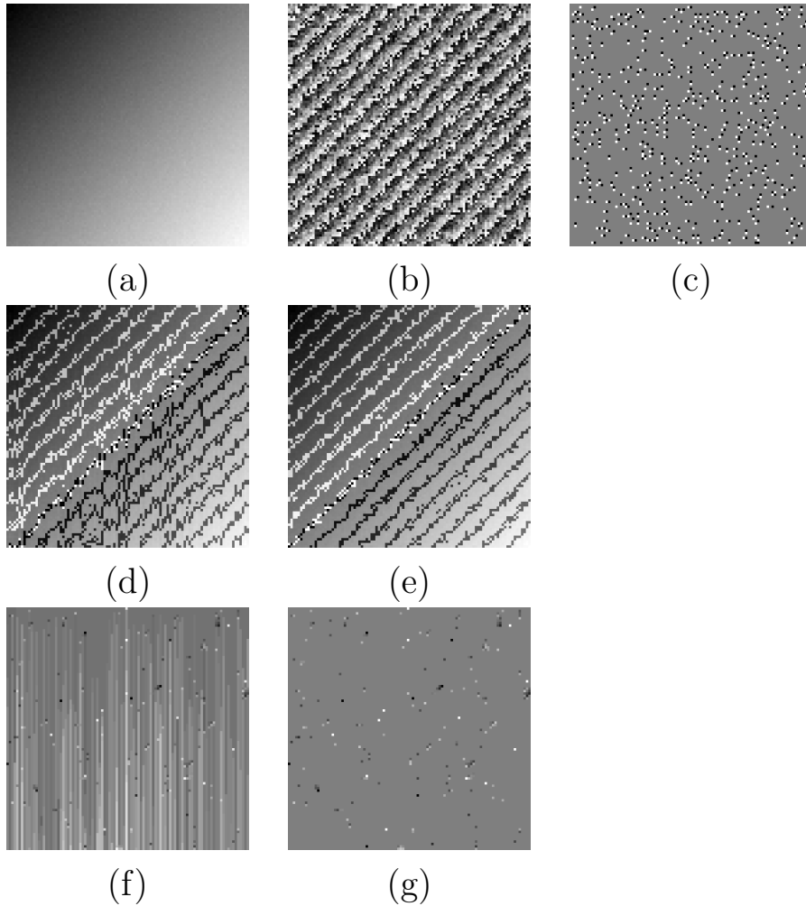
Figure 5.8: An example of unwrapped phase results for simulated phase data has noise with standard deviation 0.15 cycle, to show the errors produce when use BEM only for the old LC method: (a) original phase data, (b) wrapped data, (c) SPs distribution map (positive and negative SPs are represented by white and black dots, respectively), (d) unwrapped result of the old LC method by using BEM only, (e) unwrapped result obtained by the old LC method using both BEM and SVD, (f) errors generated due to using of BEM only for unwrapped result the range of values is [-0.3\pi : 0.4\pi] , and (g) errors generated due to using both BEM and SVD to produce unwrapped result the range of values is [-0.3\pi : 0.3\pi] . In (a), (b), and (d), (e), the phase increases with the increases of brightness. In (d), (e), contour lines of the phase with the interval of one cycle are also shown.
