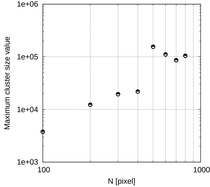
Figure 5.15: The maximum cluster size for various image sizes: The horizontal axis N denotes one-dimensional area size in pixels.
