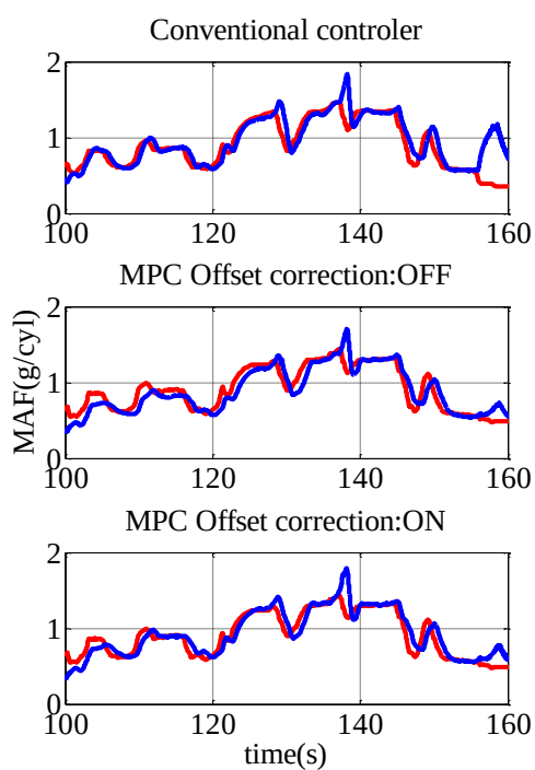
(c) MAF
