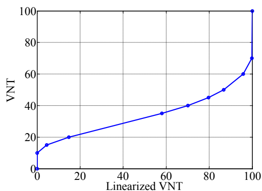
(b) VNT
