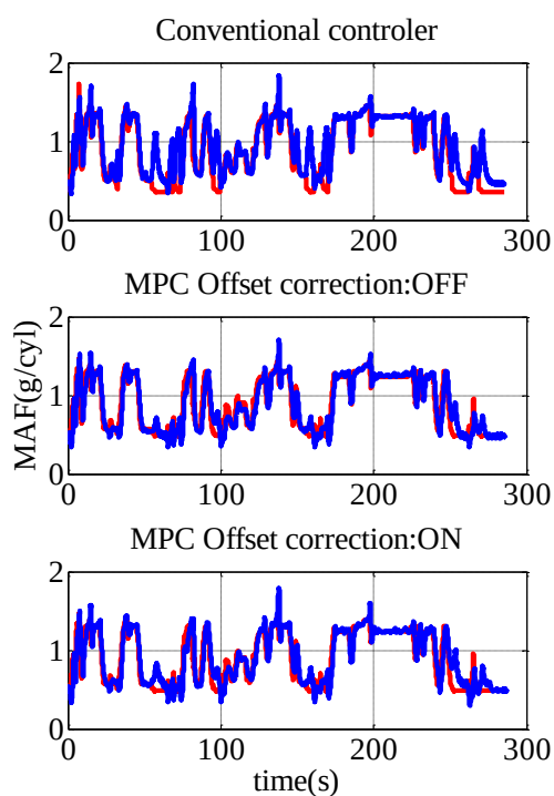
(c) MAF
