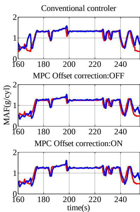
(c) MAF
