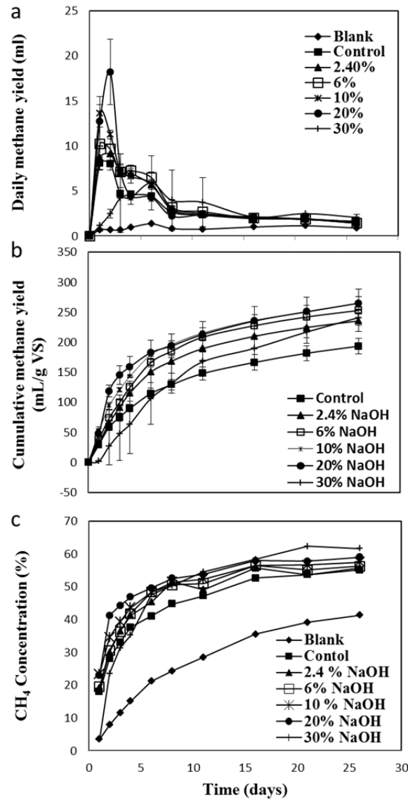
..... Fig. 3.2 Methane production of low loading rate NaOH- pretreated 2POMW(0.35 g-VS (substrate) /g-VS (inoculum) ) (a) Daily methane yield, absolute volume of methane gas produced from 100 mL reactor working volume (b) Cumulative methane yield, Values represent the methane production in all treatments minus the blank, values are represented as per volatile solid 2POMW (c) CH 4 concentration (%)
