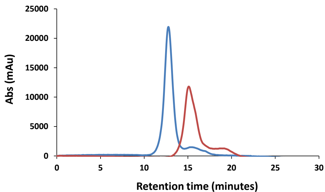
Figure 3-3. Gel filtration chromatogram of Pd4-p53Tet (Blue) and Pd4-p53Mono (Red). The longer retention time of Pd4-p53Mono compared to Pd4-p53Tet confirms that the monomeric variant is incapable of forming tetramers.
