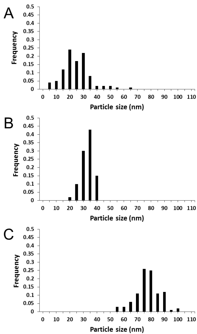
Figure 2-3. Size distribution histogram of 100 particles. Histogram increment is 5 nm. A) No buffer, B) Tris, C) HEPES
