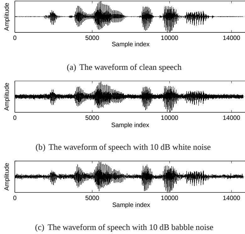
Figure 2.7. The waveforms of speech with white and babble noises
