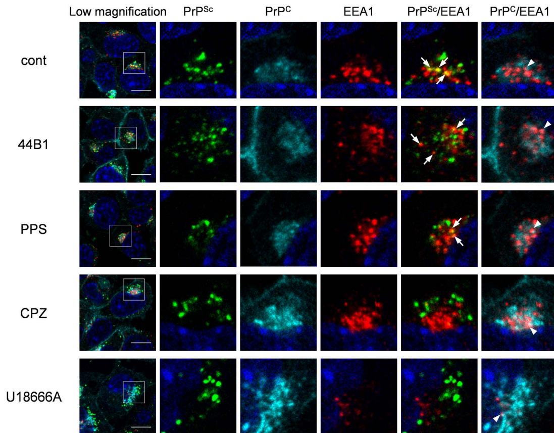
Figure 6. Co-localization of PrP Sc or PrP C with EEA1. ScN2a-3-22L cells were cultured with 7.5 µg/ml mAb 44B1, 10 µg/ml PPS, 10 µM CPZ or 5 µM U18666A or without an anti-prion compound for 6 h. The cells were subjected to direct immunostaining of PrP C and PrP Sc with 31C6-Af555 and rIgG132-EGFP, respectively and subsequently to immunostaining for EEA1 and nuclei. The leftmost column shows a lower-magnification merged image of PrP Sc (green), PrP C (cyan), EEA1 (red), and nuclei (blue). Individual and merged high-magnification images of the boxed regions are shown on the right. Arrows or arrowheads denote representative examples of the co-localization of PrP Sc with EEA1 or PrP C with EEA1, respectively. Scale bars: 10 µm.
