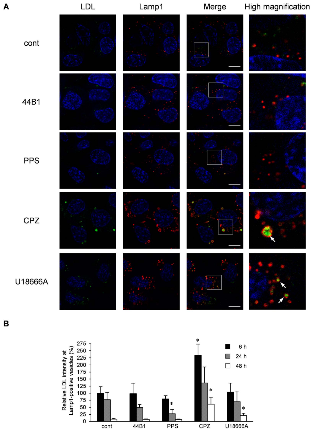
Figure 12. Degradation of LDL in cells treated with anti-prion compounds. ScN2a-3-22L cells were incubated with Alexa Fluor 488-conjugated LDL (4 \mu g/ml) for 6 h. After the incubation, the cells were cultured in the presence or absence of 0.4 \mu g/ml mAb 44B1, 0.1 \mu g/ml PPS, 10 \mu g/ml CPZ, or 5 \mu M U18666A for 6–48 h. The cells were subjected to immunostaining of Lamp1 and staining of the cell nuclei with DAPI. Z-series of the images were acquired at 0.8- \mu m steps from the top to the bottom of the cells in the area. (A) Localization of LDL. The panel shows the representative images of the signals of LDL (green), Lamp1 (red) and nuclei (blue) in cells treated with the indicated anti-prion compound for 24 h. The merged images of LDL and nuclei are shown on the left, those of Lamp1 and nuclei are shown in the middle, and those of LDL, Lamp1, and nuclei are shown on the right. The rightmost column presents the higher-magnification images of the boxed regions in the second right column. Scale bars: 10 \mu m. (B) Intensity of LDL in Lamp1-positive vesicles. The graph shows the values of the fluorescent intensities of LDL in Lamp1-positive vesicles per cell relative to those of LDL in Lamp1-positive vesicles per cell in mock-treated control cells for 6 h. The means and SDs of the value acquired in five view fields are shown. Asterisks indicate a significant difference compared with the control at the same time point (Student's t -test, p < 0.05 ). doi:10.1371/journal.pone.0106516.g012
