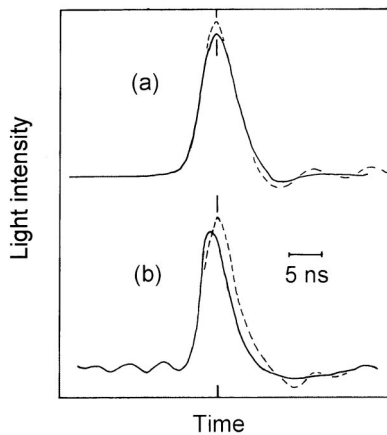
FIG. 1. Typical shape of light pulses before (dashed) and after (solid) transmitting \text{As}_2\text{S}_3 samples; (a) is obtained with light of \hbar\omega = 1.17 eV and I_0 = 430 MW/cm ^2 for a 50 mm long sample and (b) is of 2.16 eV and 82 MW/cm ^2 for a 4.2 mm sample.
