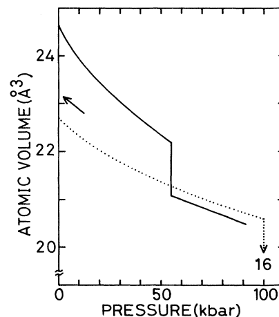
FIG. 4. Atomic volumes of a -Ge (solid line) and c -Ge (dotted line) under pressure. An arrow indicates the state released from 90 kbar.
