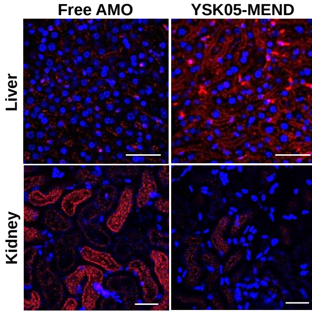
Fig. 3. Histological observations of Cy5-AMO in the liver and kidney. Mice were injected via the tail vein with either free Cy5-AMO or Cy5-AMO encapsulated in the YSK05-MEND (red). Liver and kidney were collected 30 min later. Nuclei in liver and kidney were stained with Hoechst33342 (blue). Images were captured by a CLSM. Scale bars are 50 \mu m.
