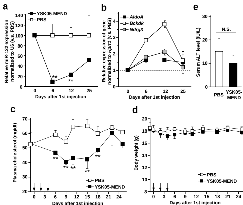
Fig. 5. Long-term observation of the expression level of miR-122 and target genes in the liver and plasma cholesterol levels. Mice were injected via the tail vein with either PBS or AMO122-YSK05-MEND at day 0, 2 and 4. (a, b) The expression of miR-122 (a) and target genes (b) in liver was determined at day 6, 12
