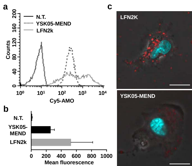
Fig. 2. Cellular uptake and intracellular distribution of Cy5-AMO.
