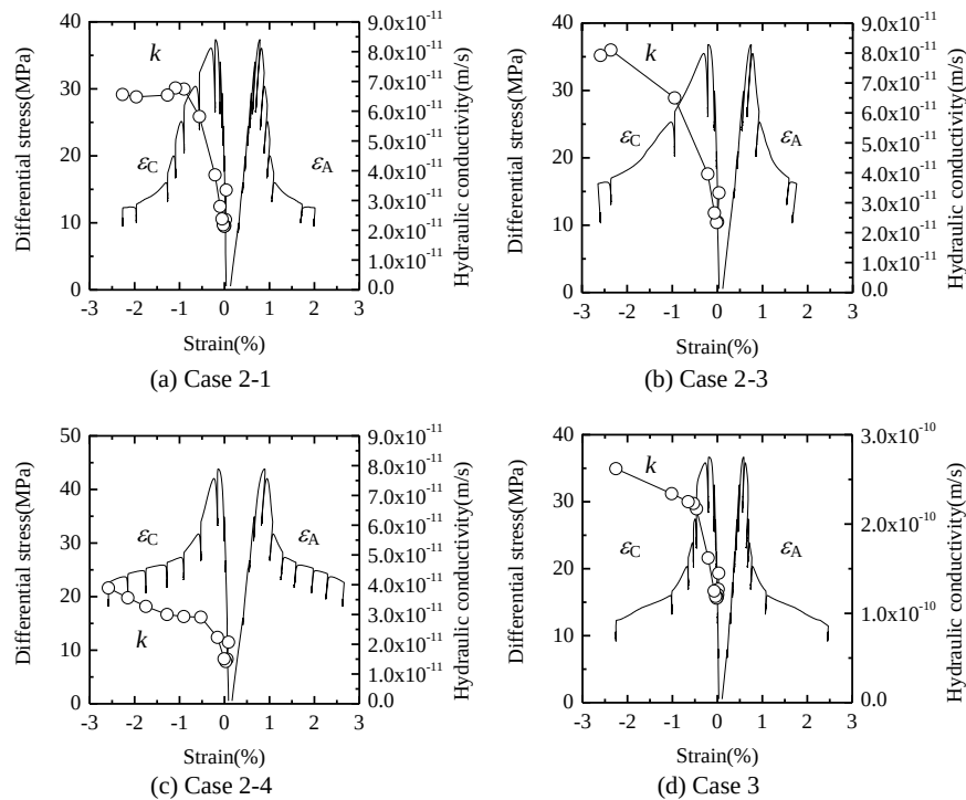
Fig. 2 Examples of stress-strain curves and hydraulic conductivity-circumferential strain curves for Kimachi sandstone. \varepsilon_A , \varepsilon_C , and k denote axial strain, circumferential strain and hydraulic conductivity. Strains were set at zero under atmospheric pressure.
