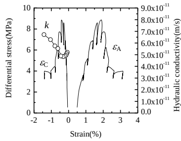
(a) Stress-strain curves and hydraulic conductivity-circumferential strain curve.
