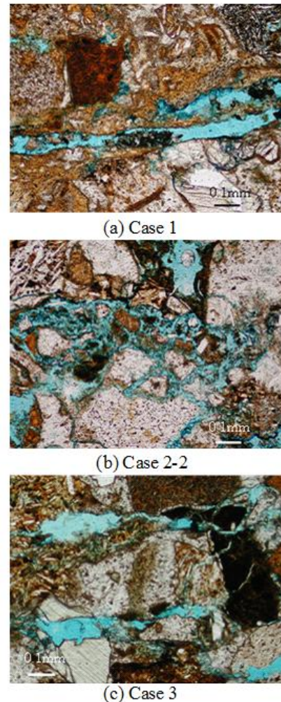
Fig. 5 Examples of thin section micrographs of Kimachi sandstone. Rupture plane is aligned parallel to horizontal.
