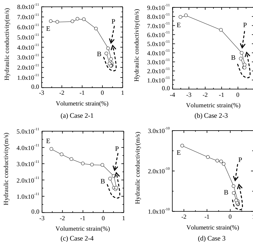
Fig. 3 Volumetric strain and hydraulic conductivity in compression 1 for Kimachi sandstone. B, E and P denote the beginning and the end of compression 1 and peak load point, respectively. The arrows denote the progress of tests.
