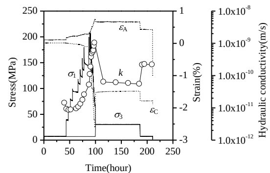
(c) Variation in strains and hydraulic conductivity due to loading.
