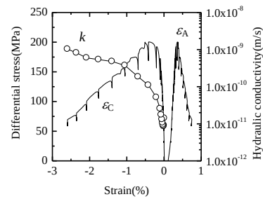
(a) Stress-strain curves and hydraulic conductivity-circumferential strain curve.
