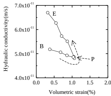
(b) Hydraulic conductivity-volumetric strain curve.
