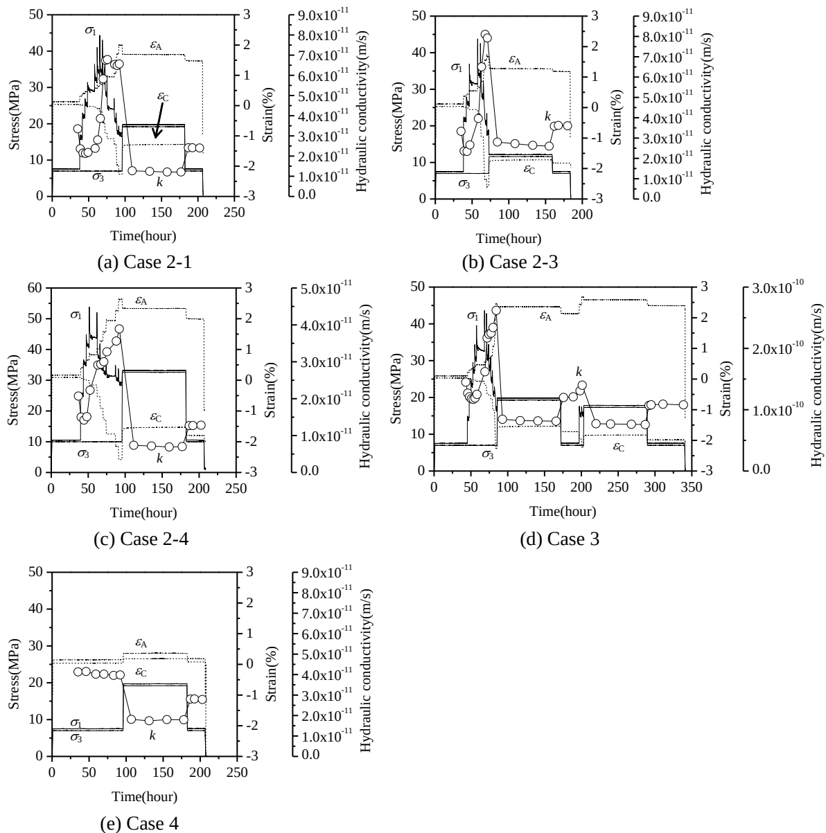
Fig. 4 Variation in strains and hydraulic conductivity during loading of Kimachi sandstone.
