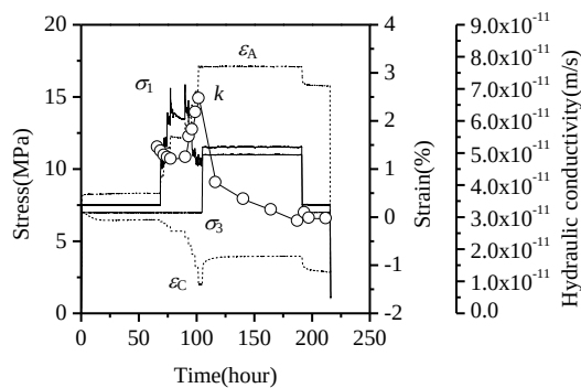
(c) Variation in strains and hydraulic conductivity due to loading.
