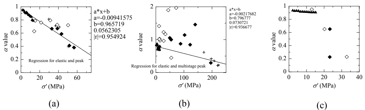
Figure. 11 Effective normal stress vs \alpha for a) Kimachi Sandstone b) Inada Granite and c) Shikotsu Welded Tuff
