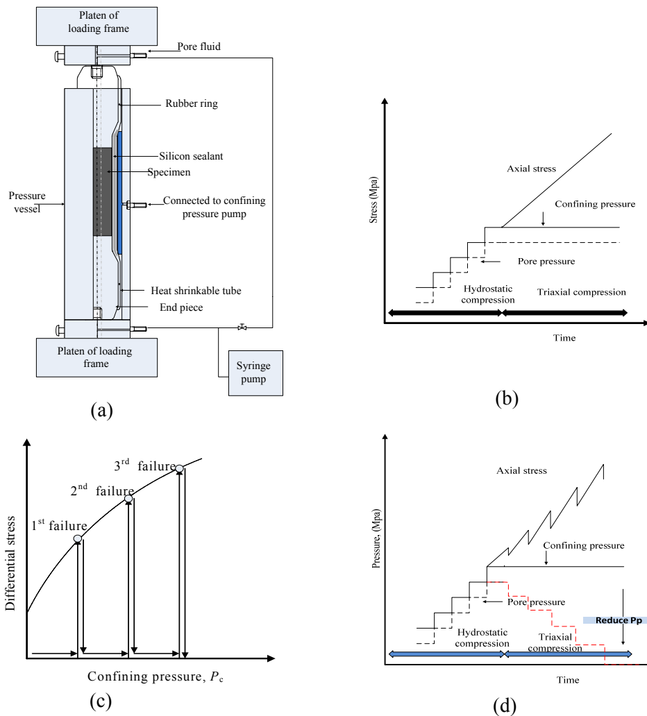
Figure 2. Experimental setup and stress paths of single and multi-stage triaxial tests. a) Experimental setup with ultra compact triaxial cell. b) Procedure to reach the target confining pressure, pore pressure and compression phase of single stage triaxial test. c) Stress paths of multi-stage triaxial test with zero pore pressure. d) Stress paths of multi-stage triaxial test with pore pressure.
