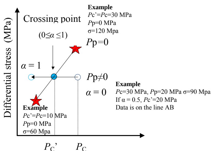
Figure 1. Evaluation of \alpha by the Modified Failure Envelope Method.
