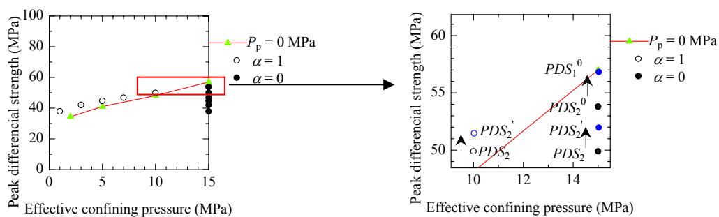
Figure 3. Correction for peak differential stress for Kimachi Sandstone.
