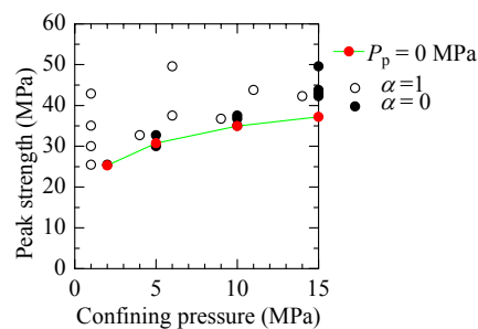
Figure 10 Peak differential stress vs effective confining pressure when \alpha = 0 and \alpha = 1 for Shikotsu Welded Tuff.
