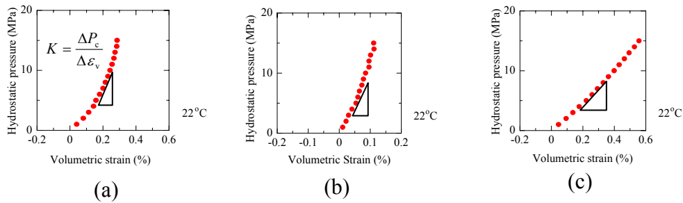
Figure 5. Stress-strain curve in hydrostatic compression test for P_p=0 a) For Kimachi Sandstone b) For Inada Granite c) For Shikotsu Welded Tuff
