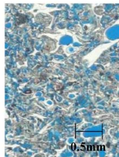
Figure 9 Blue resin-impregnated thin-section of Shikotsu Welded Tuff.
