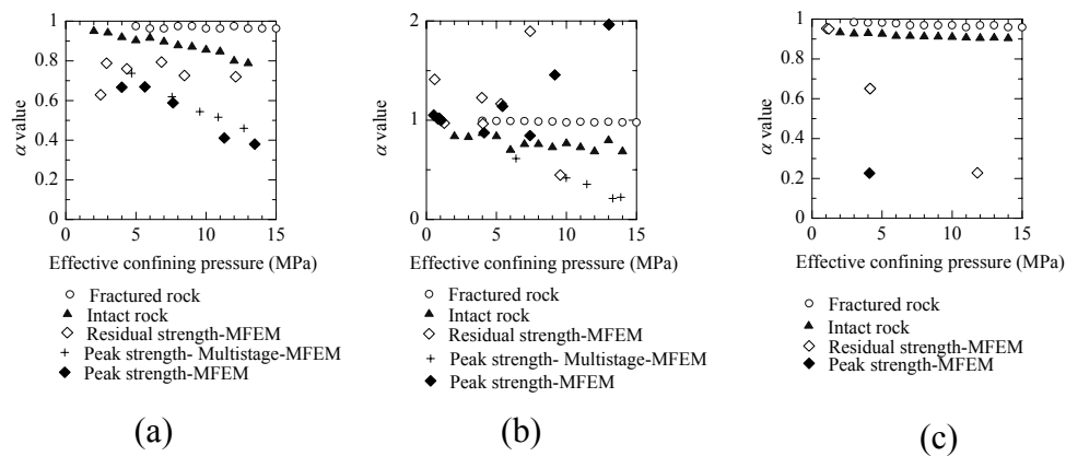
Figure 8. Summary of effective stress coefficients for a) Kimachi Sandstone b) Inada Granite and c) Shikotsu Welded Tuff
