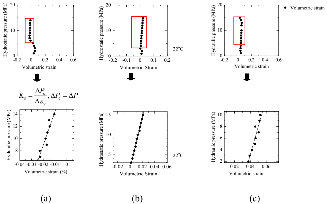
Figure 6. Stress-strain curve in hydrostatic compression test with pore pressure: \Delta P_c = \Delta P_p . a) For Kimachi Sandstone b) For Inada Granite c) For Shikotsu Welded Tuff
