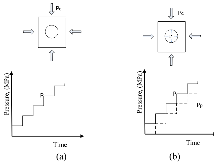
Figure 4. Stress paths of hydrostatic compression tests a) with zero pore pressure: P_p = 0 . b) with non-zero pore pressure: \Delta P_c = \Delta P_p .
