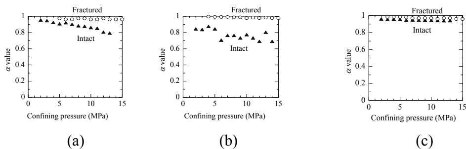
Figure 7. Biot's effective stress coefficient by hydrostatic test for intact and fractured rock specimens of a) Kimachi Sandstone b) Inada Granite and c) Shikotsu Welded Tuff
