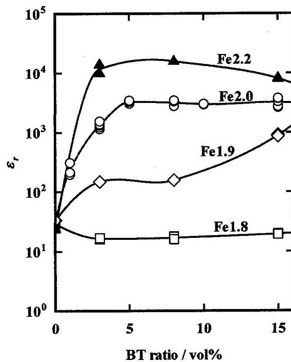
Fig.1 \epsilon_r changes with BT ratio for composites with different Fe contents.
