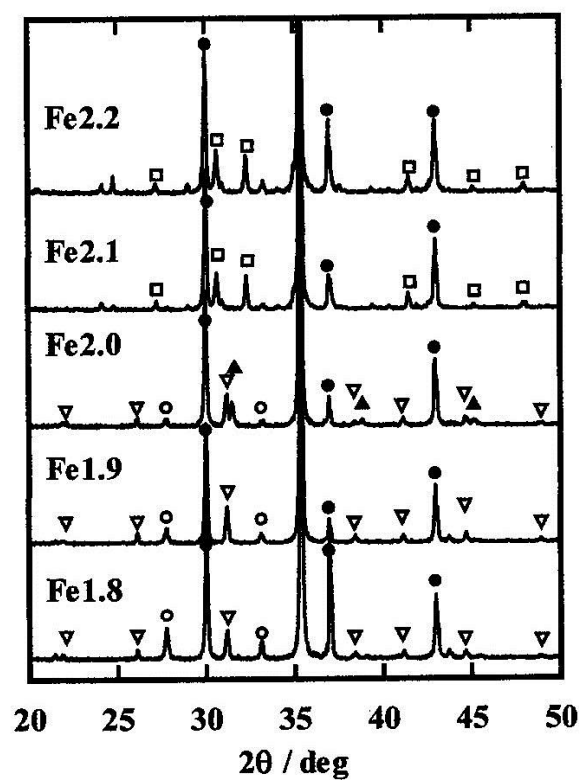
Fig.2 XRD patterns of the 8BT composites with different Fe contents. (●NiZn ferrite, ▲t-BaTiO 3 , ○BaFe 2 O 4 ss, ▽h-BaTiO 3 ss, □Ba 2 Fe 6 O 11 ss)
