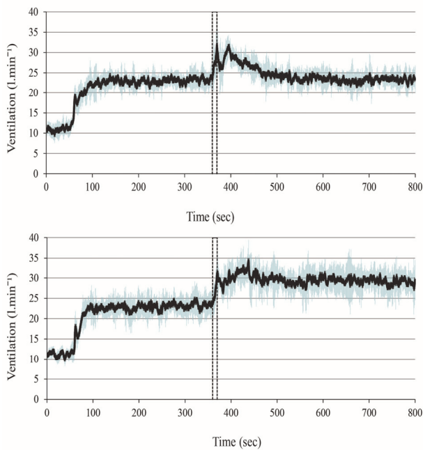
Fig. 2. Changes in ventilation ( \dot{V}_E ) during 200 watts impulse-like exercise and recovery from 200 watts impulse-like exercise with work load of 25 watts in test one ( upper panel ) and work load of 50 watts in test two ( lower panel ). The vertical dashed line bar indicates exercise time. Data presented are means \pm SD.
