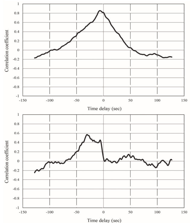
Fig. 3. Cross correlation between ventilation ( \dot{V}_E ) and predicted arterial carbon dioxide partial pressure ( \text{PaCO}_{2\text{pre}} ) during recovery from 200 watts impulse-like exercise in test one ( upper panel ) with work load of 25 watts during recovery and in test two ( lower panel ) with work load of 50 watts during recovery.
