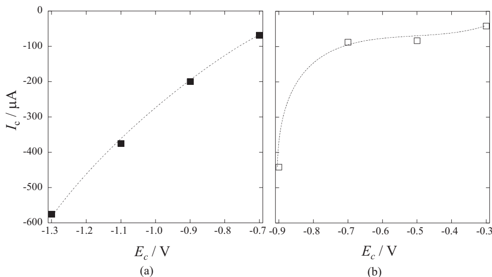
Figure 6. Potential vs. cathodic current obtained 600 s after starting the HER in (a) 0.36 M KOH and (b) 0.5 M \text{H}_2\text{SO}_4 droplets.
