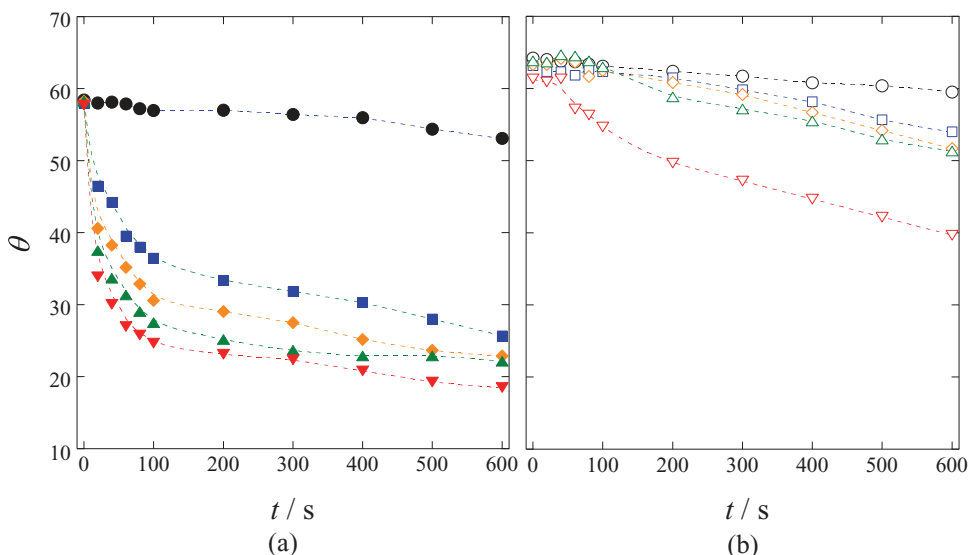
Figure 5. Time-dependent changes in the contact angle of (a) 0.36 M KOH and (b) 0.5 M \text{H}_2\text{SO}_4 droplets during the HER obtained at several electrode potentials. (●: OCP, ■: -0.7 V, ◆: -0.9 V, ▲: -1.1 V, ▼: -1.3 V in (a)) (○: OCP, □: -0.3 V, ◇: -0.5 V, △: -0.7 V, ▽: -0.9 V in (b)).
