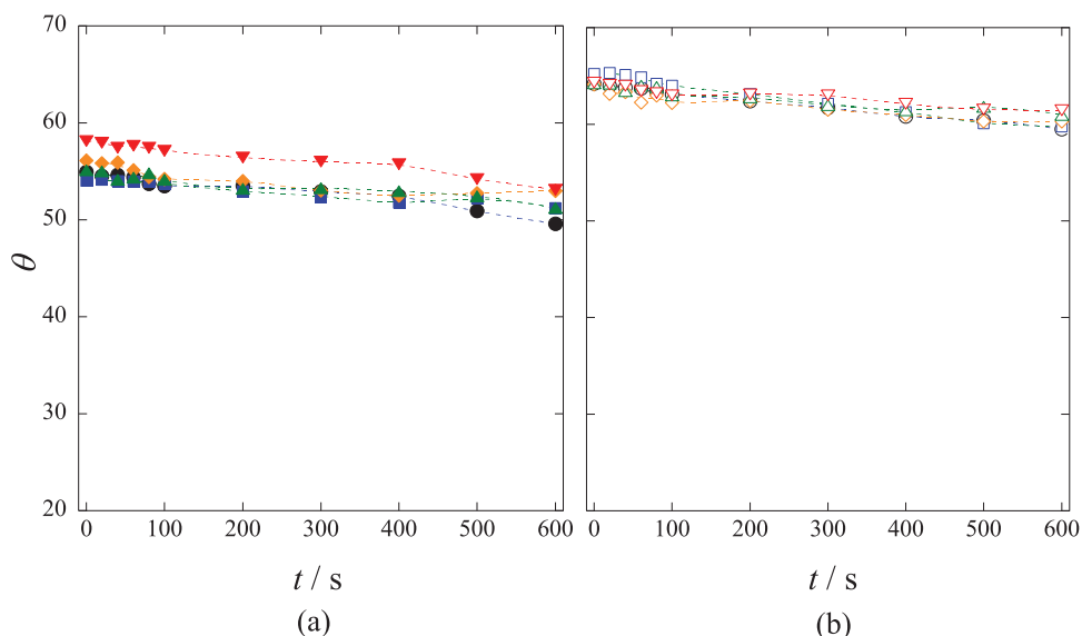
Figure 3. Time-dependent changes in the contact angle of (a) 0.36 M KOH and (b) 0.5 M \text{H}_2\text{SO}_4 droplets during the HOR obtained at several electrode potentials. (●): OCP, ■: -0.2 V, ◆: 0 V, ▲: 0.2 V, ▼: 0.4 V in (a)) (○: OCP, □: 0.1 V, ◇: 0.2 V, △: 0.3 V, ▽: 0.4 V in (b)).
