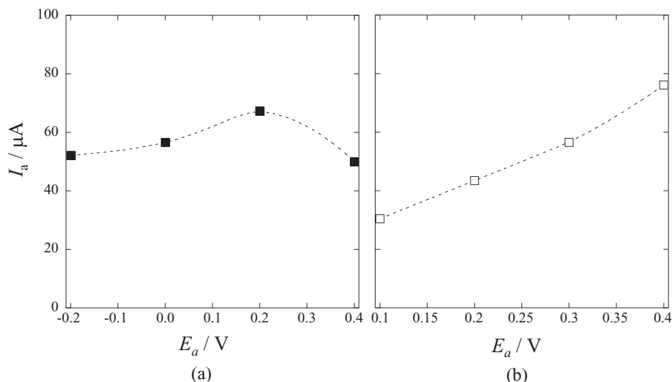
Figure 4. Potential vs. anodic current obtained 600 s after starting the HOR in (a) 0.36 M KOH and (b) 0.5 M \text{H}_2\text{SO}_4 droplets.
