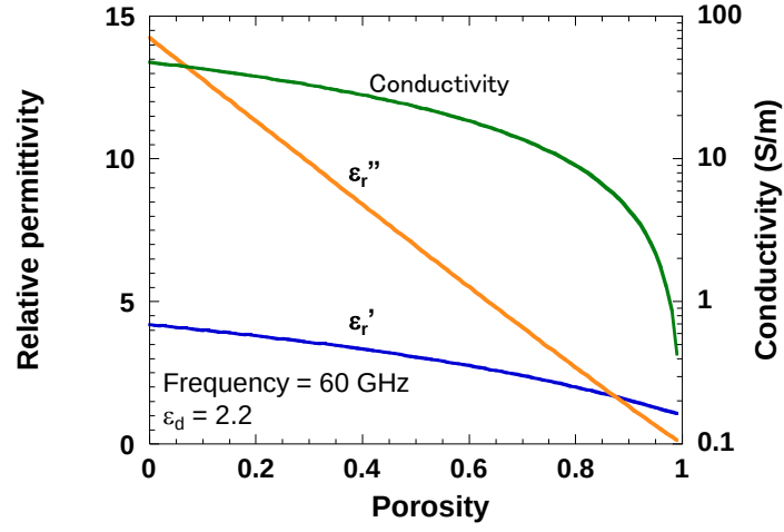
Fig. 3 Calculated dependences of real and imaginary parts of dielectric constant \epsilon_{eff} and conductivity on porosity p for a CNT composite with v=3.5\% .
