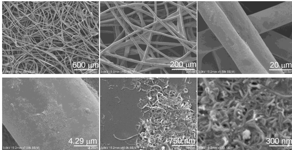
Fig. 5 SEM images of MWCNT-coated nonwoven fabric c .
