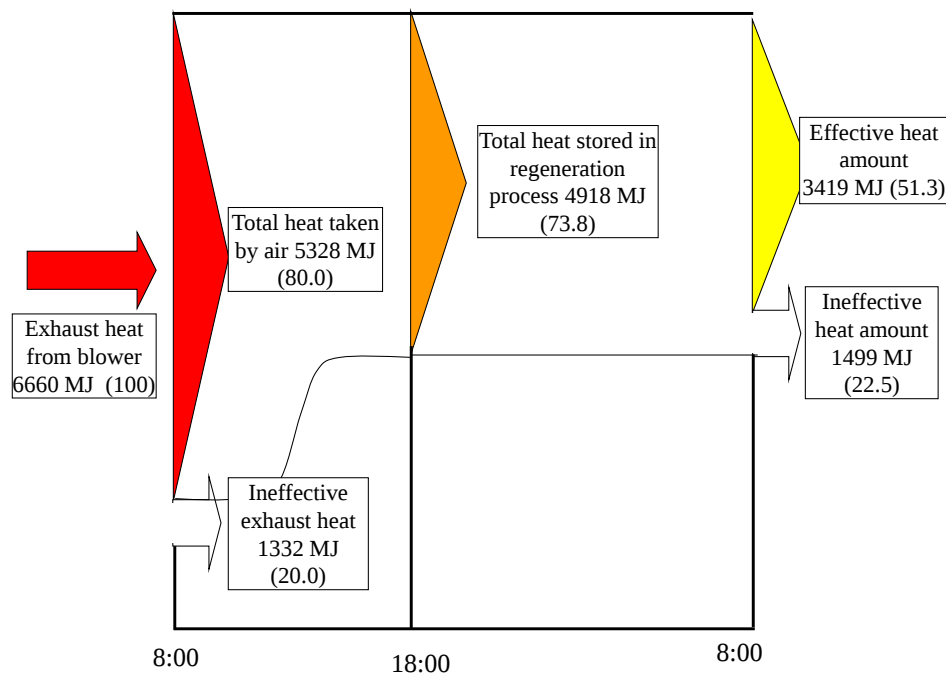
Fig. 20 Energy flow chart of the improved paint drying system incorporated with the open thermal energy storage unit
