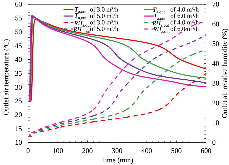
Fig. 10 Outlet air relative humidity and outlet air temperature change with time of different humid air flow rates
