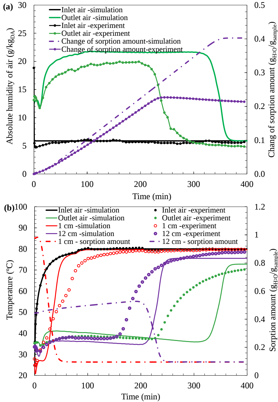
Fig. 5 (a) Comparison of inlet/ outlet air absolute humidity and change of the sorption amount during desorption process; (b) comparison of inlet/outlet air temperature and temperature of the WSS + 22.4 wt% CaCl 2 in heat desorption process (hot air flow rate: 3.8 m 3 /h; regeneration temperature: 80°C)
