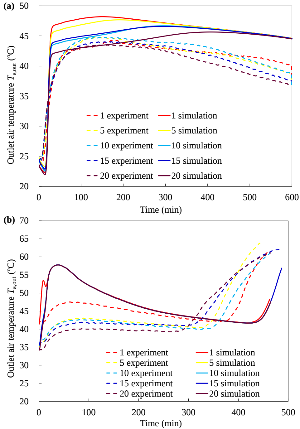
Fig. 7 (a) Comparison of the outlet air temperature during the heat release process; (b) comparison of the outlet temperature during the regeneration process of the WSS + 22.4 wt% \text{CaCl}_2 (humid air flow rate: 2.0 \text{ m}^3/\text{h} ; hot air flow rate: 2.8 \text{ m}^3/\text{h} ; regeneration temperature: 80^\circ\text{C} )
