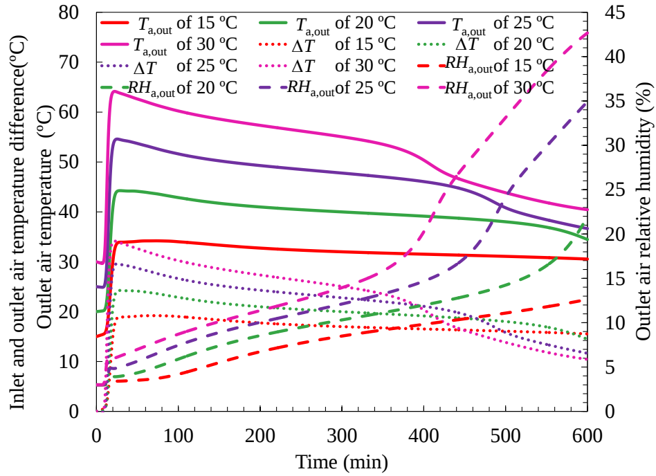
Fig. 8 Outlet air relative humidity, outlet air temperature and outlet and inlet air temperature difference change with time of different inlet air temperatures
