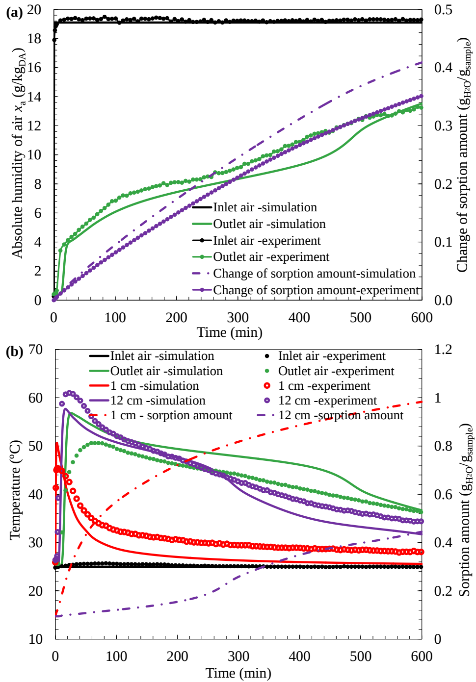
Fig. 3 (a) Comparison of inlet/ outlet air absolute humidity and change of the sorption amount during sorption process; (b) comparison of inlet/outlet air temperature and temperature of the WSS + 22.4 wt% \text{CaCl}_2 in heat release process (humid air flow rate: 3.0 \text{ m}^3/\text{h} ; regeneration temperature: 80^{\circ}\text{C} )
