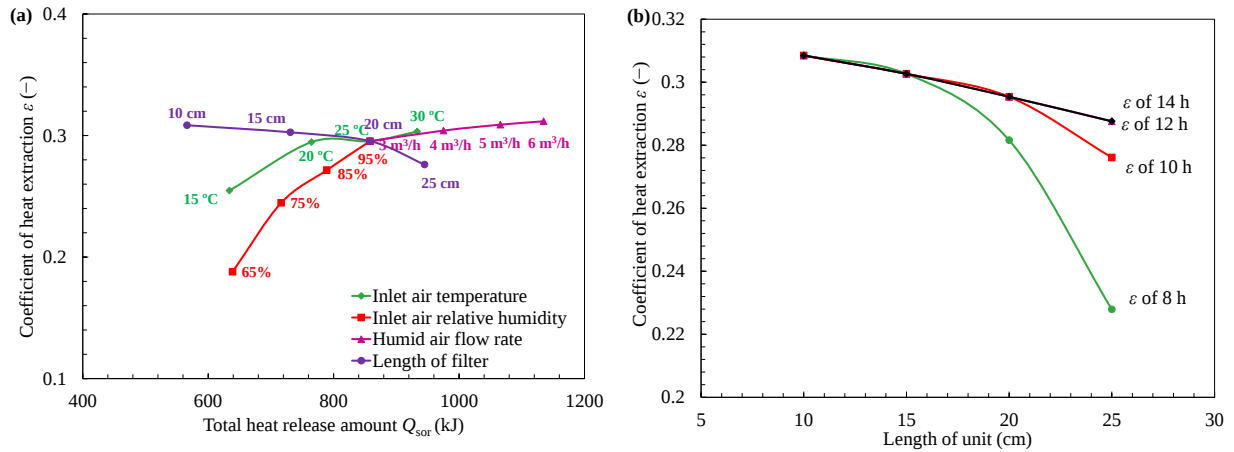
Fig. 15 (a) Effect of each parameter on total heat release amount and coefficient of heat extraction during heat release process; (b) effect of heat release duration on coefficient of heat extraction
