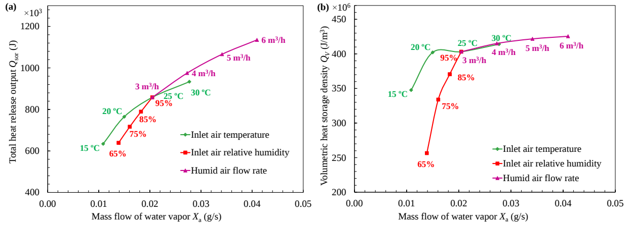
Fig. 13 (a) Effect of absolute water vapor content on total heat release amount; (b) effect of absolute water vapor content on volumetric heat storage density
