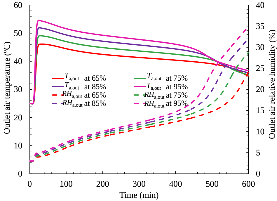
Fig. 9 Outlet air relative humidity and outlet air temperature change with time of different inlet air relative humidities
