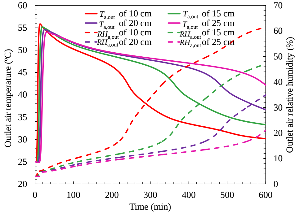
Fig. 12 Outlet air relative humidity and outlet air temperature change with time of different length of the thermal energy storage units
