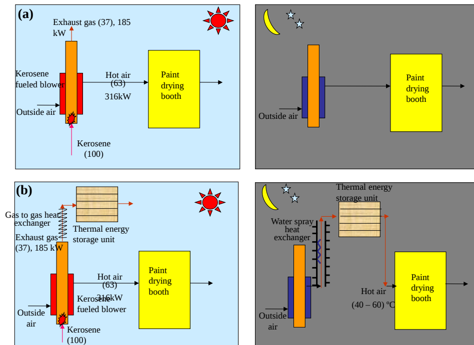
Fig. 17 (a) Previous paint drying system; (b) improved system incorporated with the
