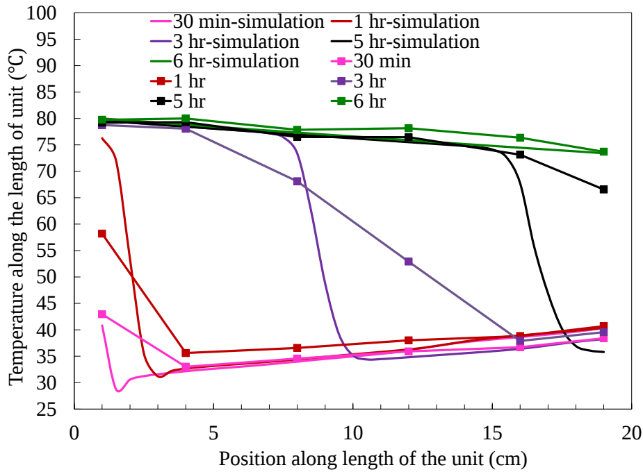
Fig. 6 Temperature profile of the WSS + 22.4 wt% \text{CaCl}_2 in heat storage process (hot air flow rate: 3.8 \text{ m}^3/\text{h} ; regeneration temperature: 80^\circ\text{C} )
