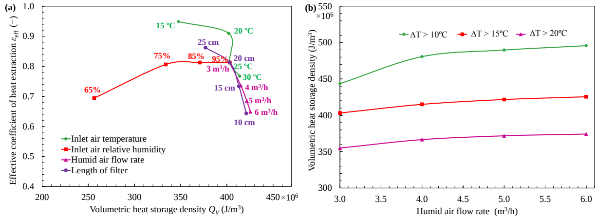
Fig. 14 (a) Effect of each parameter on volumetric heat storage density and effective coefficient of heat extraction during heat release process; (b) effect of inlet and outlet air temperature difference on volumetric heat storage density; (c) effect of heat release duration on volumetric heat storage density
