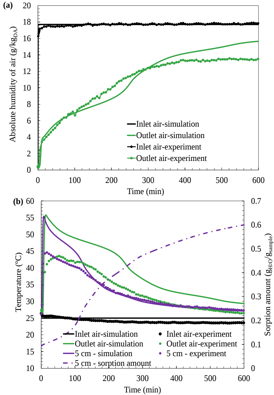
Fig. 11 (a) Comparison of inlet and outlet air absolute humidity; (b) comparison of inlet/outlet air temperature and temperature of the WSS + 22.4 wt% \text{CaCl}_2 with a length of 10 cm in heat release process (humid air flow rate: 3.0 \text{ m}^3/\text{h} ; regeneration temperature: 80^{\circ}\text{C} )
