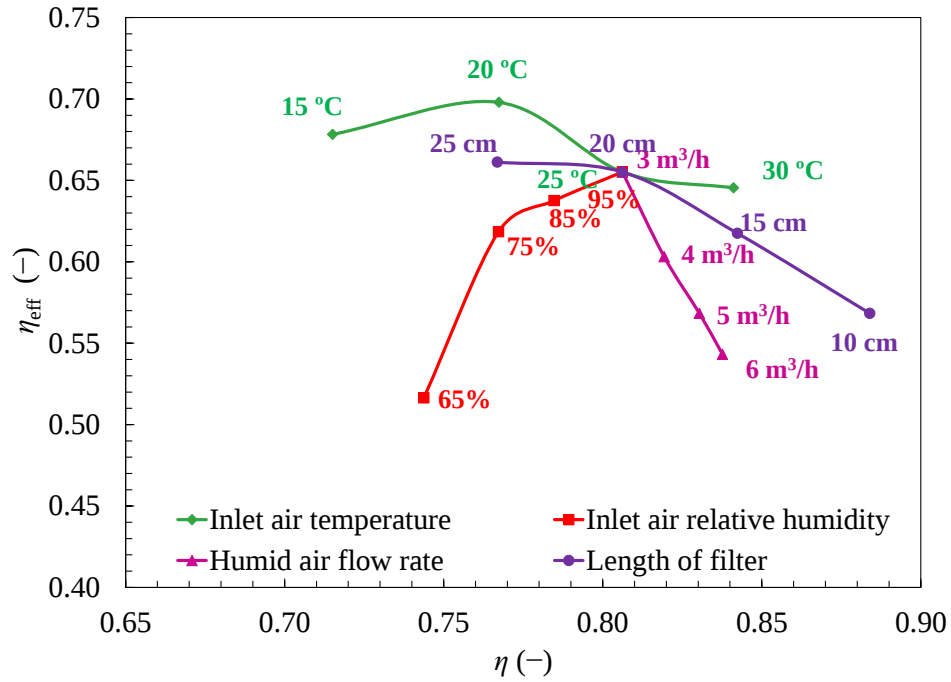
Fig. 16 Effect of each parameter on \eta and \eta_{eff} of the open sorption thermal energy storage system
