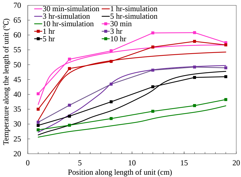
Fig. 4 Temperature profile of the WSS + 22.4 wt% \text{CaCl}_2 in heat release process (humid air flow rate: 3.0 \text{ m}^3/\text{h} ; regeneration temperature: 80^\circ\text{C} )
