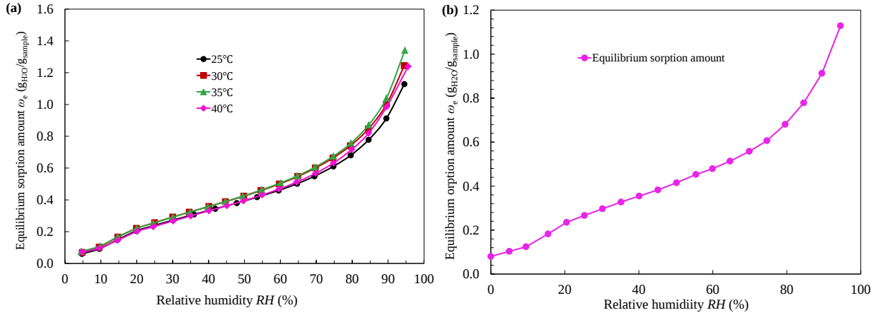
Fig. 2 (a) Equilibrium sorption amount at different temperatures for the WSS +22.4 CaCl 2 ; (b) equilibrium sorption fitting lines used in simulation for the WSS +22.4 CaCl 2
