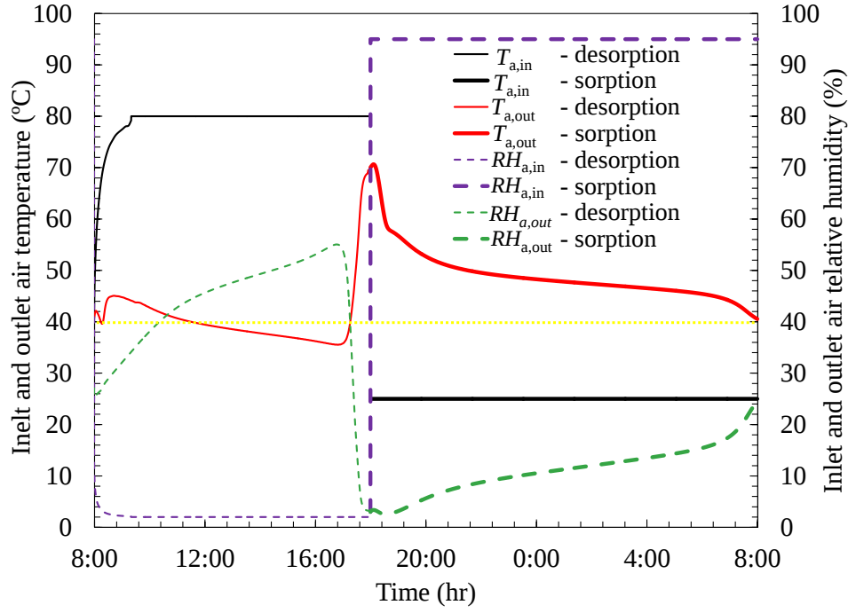
Fig. 18 Simulated outlet air relative humidity and outlet air temperature during the sorption and desorption processes, respectively
