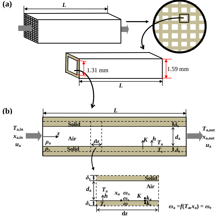
Fig. 1 The one-dimensional transient model illustration
