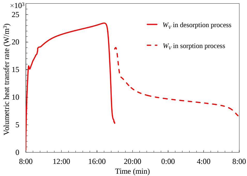
Fig. 19 Volumetric heat transfer rate of the open thermal energy storage unit
