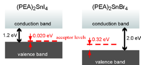
Figure 5. Schematic representation of the calculated band structures of (\text{PEA})_2\text{SnI}_4 and (\text{PEA})_2\text{SnBr}_4 and acceptor levels formed in the band gap..
