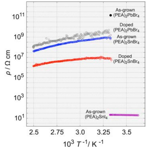
Figure 4. Temperature dependence of resistivity of the as-grown and doped (PEA) 2 SnBr 4 and (PEA) 2 PbBr 4 crystals. For comparison, the reported data 3a of the as-grown (PEA) 2 SnI 4 crystals are also shown.
