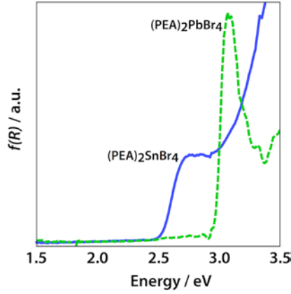
Figure 2. Diffuse reflectance spectra of (PEA) 2 SnBr 4 and (PEA) 2 PbBr 4 . The reflectivity was converted to the Kubelka-Munk function, f(R) , corresponding to the absorption.
