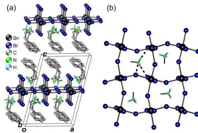
Figure 1. (a) Perspective view of the unit cell and (b) organic–inorganic interface of (\text{PEA})_2\text{SnBr}_4 viewed along the c -axis showing H-bonding between \text{NH}_3 and \text{SnBr}_6 octahedra. Crystal data are as follows: triclinic P1 ; a = 11.526(1) , b = 11.634(1) , c = 17.510(1) Å; \alpha = 80.449(2) , \beta = 74.634(2) , \gamma = 89.953(2)^\circ ; V = 2230.5(3) Å 3 ; and Z = 4 .
