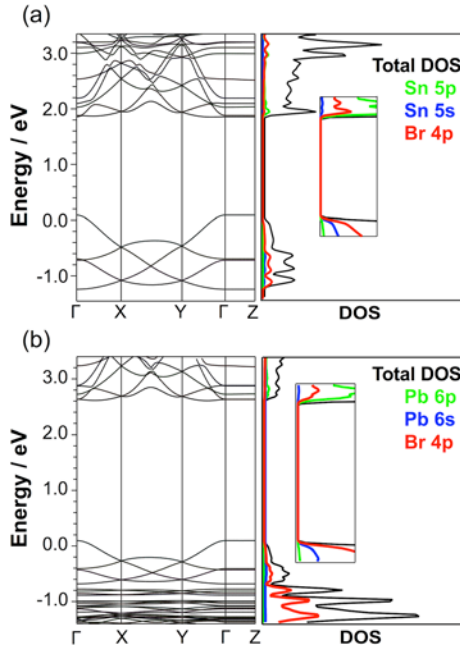
Figure 3. Calculated band dispersion (left) and density of states, (DOS, right) (inset shows magnification of the valence band and conduction band edge) of (a) (PEA) 2 SnBr 4 and (b) (PEA) 2 PbBr 4 .
