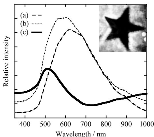
Figure 2. Reflected UV–Vis absorption spectra of the (a) OH-terminated alkylamine monolayer and (b) pyrene-labeled, \text{NH}_2 -terminated alkylamine monolayer on a HOPG surface. (c) Reflected UV–Vis absorption difference spectrum of (a) and (b). An adapted incandescent light was used as the irradiation source. Inset is the photograph of the pyrene-labeled, \text{NH}_2 -terminated alkylamine monolayer (bright areas) and OH-terminated alkylamine monolayer (dark areas) on a HOPG surface. The image was taken under ultraviolet light at a wavelength of 254 nm.
