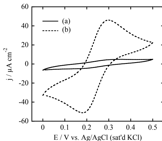
Figure 1. Cyclic voltammograms of COOH-terminated alkylamine modified HOPG electrode (a) before and (b) after the deep UV light irradiation in 200 μM K 4 [Fe(CN) 6 ] + 0.1 M KCl solution at the sweep rate of 0.02 V s -1 .
