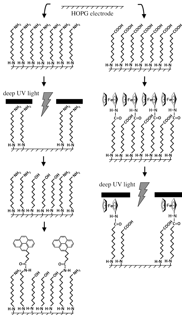
Scheme 1. Procedure for the preparation of hybrid functional group-terminated alkylamine-modified HOPG electrodes. Left side: pyrene-labeled \text{NH}_2 -terminated alkylamine monolayer and OH-terminated alkylamine monolayer; right side: ferrocene-labeled COOH-terminated alkylamine monolayer and unmodified.
