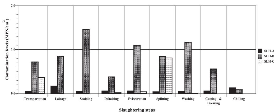
Fig. 4. Contamination levels (MPN/cm 2 ) of Salmonella spp. isolated from swabs of pig skins and carcasses taken at each step of the slaughtering process.
