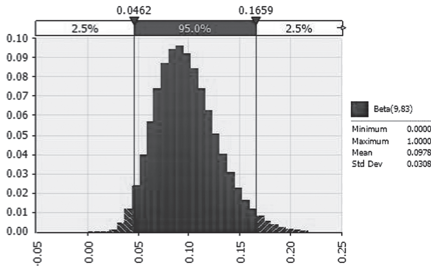
Fig. 5. Risk simulation of Salmonella spp. in pork products at the final stage of slaughtering level. X-axis; Salmonella 's prevalence. Y-axis; frequency of Salmonella samples.
