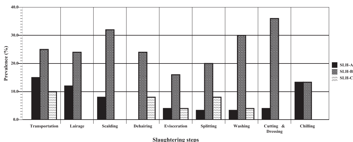
Fig. 3. Prevalence (%) of Salmonella spp. isolated from swabs of pig skins and carcasses taken at each step of the slaughtering process.
