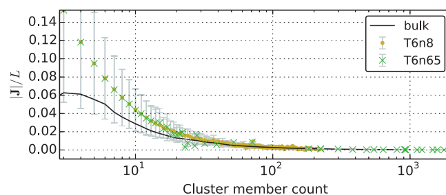
FIG. 7. This ratio (see definitions (8) and (9)) is an indicator of the extent to which the members of a cluster rotate in unison. Unity corresponds to harmonious rotation, while zero to dissonance. The cluster spin damps rapidly as they grow. While we plot this quantity for only two runs here, it exhibits similar behaviour for all runs. For comparison, this ratio was calculated in the bulk to determine the noise level, as this signal is expected to average to zero for the bulk. Finite-size effects however contribute an intrinsic noise to this quantity. We estimate this by randomly centring spheres in the bulk, and calculating the ratio for the enclosed atoms.
