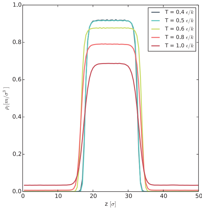
FIG. 18. Density profiles from rectangular box bulk simulations, detailed in Appendix B.
