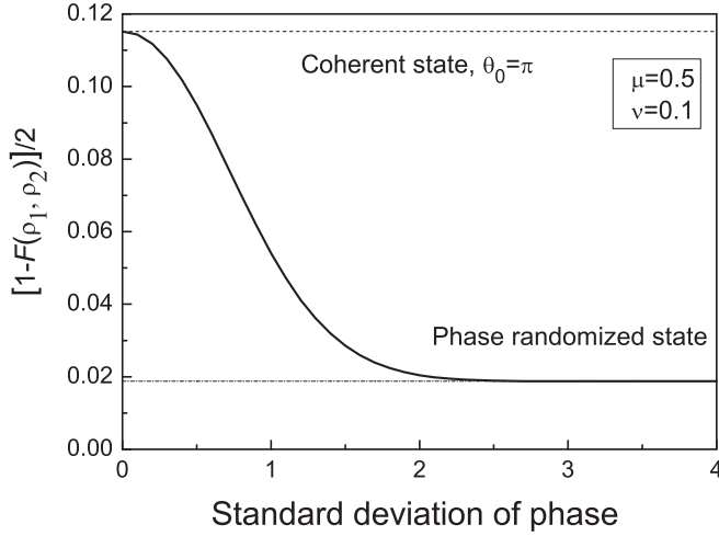
FIG. 3. Distinguishability [1 - F(\rho_1, \rho_2)]/2 between the signal and decoy states as a function of the standard deviation of phase. Calculation was done for the partially phase randomized states of average photon number 0.5 (signal) and 0.1 (decoy). Solid line represents the calculated fidelity for \theta_0 = \pi . Dashed-dot line stands for the distinguishability between the completely phase randomized states, and dashed line between coherent states with \theta_0 = \pi .
