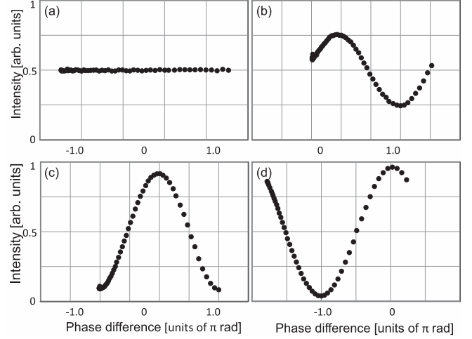
FIG. 5. Interference fringes for several values of the normalized minimum excitation: (a) \Lambda = -1.6 , (b) \Lambda = 0.074 , (c) \Lambda = 0.49 , and (d) \Lambda = 2.6 .
