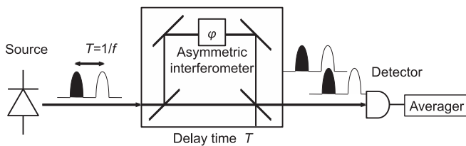
FIG. 1. A schematic illustration of a measurement apparatus for the phase correlation between the adjacent pulses. The delay time of the asymmetric interferometer is adjusted to the pulse period. The phase difference \varphi between the paths can be modulated.
