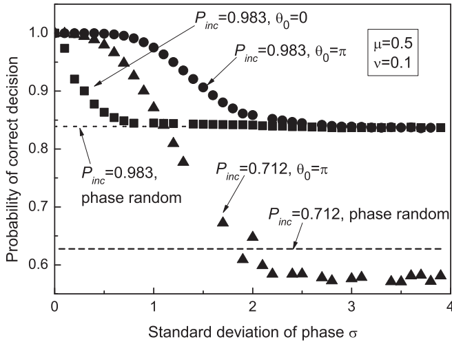
FIG. 8. Probability of correct decision in the optimal discrimination of the signal and decoy states as a function of the standard deviation of phase. The state discrimination was done for the partially phase-randomized states of average photon number 0.5 and 0.1. Inconclusive results are allowed in the state discrimination. Squares represent P_{\text{inc}} = 0.983 , \theta_0 = 0 , circles P_{\text{inc}} = 0.983 , \theta_0 = \pi , and triangles P_{\text{inc}} = 0.712 , \theta_0 = \pi . Dotted line and dashed line refer to the probability of correct decision on the phase-randomized states under the conditions of P_{\text{inc}} = 0.983 and P_{\text{inc}} = 0.712 , respectively.
