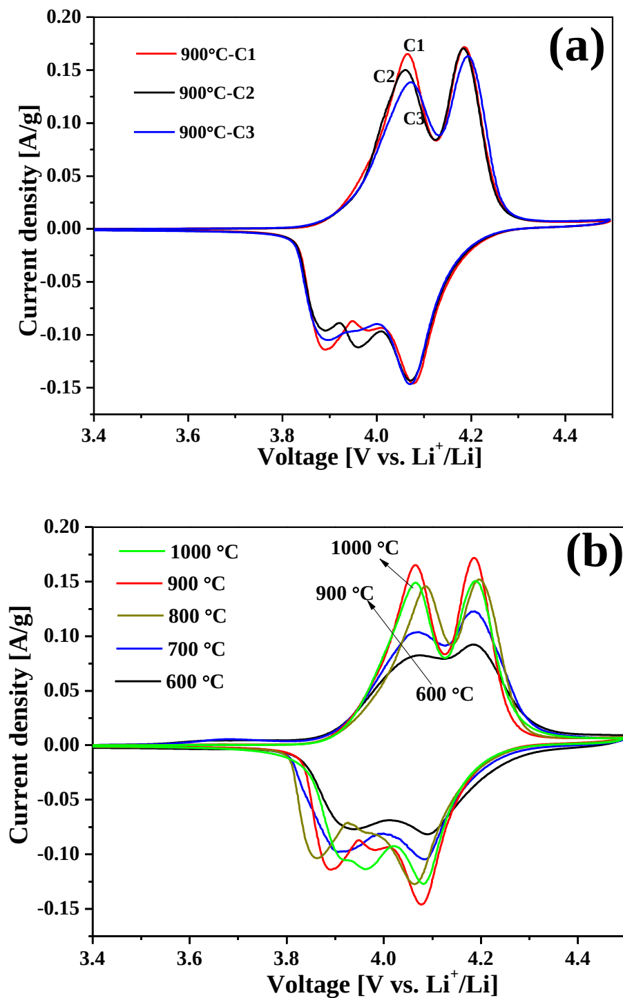
Figure 8. CV curves of the electrodes made with \text{LiMn}_2\text{O}_4 . (a) The initial three cycles of the CV curves of the sample calcined at 900 °C. (b) The first cycle of CV curves of the \text{LiMn}_2\text{O}_4 samples calcined at different temperatures. The scan rate was 0.1 \text{ mVs}^{-1} .
