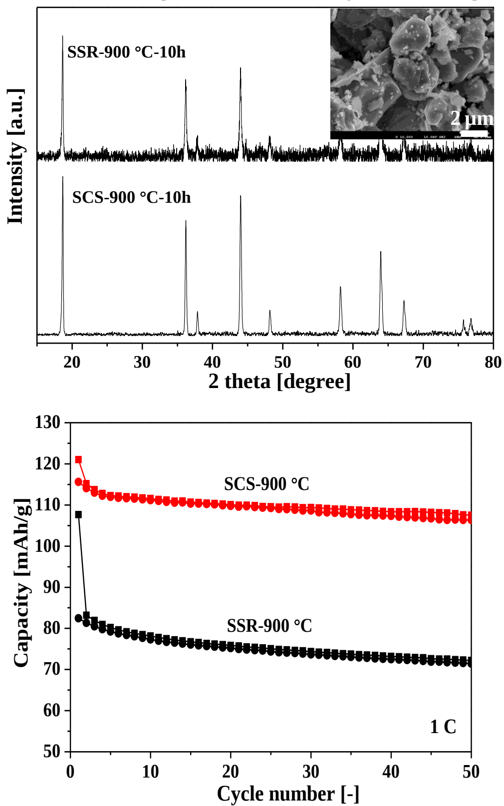
Figure 9. XRD patterns and cycling performance of the SSRed \text{LiMn}_2\text{O}_4 , in comparison to those of the SCSed sample. Inset shows the SEM image of the SSRed sample.
