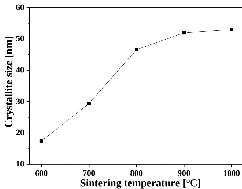
Figure 4. Crystallite sizes (calculated by Scherrer's equation) of the SCSed samples calcined at different temperatures.
