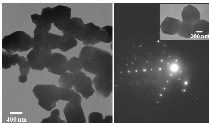
Figure 6. Typical TEM images and selected area diffraction pattern of the calcined sample at 900 °C.
