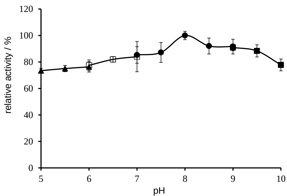
Figure S10. Effects of pH on PaxD activity. The assay was conducted at a pH range from 5.0 to 10, with 50 mM citrate (solid triangles), 50 mM MES (open squares), 50 mM Tris-HCl (solid circles), and 50 mM borate-NaOH buffer (solid squares). The assay mixture and condition were the same as those described in Figure S9.
