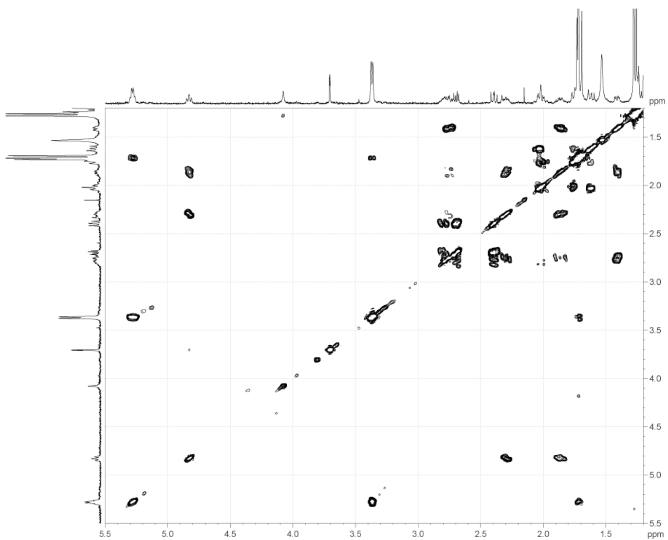
Figure S5. H-H COSY of 21,22-diprenylated paxilline (2).
