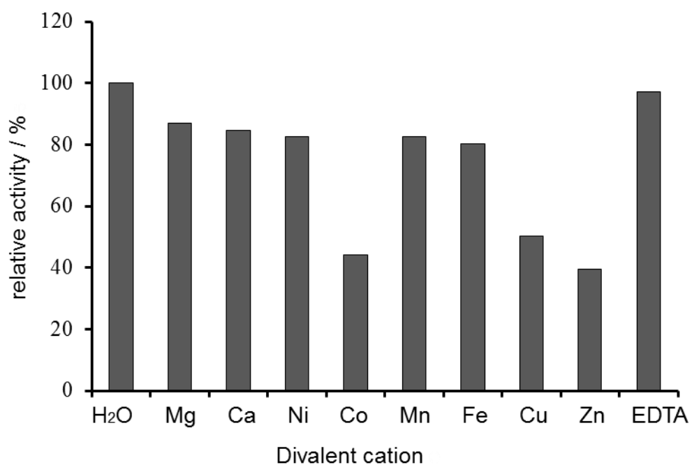
Figure S11. Effects of metal ions on PaxD activity. Each of divalent ions (5 mM), or 5 mM EDTA was added to the reaction mixture. The assay mixture and condition were the same as those described in Figure S9.
