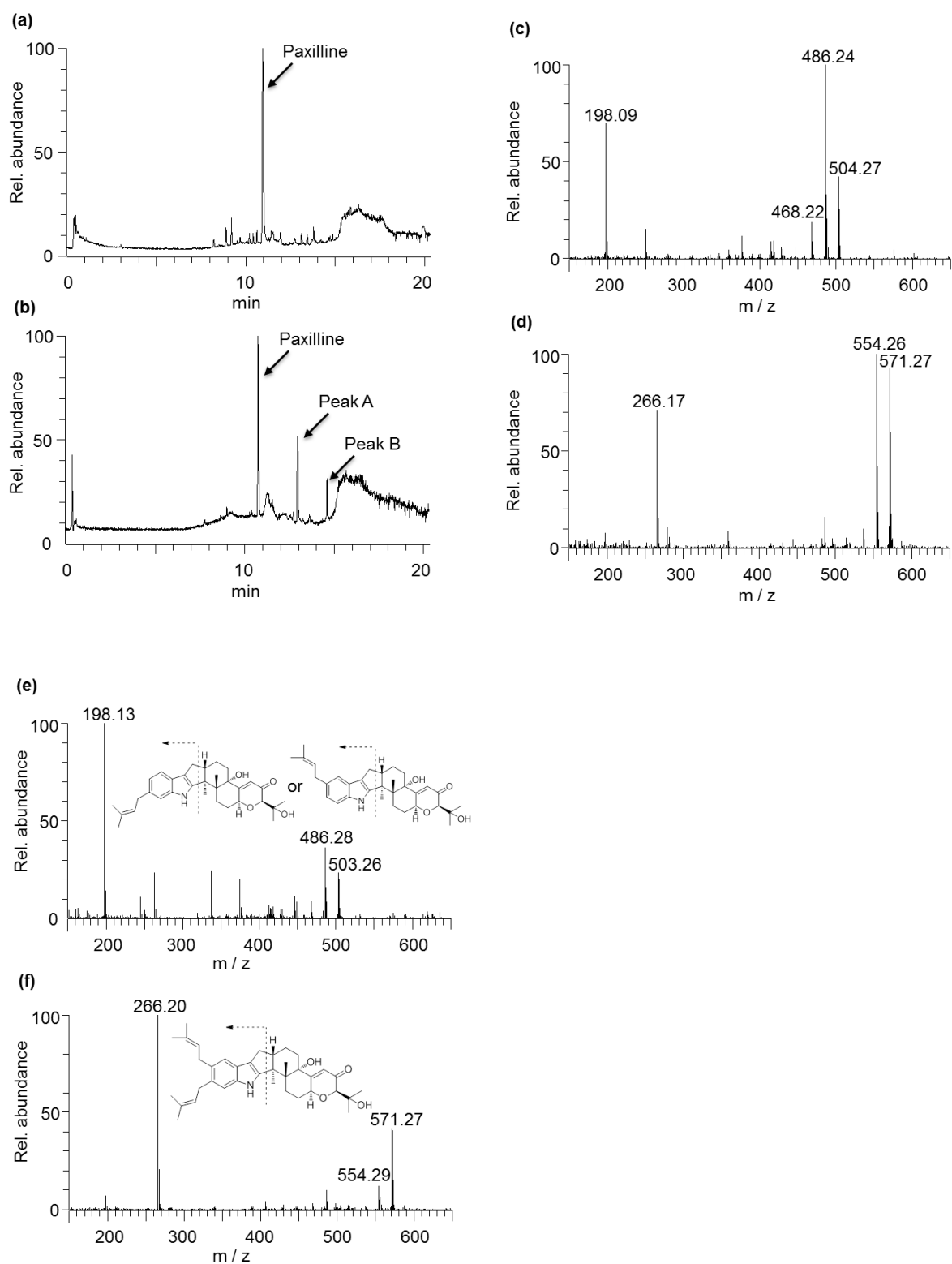
Figure S2. LC/ESI-MS analysis of the prenylated paxillines. Total ion chromatogram of products formed by in vitro assay without (a) and with (b) PaxD and mass spectra of peak A (c) and peak B (d) are shown. Mass spectra obtained from selected ion chromatograms of products accumulated in culture broth are also shown (e and f) together with probable fragment principles.
