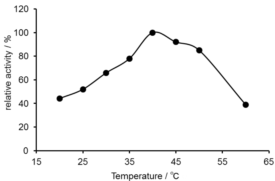
Figure S9. Effects of temperature on PaxD activity. The assay was conducted at a temperature range from 20 to 60°C. The assay mixture contained, in a final volume of 100 \mu L, 0.25 mM of paxilline, 0.25 mM of DMAPP, 50 mM Tris-HCl (pH 8.0), and 0.2 \mu g of PaxD. This mixture was incubated at each temperature for 10 min.
