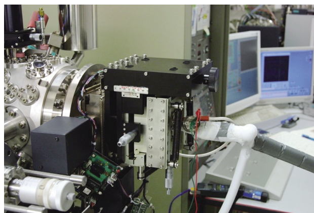
Fig. 3. Cryo-sample-stage installed on Cameca ims-1270. The temperature of the sample stage is cooled by liquid nitrogen, which is supplied by the frost-covered (white) tube.
