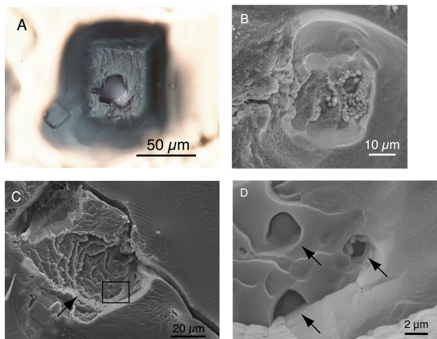
Fig. 7. Representative sputtering crater after isotope analysis. (A) Photomicrograph of the surface of the synthetic halite standard. A negative crystal of a fluid inclusion is observed in the crater bottom. The fluid has been evaporated during takeout from sample chamber of SIMS. (B) Secondary electron image of the negative crystal surface of (A). Small halite grains precipitated during evaporation of the fluid inclusion fluid are observed on the bottom. (C) Secondary electron image of the surface of a Monahans halite crystal. An arrow indicates a sputtering crater of ~50 \mu\text{m} -square. A fluid inclusion analyzed (incl-1) was completely sputtered during analysis, but negative crystals of other three small fluid inclusions (~2 \mu\text{m} ) newly appeared in the crater bottom (in black rectangular). (D) Enlarged image of the rectangular area of (C). Arrows indicate negative crystals.
