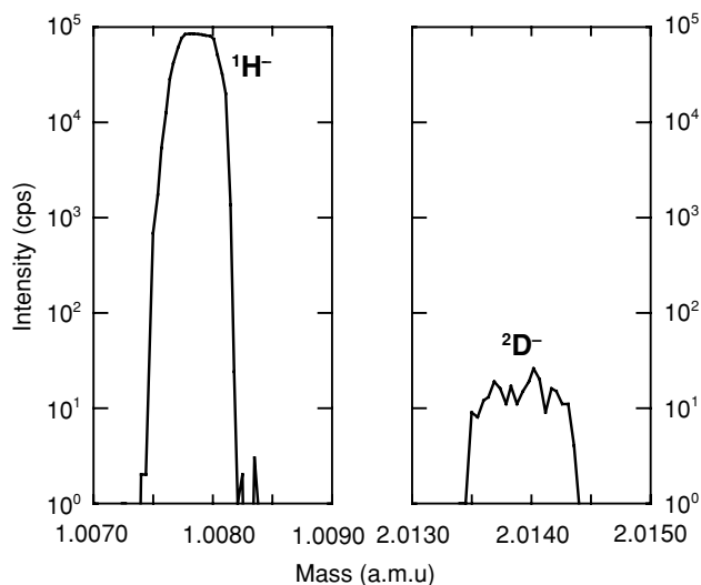
Fig. 5. Representative mass spectra of hydrogen isotopes of a fluid inclusion standard.
