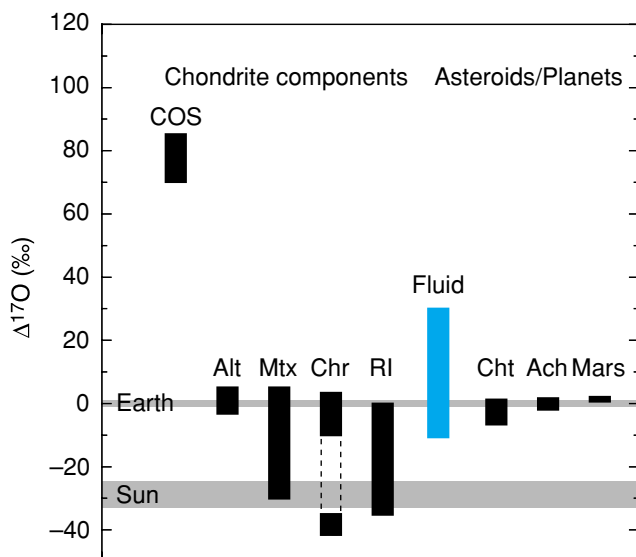
Fig. 14. Distribution of oxygen isotopic compositions observed in the Solar System. Sun (McKeegan et al. , 2011), Earth, Mars, achondrite (Ach), chondrite (Cht) (Clayton, 1993), chondrule (Chr), refractory inclusions (RI), chondrite matrix excluding presolar grains (Mtx), aqueous alteration phases of chondrite (Alt) (Yurimoto et al. , 2008), cosmic symplectite (COS) (Sakamoto et al. , 2007) and fluid inclusion of chondrite (Fluid) (this study).
