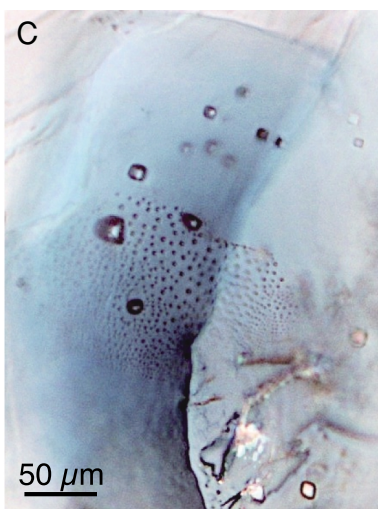
Fig. 1. Representative photographs of fluid inclusions in halite crystals (A) Distributions of fluid inclusions in halite of Monahans (1998). Arrows point to several inclusions. (B) Fluid inclusions in Monahans halite. (C) Fluid inclusions in Zag halite.
