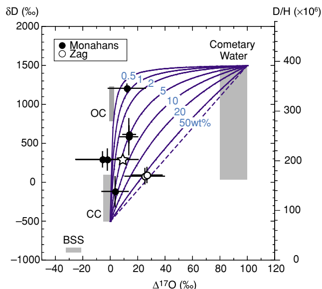
Fig. 15. Relationships of isotopic compositions between hydrogen and oxygen. Open star: average of all measurements shown in Table 1, BSS: bulk solar system, OC: water of ordinary chondrites, CC: water of carbonaceous chondrites, error bars: 2 standard deviations. Water-rock interaction relationships between cometary water and carbonaceous chondrites are shown as blue curves. Water contents of carbonaceous chondrites are parameters and the values are shown on each curve. Isotope fractionation of hydrogen during the interaction is not taken into account because isotopic compositional differences between CC and Cometary water are much larger than the isotopic fractionation factors. Fluid inclusions in Monahans and Zag halite are plotted in the mixing area between CC and Cometary water (reference data from Alexander et al. (2012); Clayton and Mayeda (1999); Clayton et al. (1991); Hartogh et al. (2011); McKeegan et al. (2011); Sakamoto et al. (2007); Yurimoto et al. (2008) and references therein).
