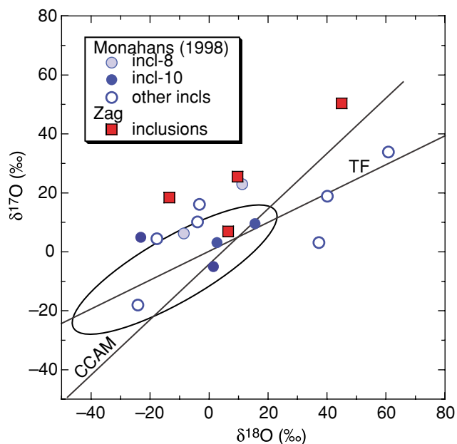
Fig. 11. Three oxygen isotope plots of fluid inclusions in the Monahans and Zag halites. Error ellipse of 95% confidence of standard measurement reproducibility is shown. Duplicate measurements of inclusion #8 and inclusion #10 show that the precision of sample measurements is comparable to the error ellipse. TF: terrestrial fractionation line, CCAM: carbonaceous chondrites anhydrous mineral mixing line.
