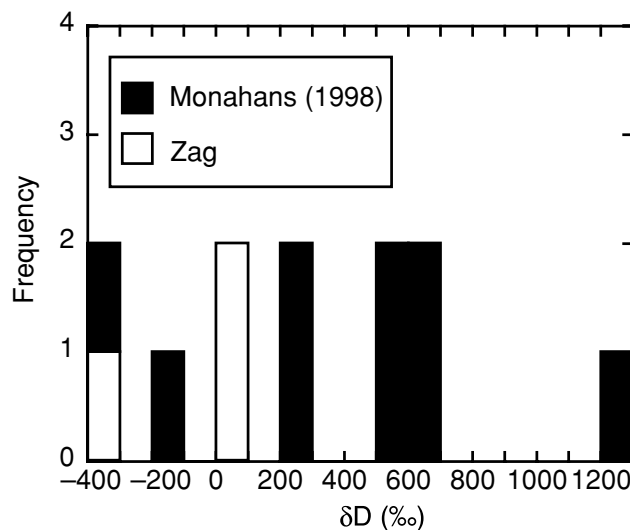
Fig. 9. Variations of hydrogen isotope compositions of fluid inclusions in the Monahans and Zag halite.
