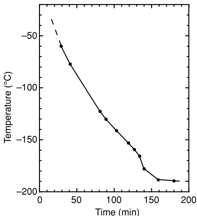
Fig. 4. Cooling temperature curve of cryo-sample-stage as a function of time after supplying liquid nitrogen from room temperature.
