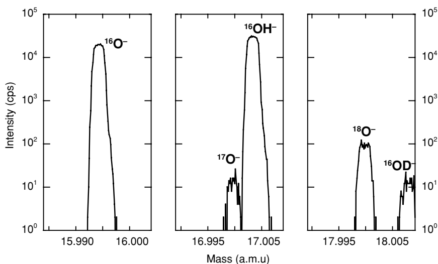
Fig. 6. Representative mass spectra of oxygen isotopes of a fluid inclusion standard.
