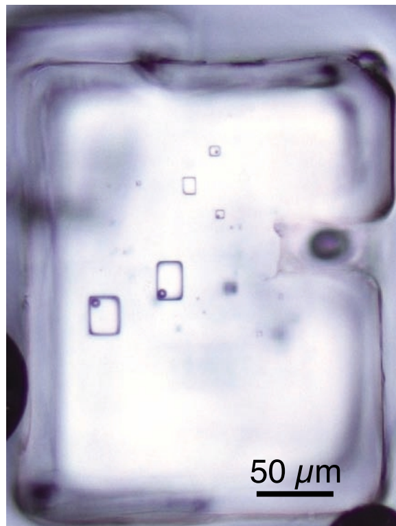
Fig. 2. Photomicrograph of synthetic fluid inclusions in halite.
