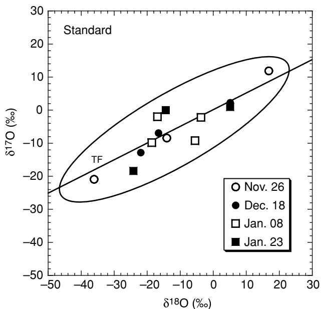
Fig. 10. Reproducibility of oxygen isotope measurements of fluid inclusion standards. Error ellipse indicates 95% confidence. TF: terrestrial fractionation line.
