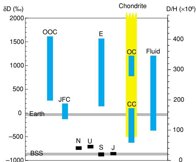
Fig. 13. Distribution of hydrogen isotopic compositions observed in the Solar System. Bulk Solar System (BSS) (Geiss and Gloeckler, 2003; Linsky et al. , 2006), Bulk Earth (Earth) (Lecuyer et al. , 1998), Jupiter (J) (Lellouch et al. , 2001), Saturn (S) (Lellouch et al. , 2001), Uranus (U) (Feuchtgruber et al. , 2013), Neptune (N) (Feuchtgruber et al. , 2013), Enceladus (E) (Waite et al. , 2009), Oort-cloud comets (OOC) (Balsiger et al. , 1995; Biver et al. , 2006; Bockelée-Morvan et al. , 1998, 2012; Hutsemékers et al. , 2008; Meier et al. , 1998; Villanueva et al. , 2009), Jupiter-family comets (JFC) (Hartogh et al. , 2011; Lis et al. , 2013), chondrites (Robert, 2006), estimated compositions of water in carbonaceous (CC) and ordinary (OC) chondrites (Alexander et al. , 2012) and fluid inclusion of chondrite (Fluid) (this study).
