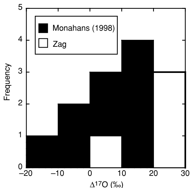
Fig. 12. Variations of mass-independent-fractionation component of oxygen isotope composition of fluid inclusions in the Monahans and Zag halite.
