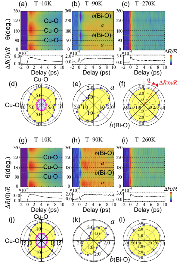
FIG. 2. (Color online) (a)–(c) and (g)–(i) \Delta R(\theta)/R transients at typical temperatures for OD and UD samples, respectively. (d)–(f) and (j)–(l) Polar plots of the maximum values of \Delta R(\theta)/R ( \times 10^4 ). The solid lines indicate fits using Eq. (1). \Delta R(\theta)/\Delta R at delay time of 10 ps is also shown (open circles with dashed fitting line) in (d) and (j). Note that the Cu-O bonds directions are drawn horizontal and vertical, while the crystalline axes are along the Bi-O bonds, and are rotated nearly 45^\circ from the Cu-O bonds.
