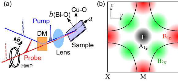
FIG. 1. (Color online) (a) A schematic illustration of the two-color pump-probe setup for polarization-resolved measurements. The probe ( \lambda_{\text{pr}} = 800 nm) was variably polarized by a half-wave plate (HWP) and was combined with the pump ( \lambda_{\text{pu}} = 400 nm) by a dichroic mirror (DM). The angle \theta is measured relative to the Cu-O bond axes. (b) The k -space selectivity of the probe according to the Raman-like process is indicated [15].
