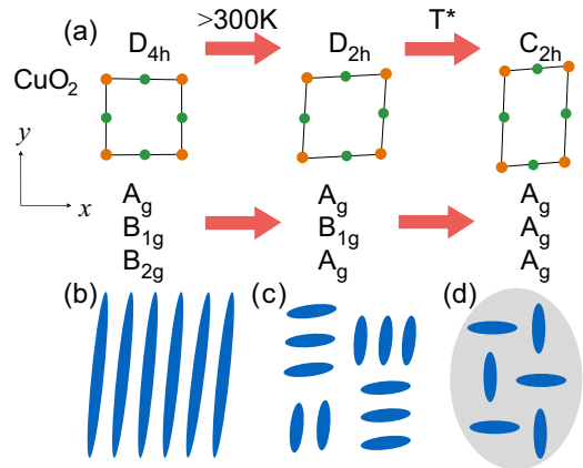
FIG. 5. (Color online) (a) The reduction of symmetries consistent with the observed polarization anisotropy. The \text{CuO}_2 layers are shown. Using the centrosymmetric refinement [39], the highest possible symmetry below T^* is C_{2h} . The relevant irreducible representations are given in each case. (b) Schematic representations corresponding to nematic ordering, (c) short stripe ordering [41–46], and (d) local polaronic order [47].
