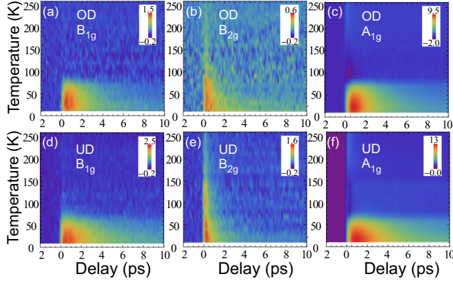
FIG. 3. (Color online) T dependencies of the B_{1g} , B_{2g} , and A_{1g} components of \Delta R corresponding to SC, PG, and metallic state relaxation, respectively, for OD (top) and UD (bottom) samples. The values of the color bars indicate \Delta R/R \times 10^4 .
