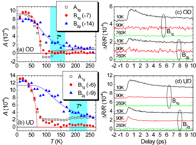
FIG. 4. (Color online) T dependencies of the A_{1g} , B_{1g} , and B_{2g} component amplitudes for UD and OD samples. Note that both B components begin to show an increase of the amplitude below T^* . T^* 's obtained from tunneling [30] are within the region indicated by the shaded area. In the case of the A_{1g} symmetry the PG contribution is superimposed on top of the nearly temperature-independent signal, and has a negative sign. The solid and dashed lines are fits using Mattis-Bardeen [31] and Kabanov [32] models, respectively.
