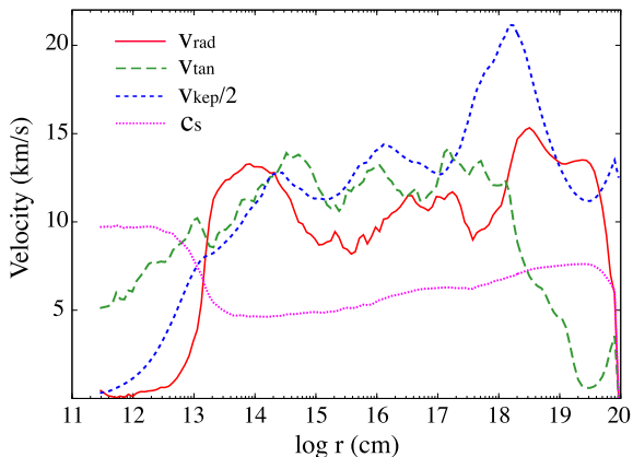
Figure 5. Profiles of the radial (solid) and tangential velocities (long-dashed) at the end of the simulation. For comparison, a half of the Keplerian velocity (short-dashed) and sound speed (dotted) are also shown. All the quantities are spherically averaged.
