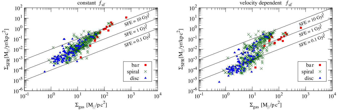
Figure 3. Relation between gas surface density and SFR surface density. The SFR is estimated by the cloud collision model depending on the average collision velocity in 500 \text{ pc} \times 5 \text{ kpc} cylindrical regions. The left-hand panel uses a constant f_{\text{sf}} while the right-hand panel uses the collision velocity-dependent f_{\text{sf}} , as described in Table 2. The coloured markers denote different galactic regions: red squares are clouds in the bar region, green crosses are for the spiral region and blue triangles are those in the disc region. The black solid lines show constant SFEs = 10, 1, 0.1 \text{Gyr}^{-1} .
