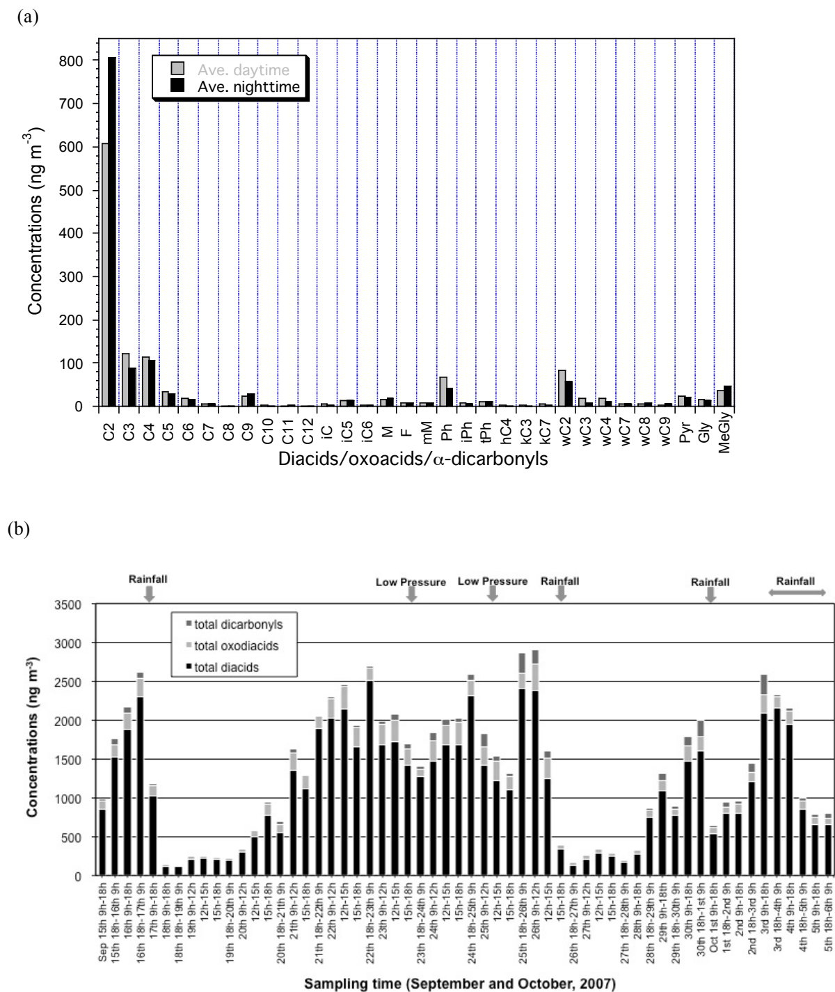
Figure 3. (a) Averaged molecular distributions of dicarboxylic acids, oxocarboxylic acids and \alpha -dicarbonyls in the day and nighttime aerosols from Mangshan. (b) Temporal variations in the concentrations ( \text{ng m}^{-3} ) of water-soluble dicarboxylic acids, oxocarboxylic acids and \alpha -dicarbonyls in the ambient aerosols from Mangshan.
