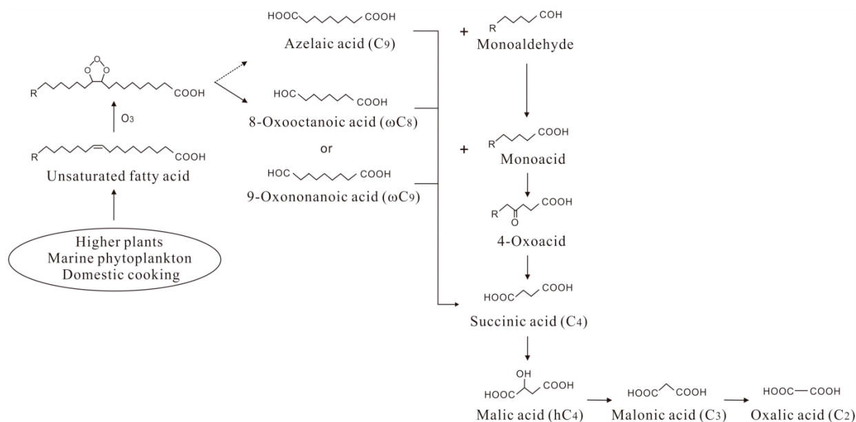
Figure 6. Photochemical formation mechanisms of ωC 8 , ωC 9 and C 9 , as well as C 4 , C 3 and C 2 from biogenic unsaturated fatty acids emitted from higher plants, marine phytoplankton and domestic cooking. Modified from Kawamura et al. (1996a, 1996b) and Kawamura and Sakaguchi (1999).
