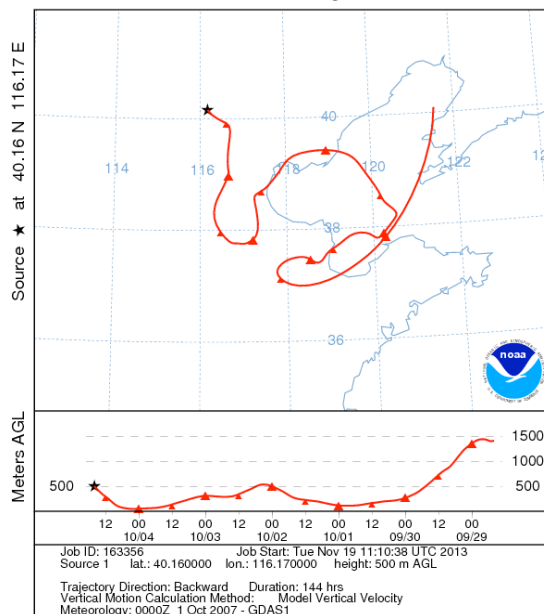
Figure S1. Backward air mass trajectories for the aerosol sample collected during (a) October 3-4 and (b) October 4-5, 2007 (local time is 00h) when higher peaks of diacid-C/TC were obtained (Figure 4). The trajectories were calculated for 6 days using the NOAA Hybrid Single-Particle Lagrangian Integrated Trajectory (Draxler and Ralph, 2013; Rolph 2013).
