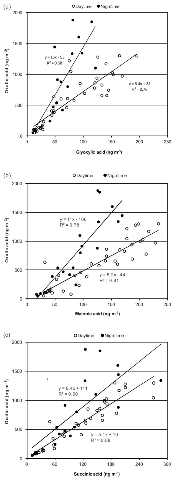
Figure 5. Correlation plots for the concentrations of (a) oxalic acid (C 2 ) and glyoxylic acid (ωC 2 ), (b) oxalic acid (C 2 ) and malonic acid (C 3 ), and (c) oxalic acid (C 2 ) and succinic acid (C 4 ) in Mangshan aerosols for daytime and nighttime.
