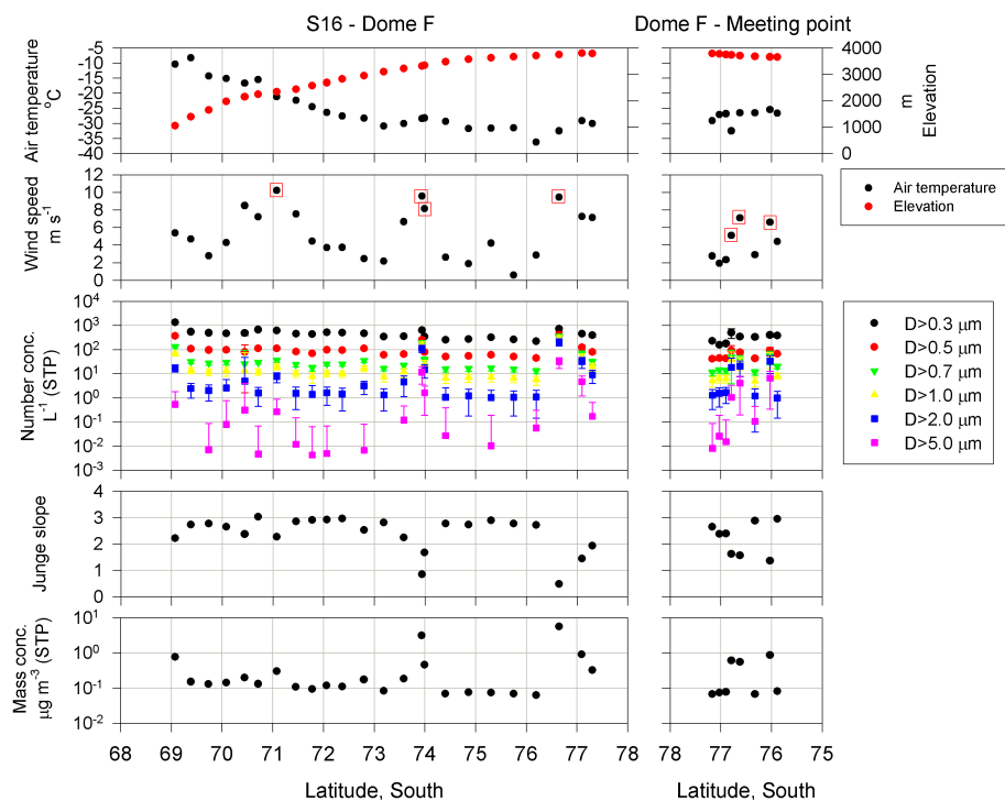
Figure 4. Horizontal features of air temperature, elevation, wind speed, aerosol number concentrations and Junge slope during incoming traverse from S16 to the meeting point. Red boxes show conditions with drifting snow.
