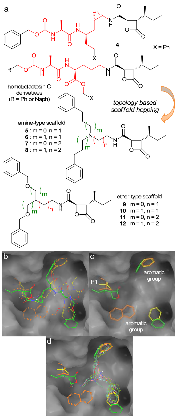
Fig. 2 Rational design of the non-peptidic belactosin A derivatives by topology-based scaffold hopping (a) Structure of the compound 4 , homobelactosin C derivatives 14, 15 and newly designed non-peptide derivatives 5-12 (b) Previously analyzed non-covalent binding mode of 4 (green tube) and X-ray analyzed binding mode of the homobelactosin C derivatives (yellow and
