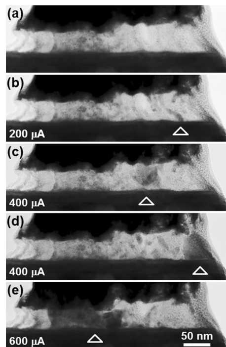
FIG. 5. TEM images of the ReRAM in the (a) initial state and (b)–(e) LRS after the continuous set operations with increasing compliance current as indicated in each figure. Triangles are the filament positions.
