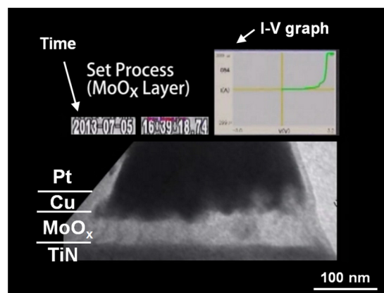
FIG. 2. Video movie of a ReRAM operation cycle with the frames of the I - V graph and time. The left part of the image was darker than the right part. This was caused by imperfection of the experimental condition. The center of the electron beam for the TEM observation was slightly shifted to the upper right. (Multimedia view) [URL: http://dx.doi.org/10.1063/1.4898773.1 ].
