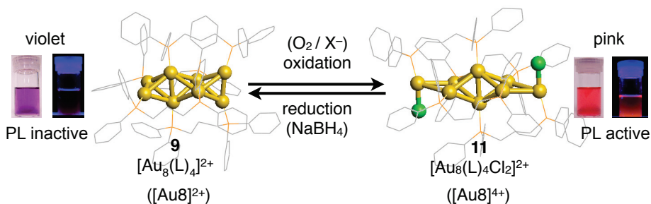
Fig. 11 Redox-mediated chromism between 9 and 11 associated with the isomerization of the \text{Au}_8 cluster framework
