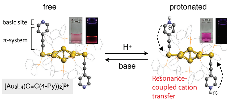
Fig. 12 Protonation-induced chromism of 4-pyridylethynyl-appended \text{Au}_8 cluster
