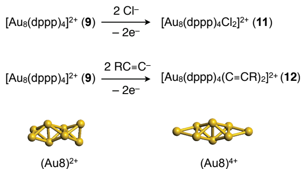
Scheme 8 Nucleophilic addition to [Au 8 (dppp) 4 ] 2+ (9) accompanying the oxidative skeletal isomerization
