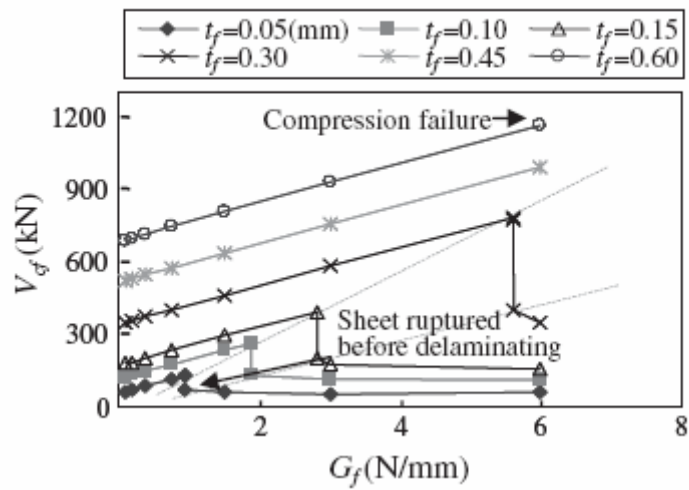
Figure 27 Effects of fracture energy on the shear capacity of strengthened members
