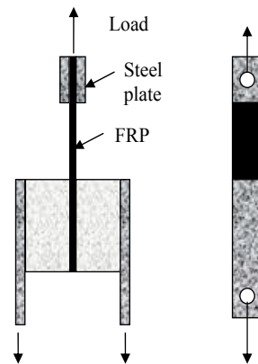
Figure 6 inserted type shear bond test
