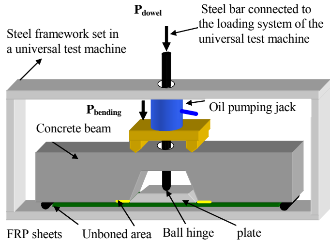
Figure 13 Mix-mode bond tests for FRP sheet-concrete interfaces
