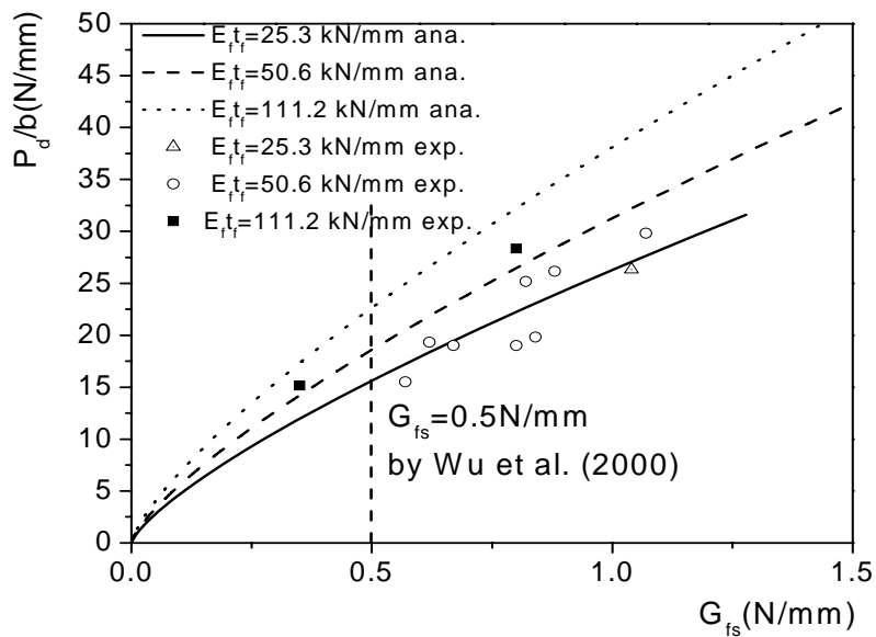
Figure 22 Relationship between dowel force capacity and the interface spalling fracture energy
