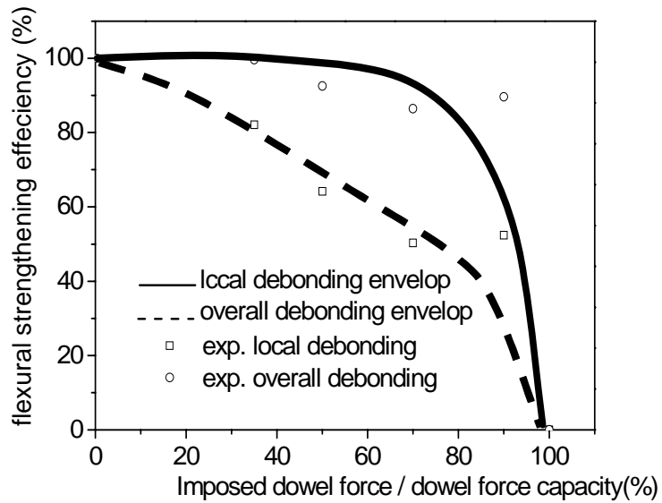
Figure 14 Effects of the dowel force on the shear force transfer on the interface shear stress transfer
