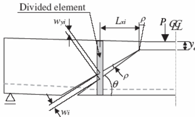
Figure 25 Rigid body model for predicting the shear capacity of FRP strengthened members
