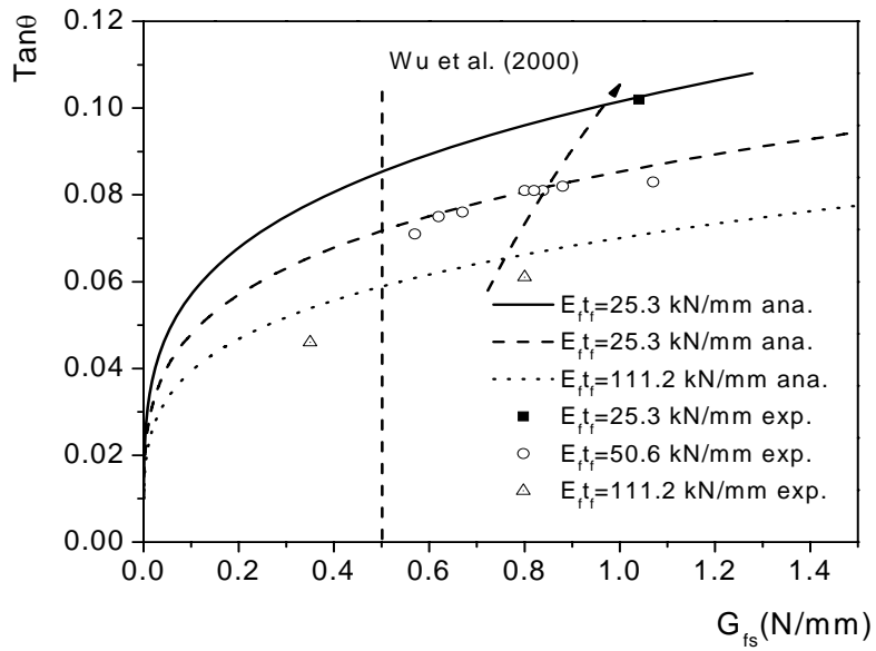
Figure 21 Relationship between peeling angle and the interface spalling fracture energy
