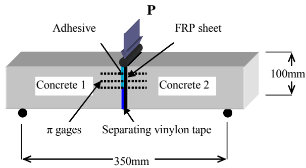
Figure 8 three-point bending test
