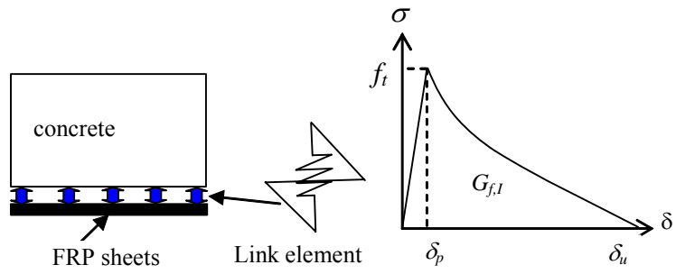
Figure 19 Modeling of the interface bond under tension
