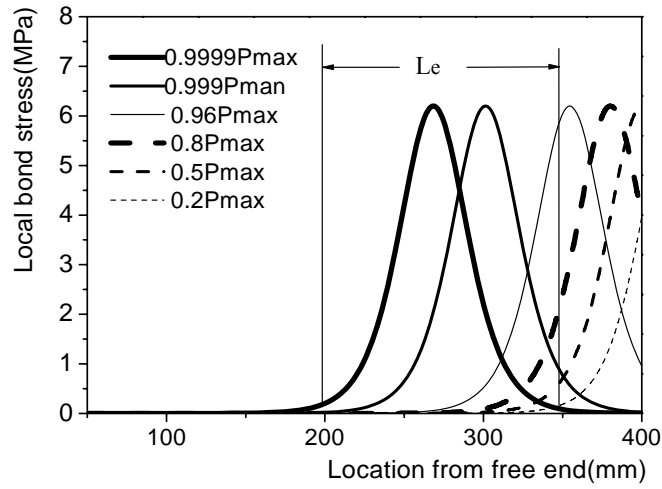
Figure 17 Definition of the effective bond length L_e
