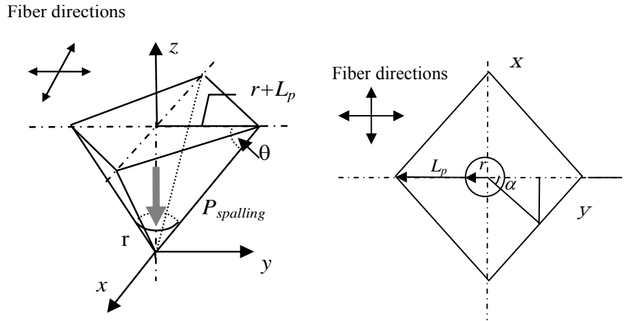
Figure 23 Spalling of FRP sheet-concrete interfaces in two dimensional retrofitting cases
