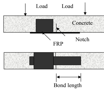
Figure 5 bending-type shear bond test
