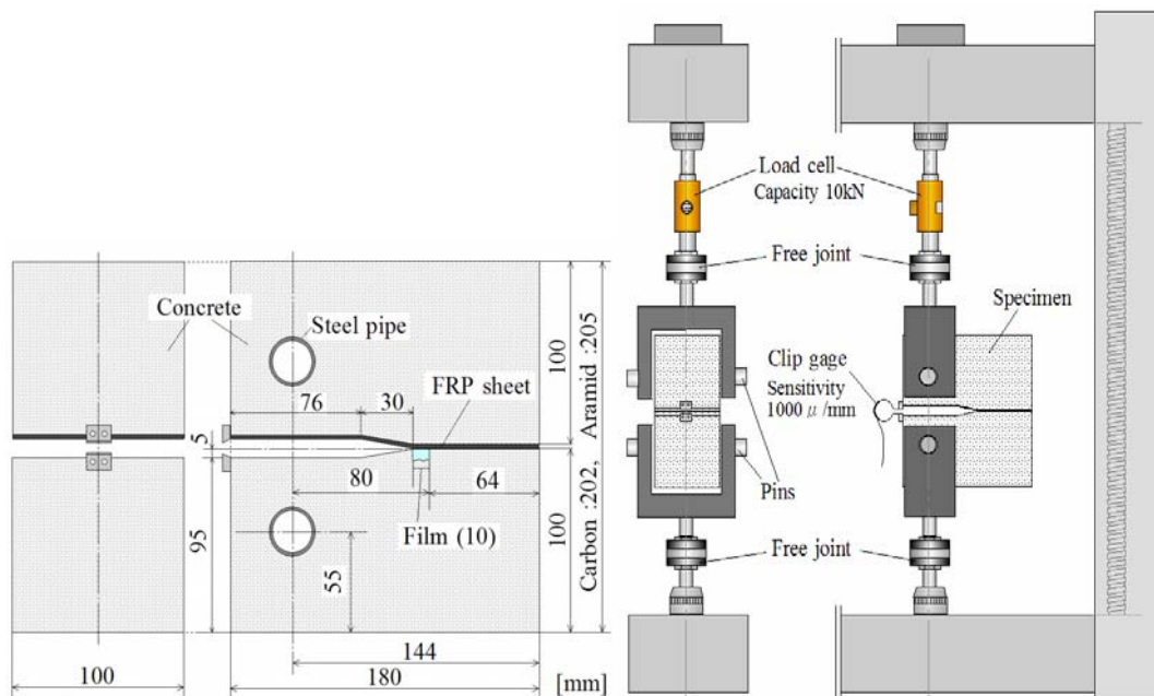
Figure 9 wedging splitting test
