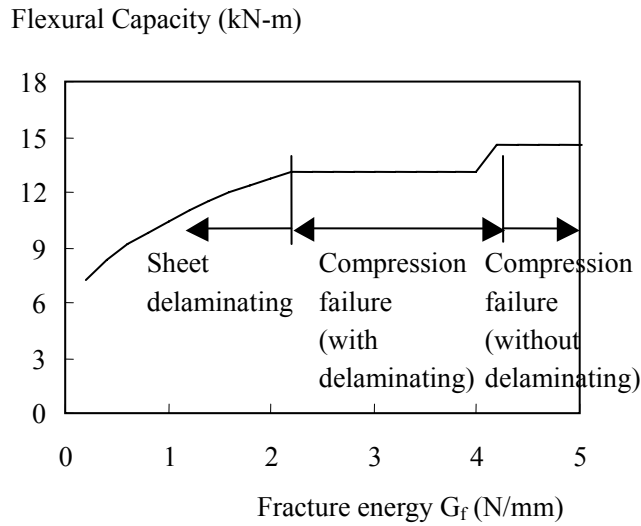
Figure 24 Effects of the interfacial fracture energy in FRP flexurally strengthened members
