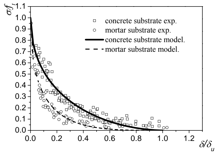
Figure 20 Tension softening diagrams of FRP sheet-concrete interfaces
