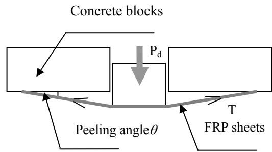
Figure 10 Dowel test for FRP sheet-concrete interfaces
