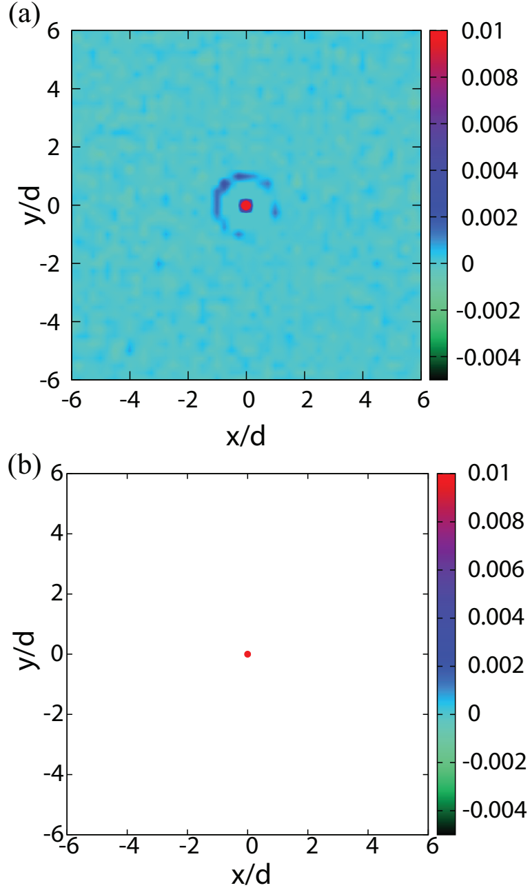
FIGURE C.1: (a) The time averaged spatial correlation of \bar{\psi}_6 . (b) the time averaged spatial correlation of \bar{\psi}_6 larger than the standard error in correlation showing that the time averaged spatial correlation of \bar{\psi}_6 does not have a significant statistical correlation except the center particle. The color grade indicates the strength of correlation.
