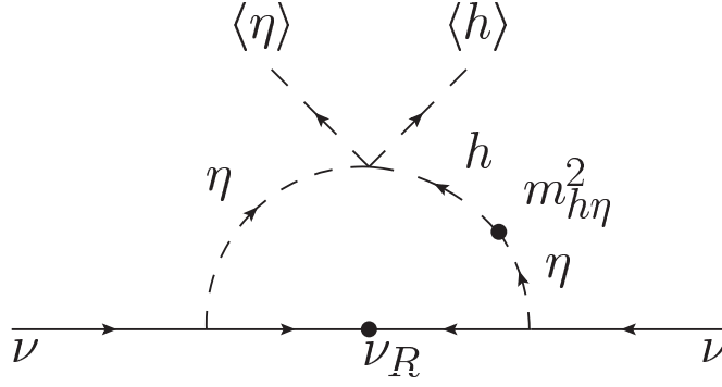
Figure 2. The one-loop diagrams contributing to A_4 breaking neutrino masses under mass insertion approximations for m_{h\eta}^2/m_\eta^2 .
