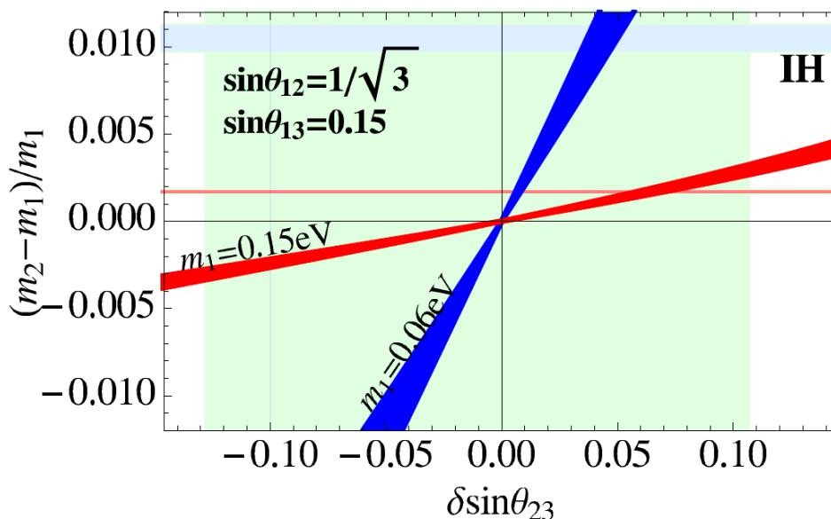
Figure 5. \delta s_{23} and \delta m_{12}/m_1 in the IH case with s_{23} > 0 , s_{12} = 1/\sqrt{3} and s_{13} = 0.15 . The red (blue) line is the prediction of our A_4 model with m_1 = 0.15(0.06)\text{eV} , within 3\sigma of |\Delta m^2| . The light green region for the 3\sigma allowed range of \sin^2 \theta_{23} , and the light pink (blue) band for the one of \Delta m_{12}^2 with m_1 = 0.15(0.06)\text{eV} respectively.
