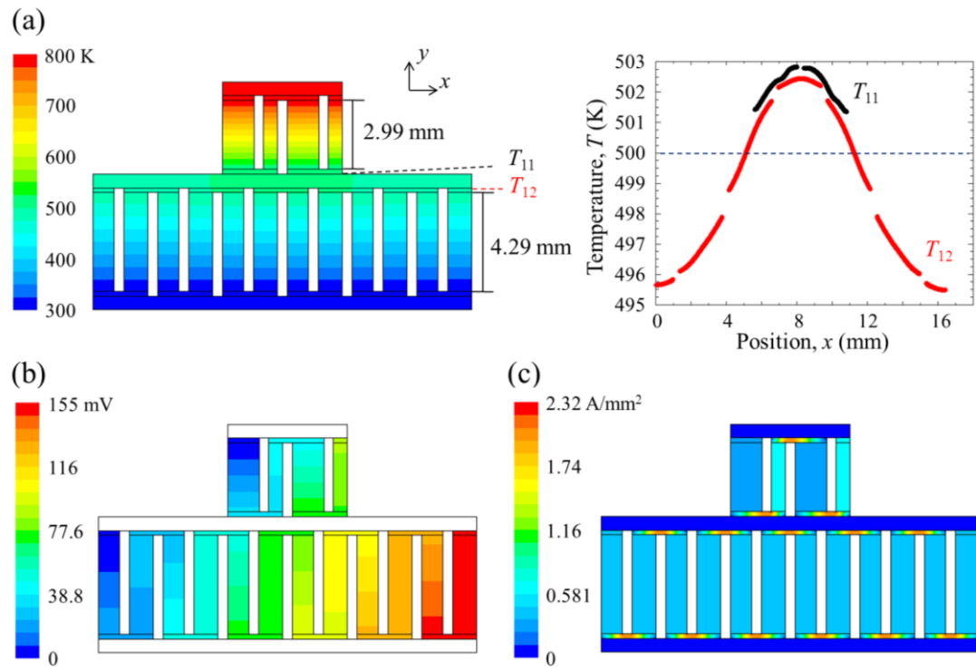
Fig. 8 (a) Temperature profile, (b) electric potential profile, and (c) current density profile of Module C
