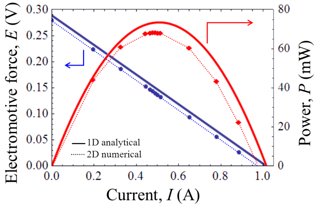
Fig. 4 Voltage-current and power-current characteristics of Module A calculated using a one-dimensional analytical model (1D) and numerical model (2D)
