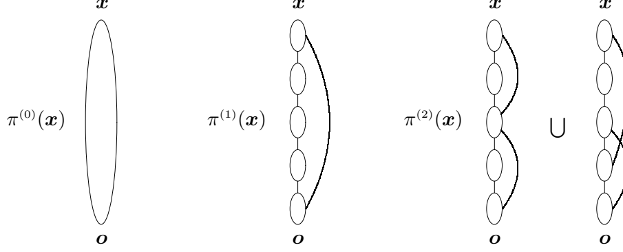
Figure 4: Schematic representations of \pi^{(0)}(\mathbf{x}) , \pi^{(1)}(\mathbf{x}) and \pi^{(2)}(\mathbf{x}) .
