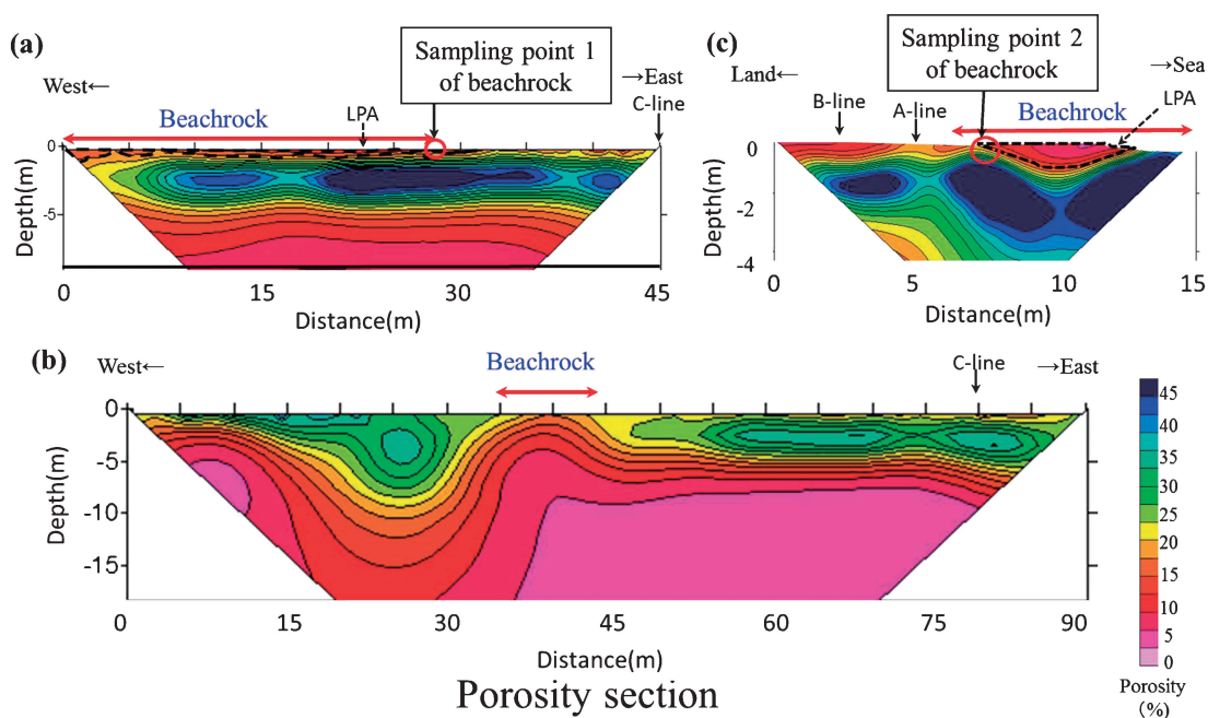
Fig. 10 Porosity sections. (a) Porosity section of A-line, (b) Porosity section of B-line, (c) Porosity section of C-line. LPA: low porosity area.
