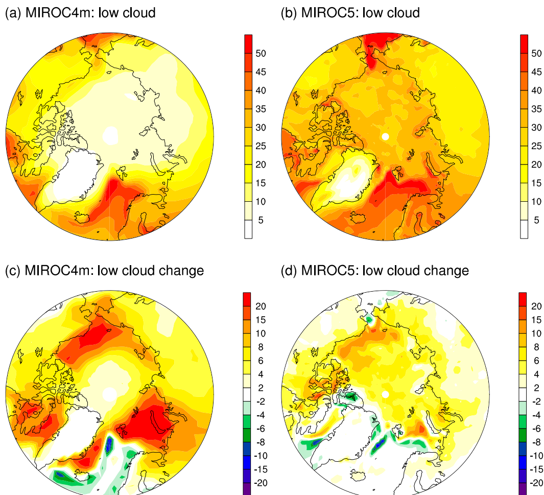
FIG. 7. Low-level cloud amount in OND (%) for (a) MIROC4m control, (b) MIROC5 control, (c) MIROC4m 2 \times \text{CO}_2 change, and (d) MIROC5 2 \times \text{CO}_2 change.
