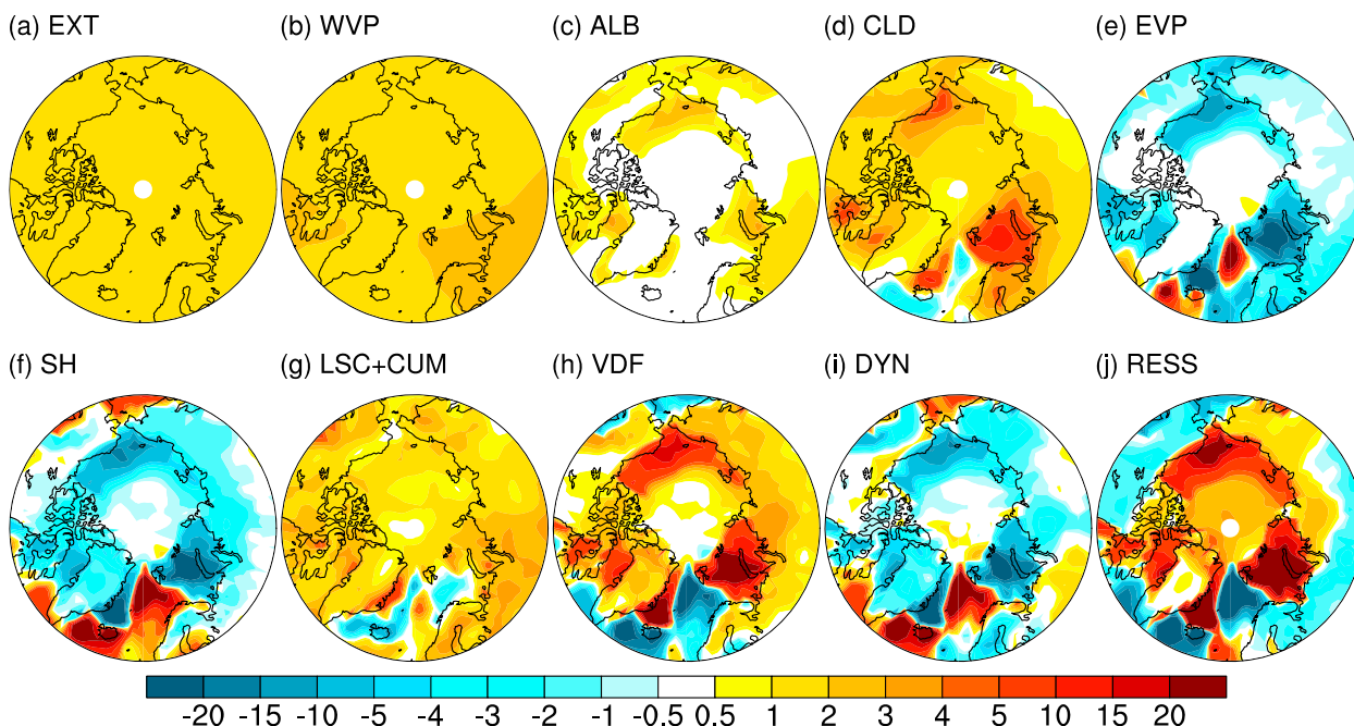
FIG. 5. OND partial surface (skin) temperature changes (°C) in MIROC4m ( >60^{\circ}\text{N} ) from (a) 2 \times \text{CO}_2 , (b) water vapor, (c) surface albedo, (d) clouds, (e) surface evaporation, (f) surface sensible heat flux, (g) large-scale condensation and cumulus convection, (h) vertical diffusion, (i) dynamical heating, and (j) net surface energy flux. Partial temperature changes due to dry adjustments and atmospheric heat storage are small and not shown.
