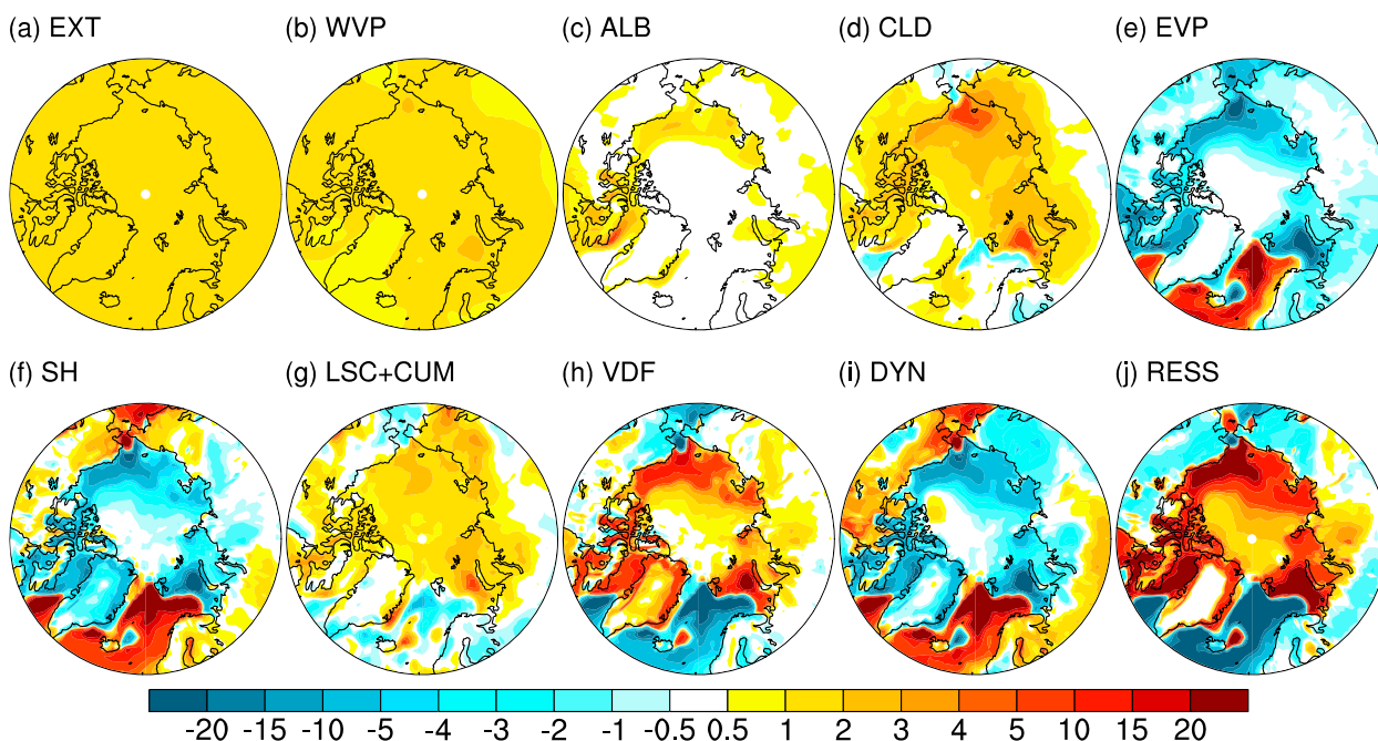
FIG. 6. As in Fig. 5, but for MIROC5. Partial surface temperature change due to atmospheric heat storage is small and not shown.
