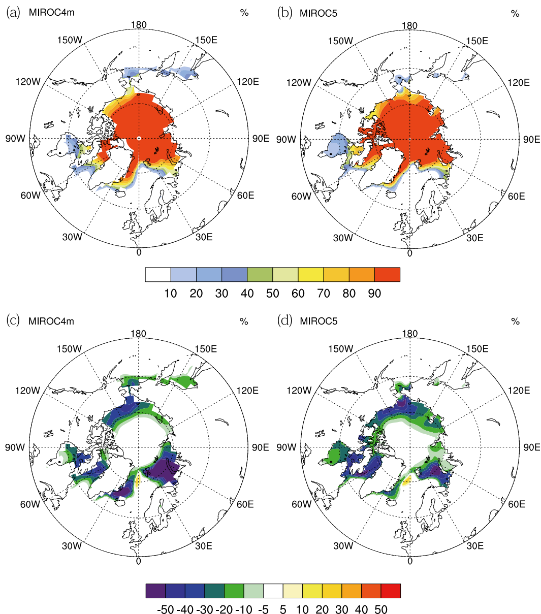
FIG. 4. Sea ice concentration (%) averaged over OND for (a) MIROC4m control, (b) MIROC5 control, (c) MIROC4m 2 \times \text{CO}_2 change, and (d) MIROC5 2 \times \text{CO}_2 change.
