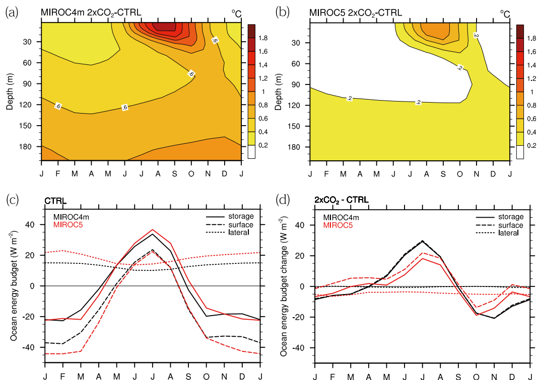
FIG. 9. Seasonal changes in the Arctic Ocean ( >70^{\circ}\text{N} ) for the top 200-m ocean potential temperature change in (a) MIROC4m and (b) MIROC5. (c) Energy budget and (d) energy budget changes over the full ocean depth from the control simulations. In (c) and (d), positive values indicate net energy gain for the Arctic Ocean.
