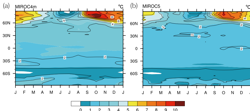
FIG. 2. Changes in zonal mean surface (skin) temperature ( ^{\circ}\text{C} ) from the control simulations for (a) MIROC4m and (b) MIROC5. Color shadings represent simulated temperature change, and line contours represent sum of individual partial temperature changes diagnosed using the CFRAM technique.
