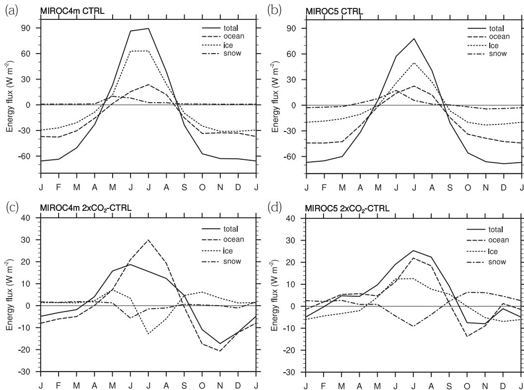
FIG. 8. Seasonal energy exchange in the Arctic Ocean ( >70^{\circ}\text{N} ) for (a) MIROC4m control, (b) MIROC5 control, (c) MIROC4m 2 \times \text{CO}_2 change, and (d) MIROC5 2 \times \text{CO}_2 change. Total (solid lines) is RESS, ocean (dashed lines) is energy flux into the ocean, ice (dotted lines) is latent heat consumed and released with sea ice melting and growth, and snow (dashed-dotted lines) is latent heat consumed for snow melting. Note that the interpolation from atmospheric to ocean grids introduces a small error into the estimate of snow [which must be positive in (a) and (b)].
