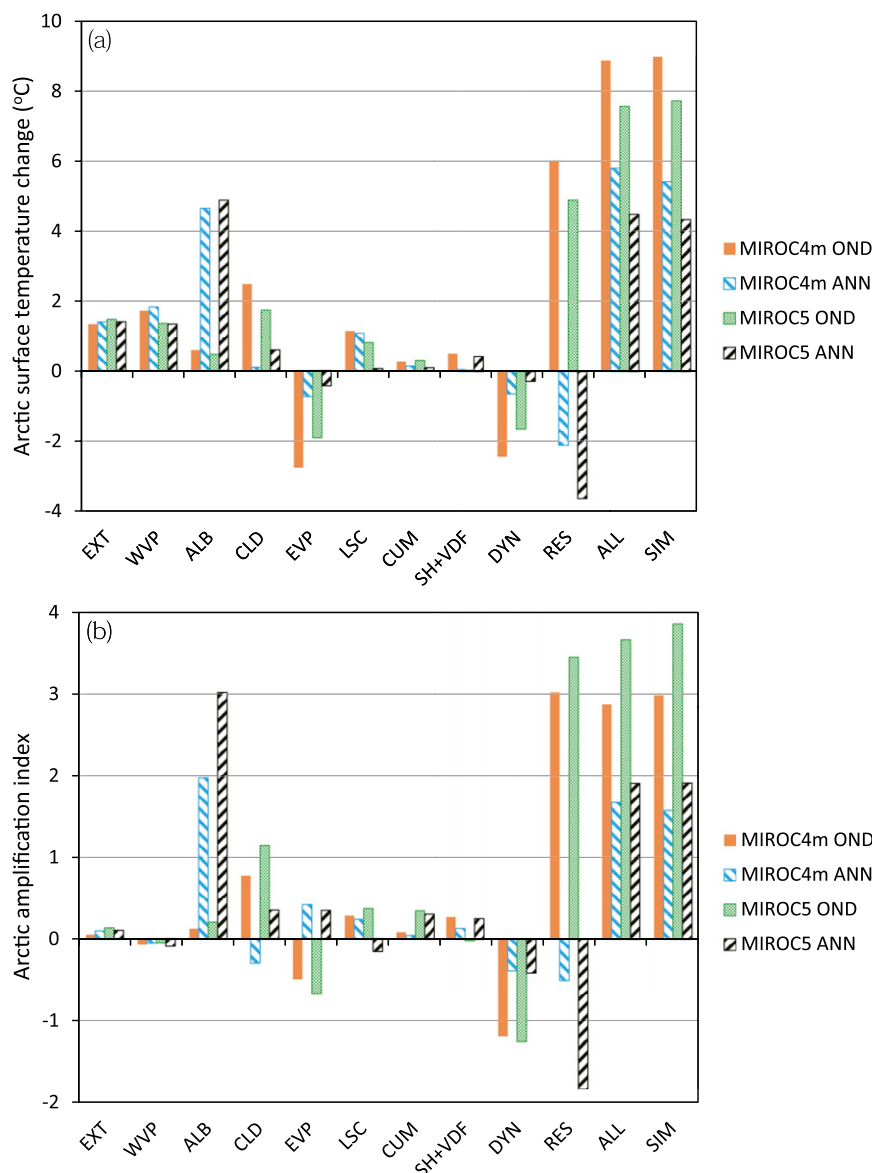
FIG. 11. Partial surface temperature changes diagnosed using the CFRAM technique (EXT–RES), their sum (ALL), and simulated temperature changes (SIM) with (a) Arctic average temperature and (b) AAI. See text for the definition of the AAI. Abbreviations on the bottom are defined in Table 2. The OND and annual (ANN) means for MIROC4m and MIROC5 are shown.
