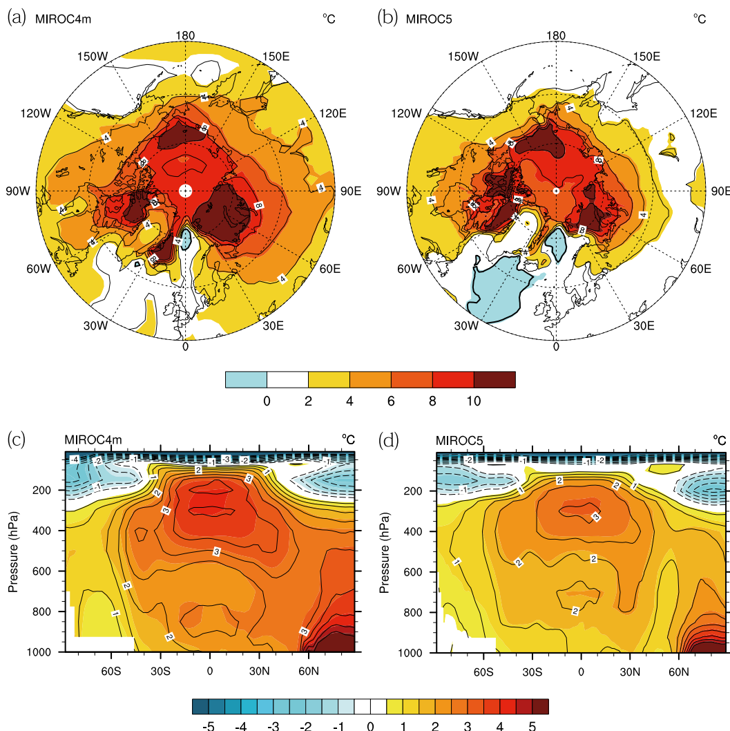
FIG. 3. Temperature changes ( ^{\circ}\text{C} ) from the control simulations averaged over OND (a),(b) at the surface and (c),(d) in the zonally averaged atmosphere, for (left) MIROC4m and (right) MIROC5. Color shadings represent simulated temperature change, and line contours represent sum of individual partial temperature changes diagnosed using the CFRAM technique.
