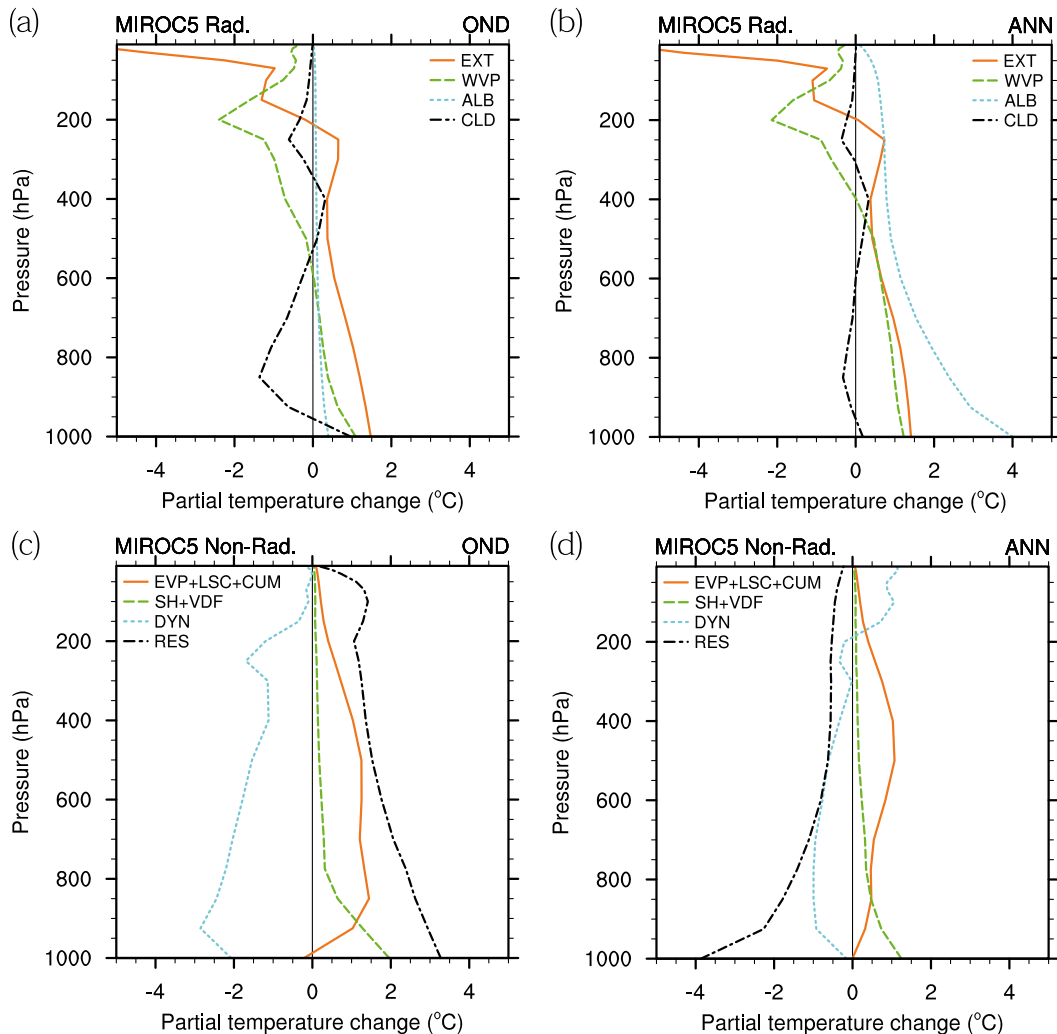
FIG. 10. Vertical profiles of atmospheric partial temperature changes in the Arctic ( >70^{\circ}\text{N} ) diagnosed using the CFRAM technique for MIROC5 (a) OND and (b) annual mean radiative terms, and (c) OND and (d) annual mean nonradiative terms.
