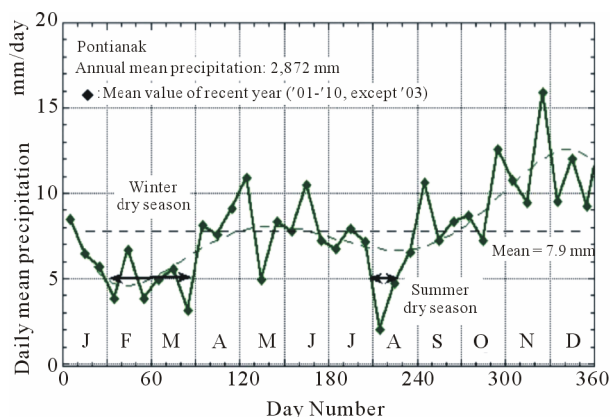
Figure 3. Daily mean precipitation patterns using 9-year data in Pontianak, West Kalimantan.
