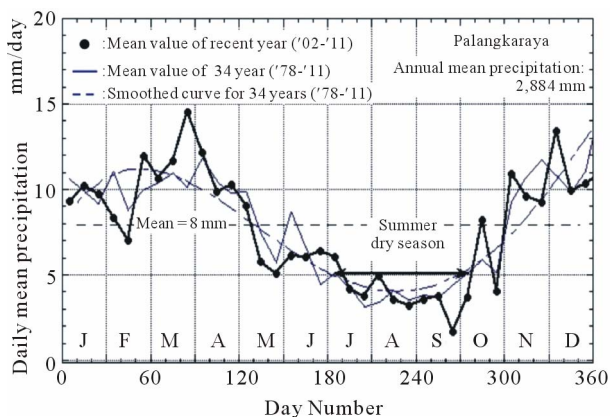
Figure 2. Daily mean precipitation patterns using 10- and 34-year data from Palangkaraya, Central Kalimantan.
