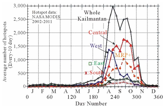
Figure 6. Seasonal (every 10 days) fire occurrence tendencies in Kalimantan.
