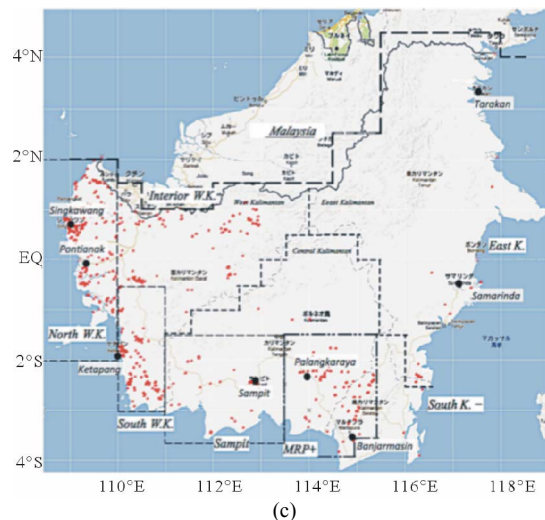
Figure 8. Three typical fire distributions in Kalimantan. (a) Typical severe fire distribution in mid October (2006); (b) Typical West Kalimantan fire distribution in early August (2009); (c) Typical pre-dry season (caution) fire distribution in late July (2009).
