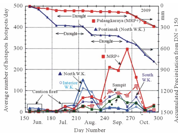
Figure 7. Seasonal fire occurrence and accumulated precipitation from June in 2009.
