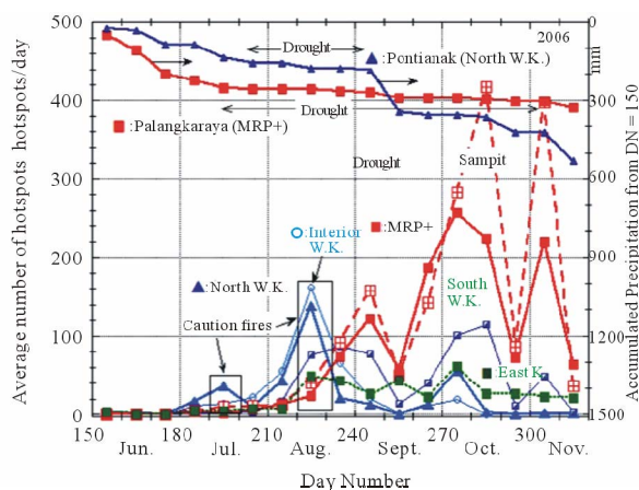
Figure 9. Seasonal fire occurrence and accumulated precipitation from June in 2006.
